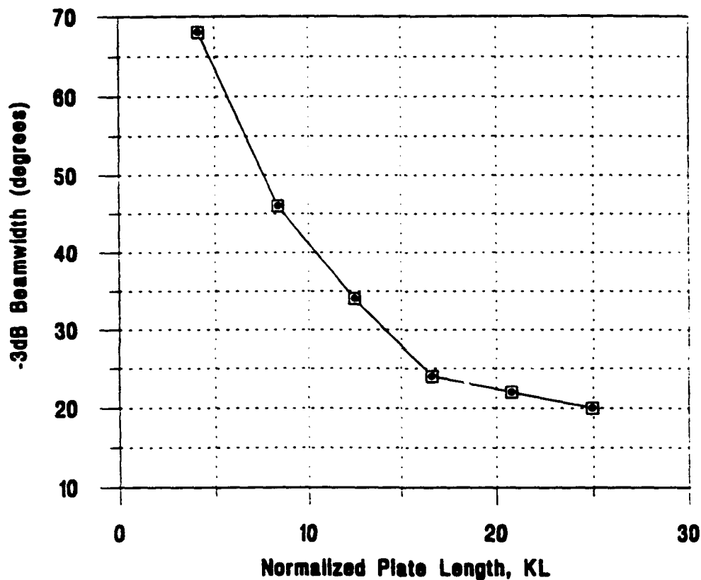
Figure 11. -3dB Beam Width Values for Finite Ribbed Plates at 407Hz .
