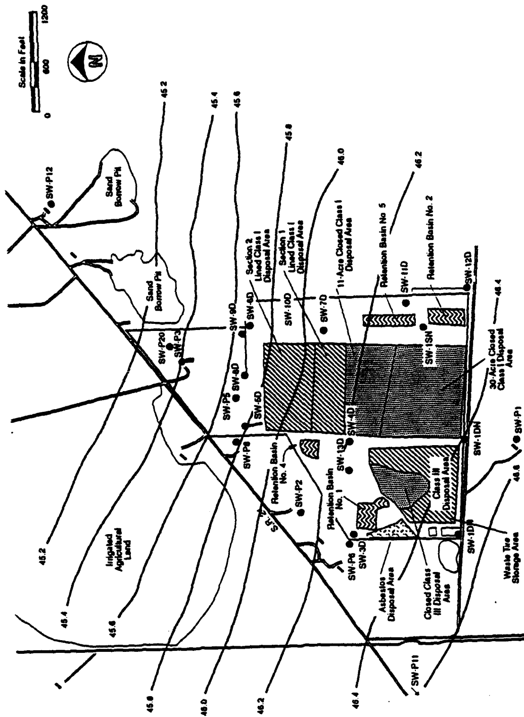
Figure 3-2. Potentiometric Surface at ACSWL, Floridan Aquifer, January 1991 (source: CH2M-Hill, 1992a)
