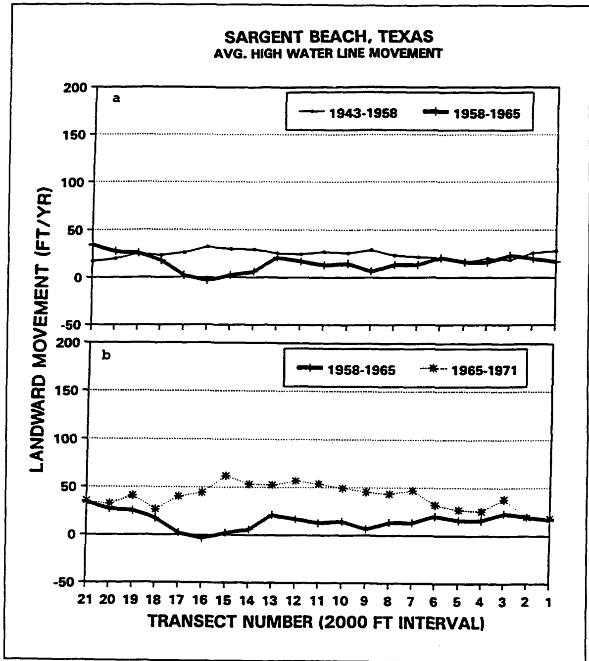
Figure 18. Average high-water line movement (a) from 1943-1958 and 1958-1965, (b) from 1958-1965 and 1965-1971
