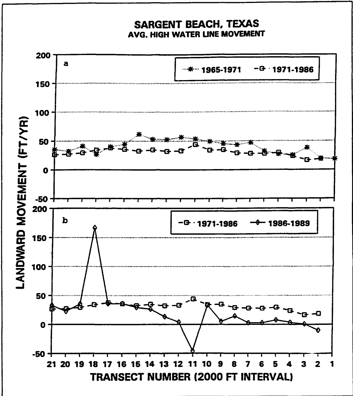
Figure 19. Average high-water line movement (a) from 1965-1971 and 1971-1986, (b) from 1971-1986 and 1986-1989
