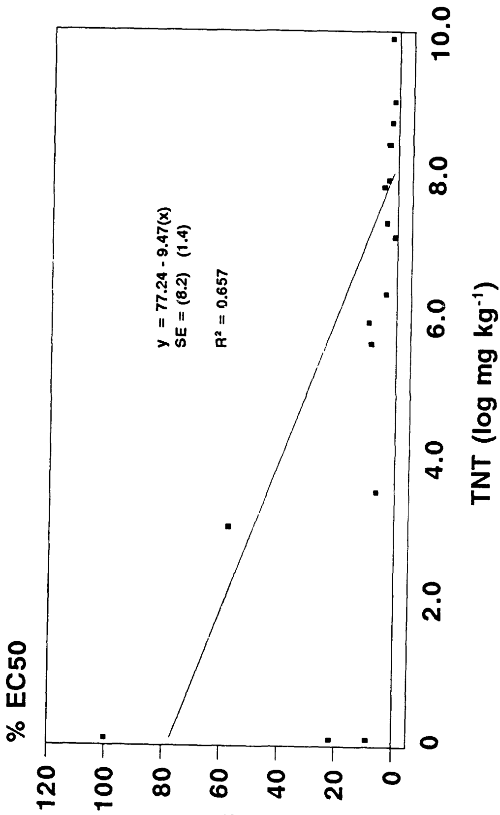
Figure 14. Area L2 - Microtox Percent EC 50 vs TNT
