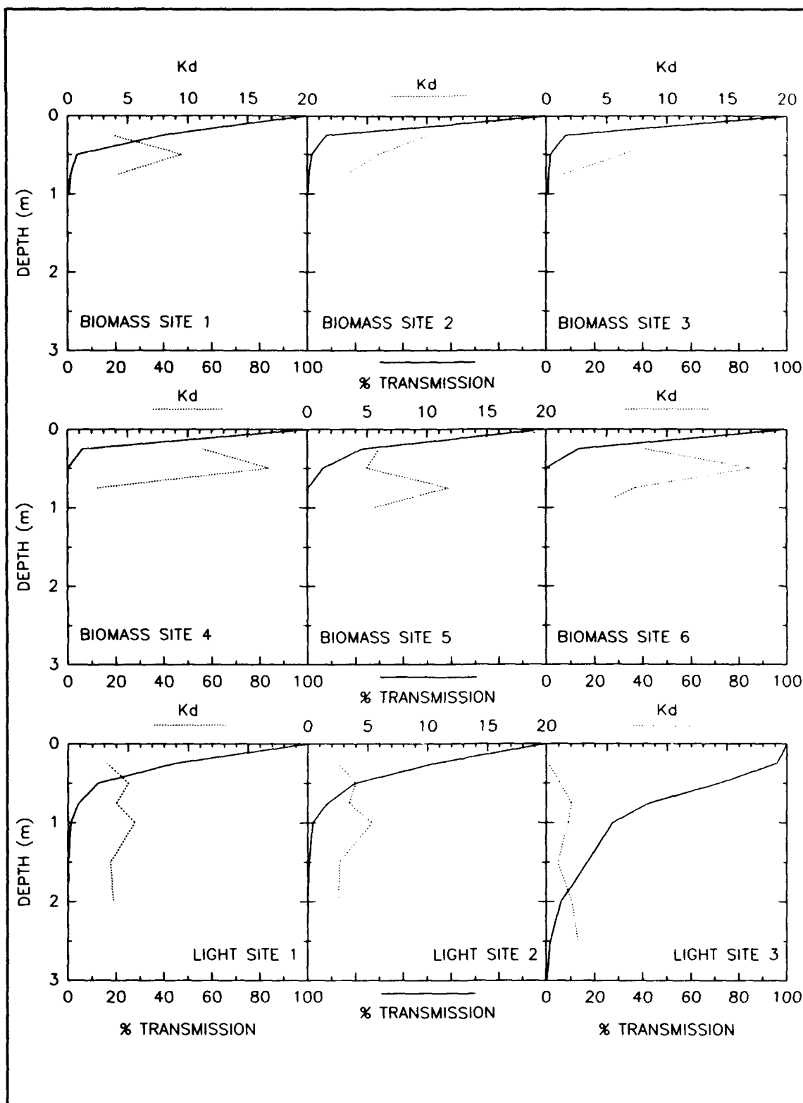
Figure 7. Light profiles for six vegetated sites (I - VI) and three unvegetated sites (L1 - L3) for Kirk Pond. Solid line, percent light transmission; dotted line, light extinction coefficient ( K_d )
