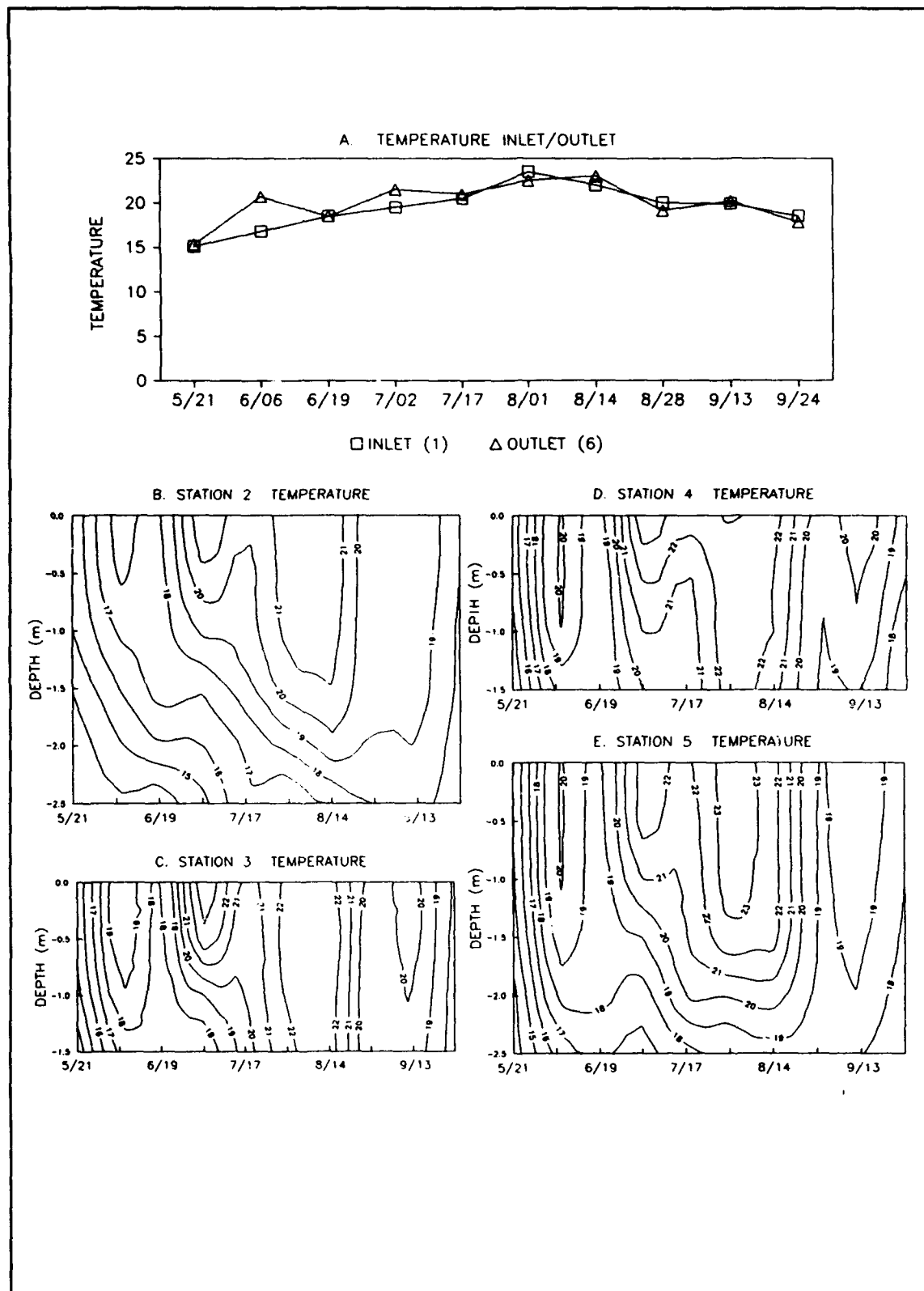
Figure 8. Water temperature ( ^{\circ}\text{C} ) in Kirk Pond at the inflow and outflow, stations 1 and 6, respectively (A), and temperature isopleths for stations 2 through 5 (B through E)
