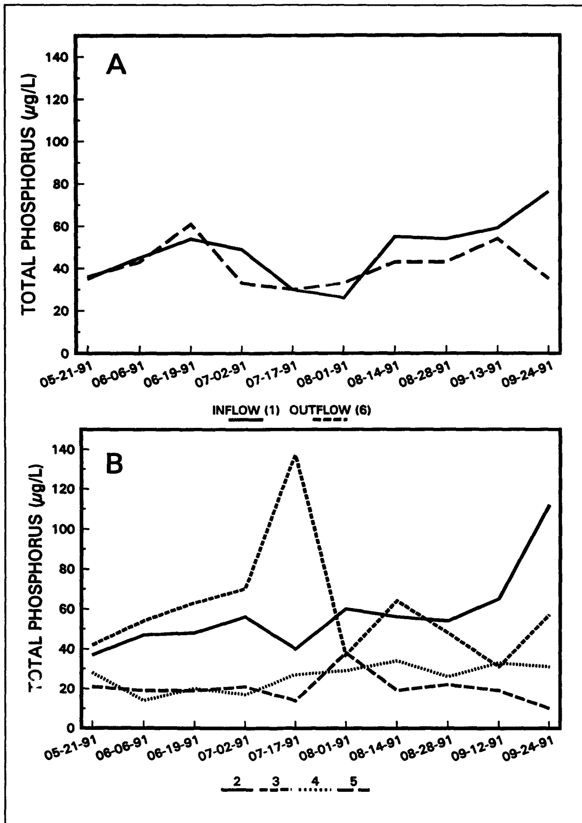
Figure 13. Total phosphorus ( \mu\text{g L}^{-1} ) in Kirk Pond at the inflow and outflow stations (A; 1 and 6, respectively) and at sites 2 through 5 (B)
