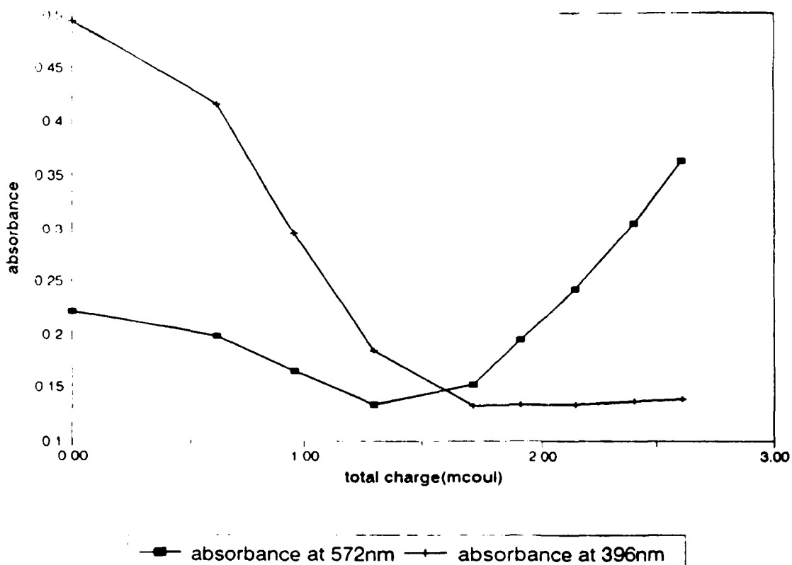
Figure 6 Oxidation of "Blank" 8/12/93
