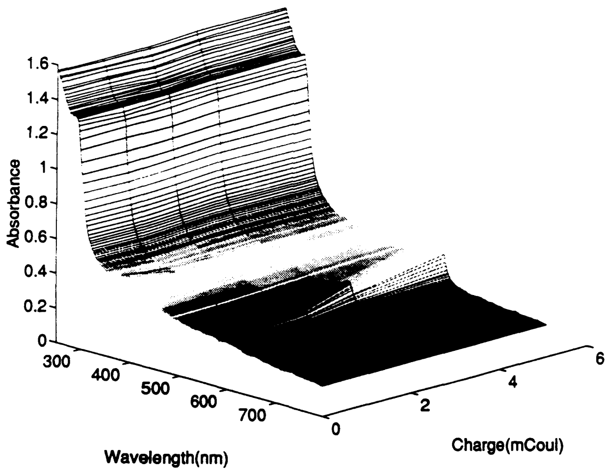
Figure 12 Oxidation of Sediment
