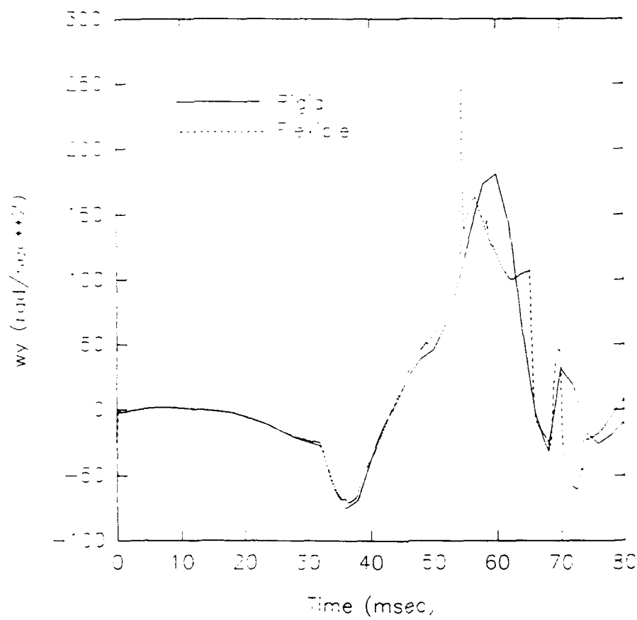
Figure 6. Right Lower Leg Angular Acceleration about Y-Axis
