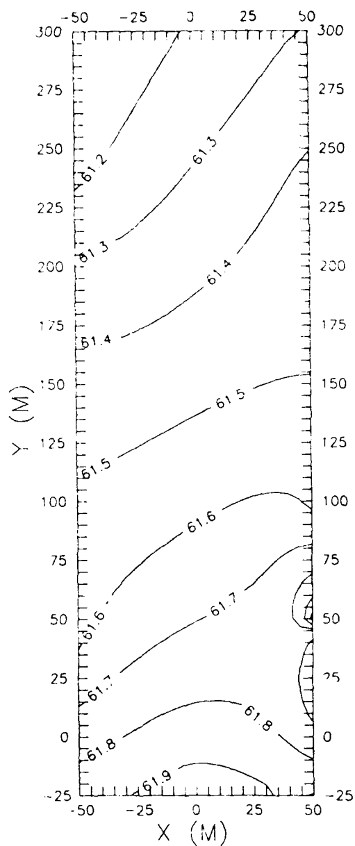
Figure 5. Predicted water table contours in meters on simulation day 42. Left: uniform hydraulic conductivity model. Right: variable hydraulic conductivity model.
