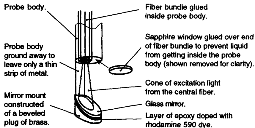
Figure 1. Construction of the Fiber-Optic Probe.
