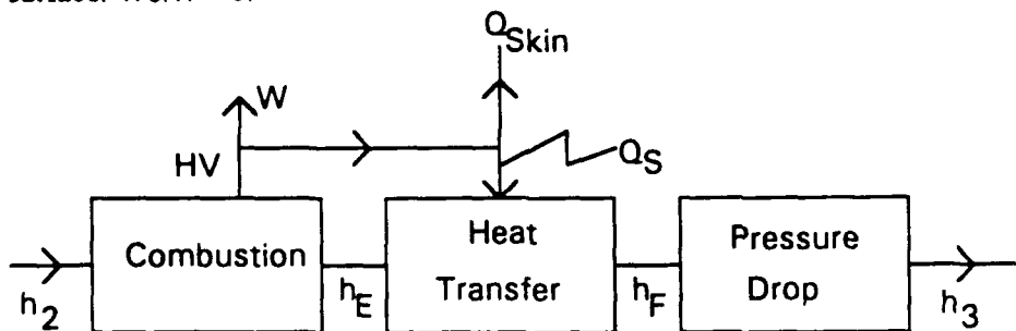
FIGURE 4 Systemic Block Diagram
