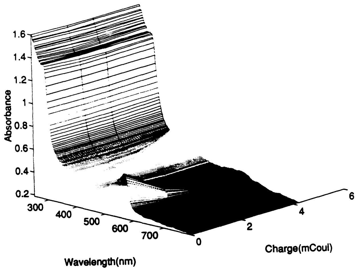
Figure 13 Second Reduction of Sediment
