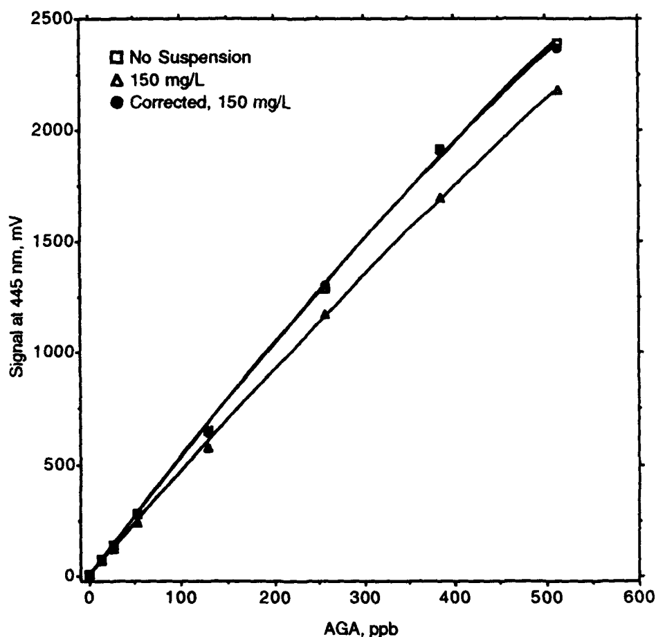
Figure 7. Correction of AGA Fluorescence Data for Turbidity.
