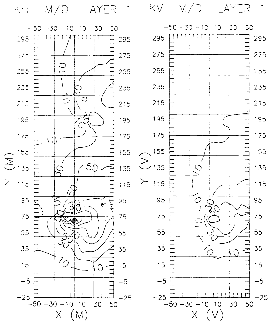
Figure 4. Horizontal (left) and vertical (right) hydraulic conductivity in m/day for the top layer of the variable conductivity model.
