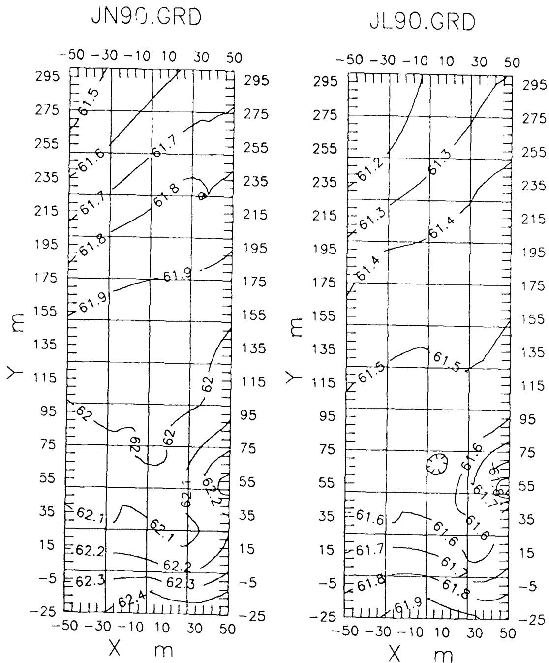
Figure 3. Krigged water table contours in meters for the first two piezometer surveys. Left: simulation day 8 (June 19). Right: simulation day 42 (July 23).
