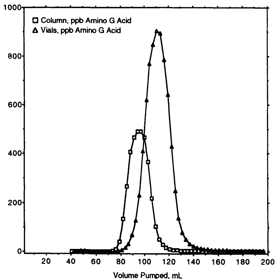
Figure 3. Breakthrough of AGA on Sand (1 mL/min Pump Rate).
