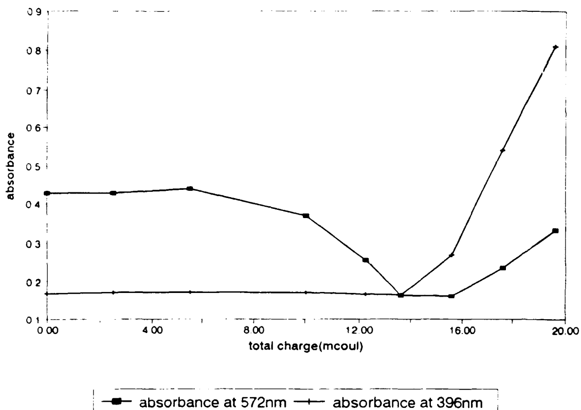
Figure 5 Reduction of "Blank" 8/12/93
