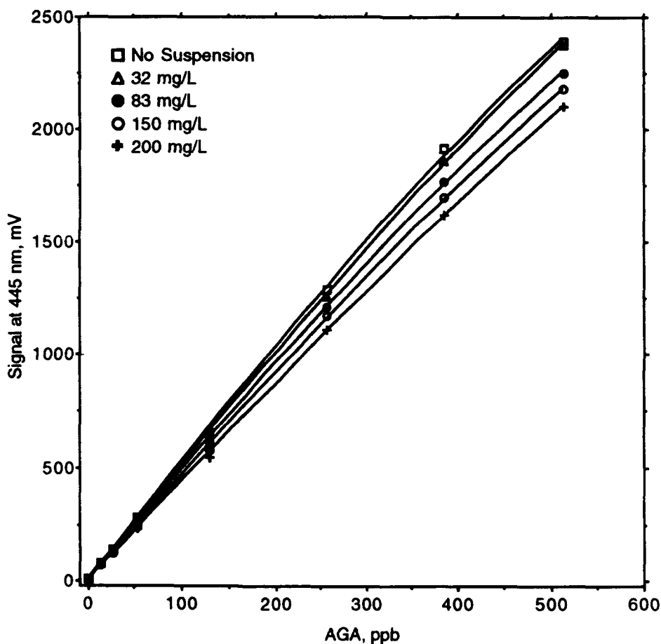
Figure 6. Affect of Turbidity on AGA Fluorescence.
