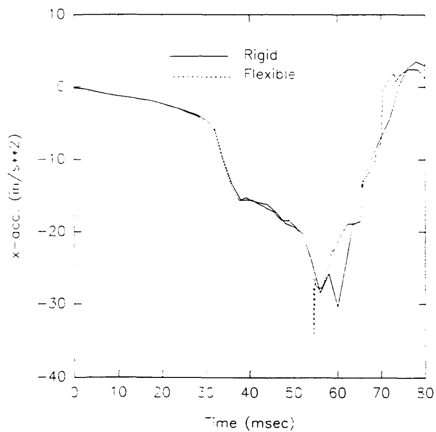
Figure 5. Right Lower Leg Acceleration Relative to the Vehicle in X-Direction
