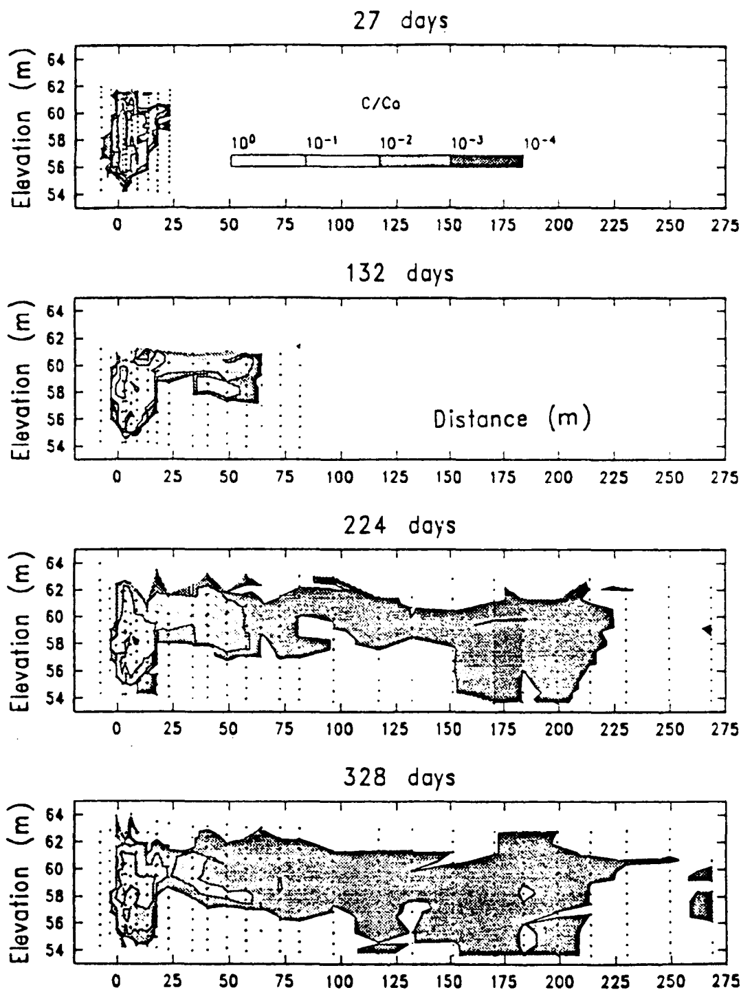
Figure 2. Tritium relative activity profiles along the plume axis during MADE-2. Times are days after start of injection: 27 days after injection = simulation day 42, etc. Source: Boggs and others, 1993.
