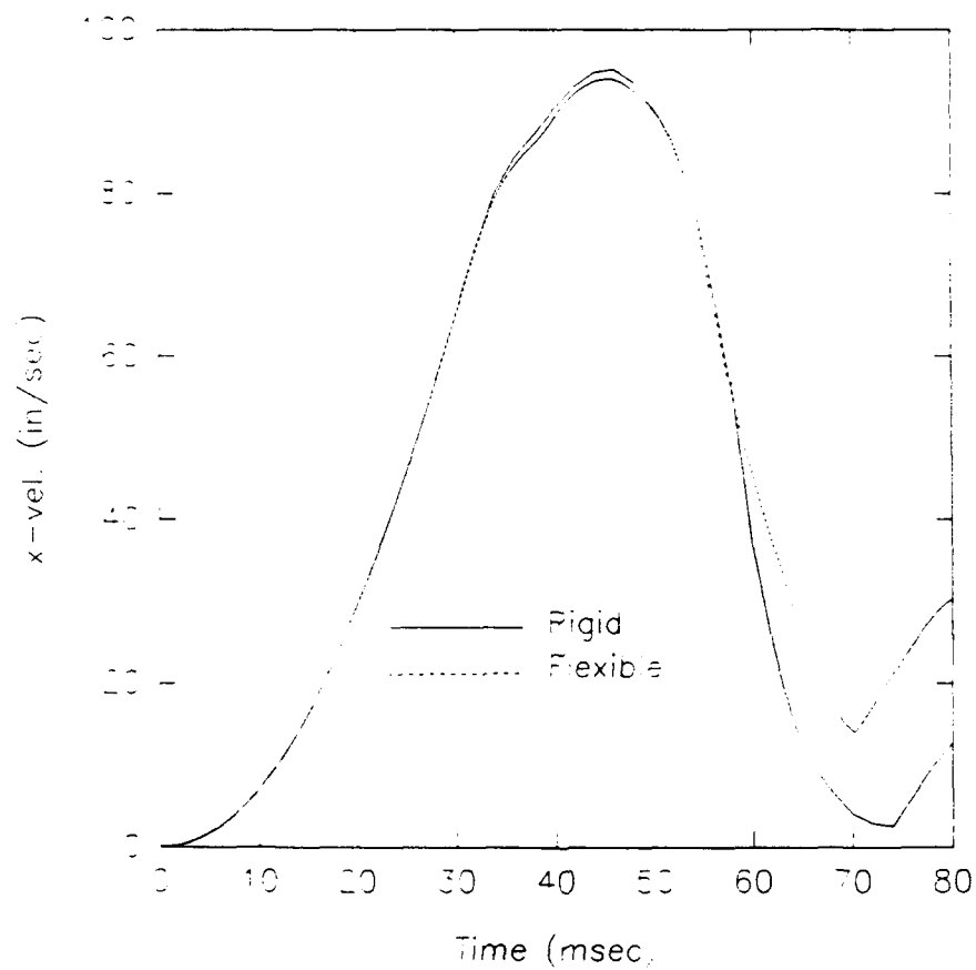
Figure 4. Right Lower Leg Velocity Relative to the Vehicle in X-Direction
