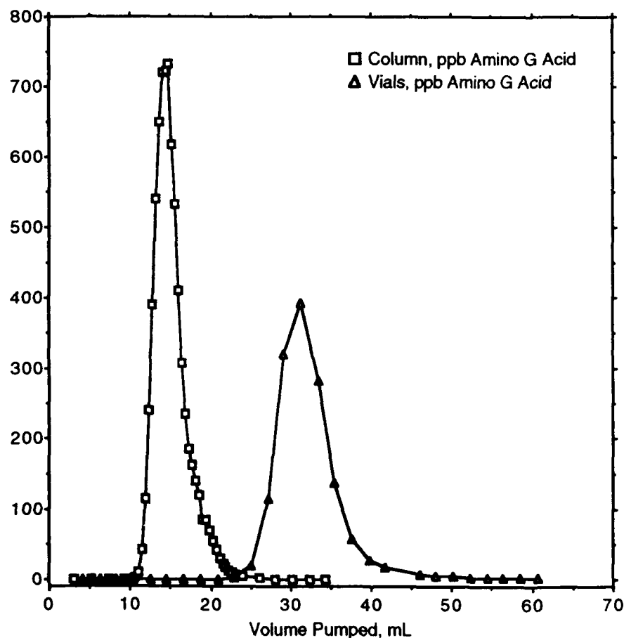
Figure 4. Breakthrough of AGA on Sand (0.2 mL/min Pump Rate).
