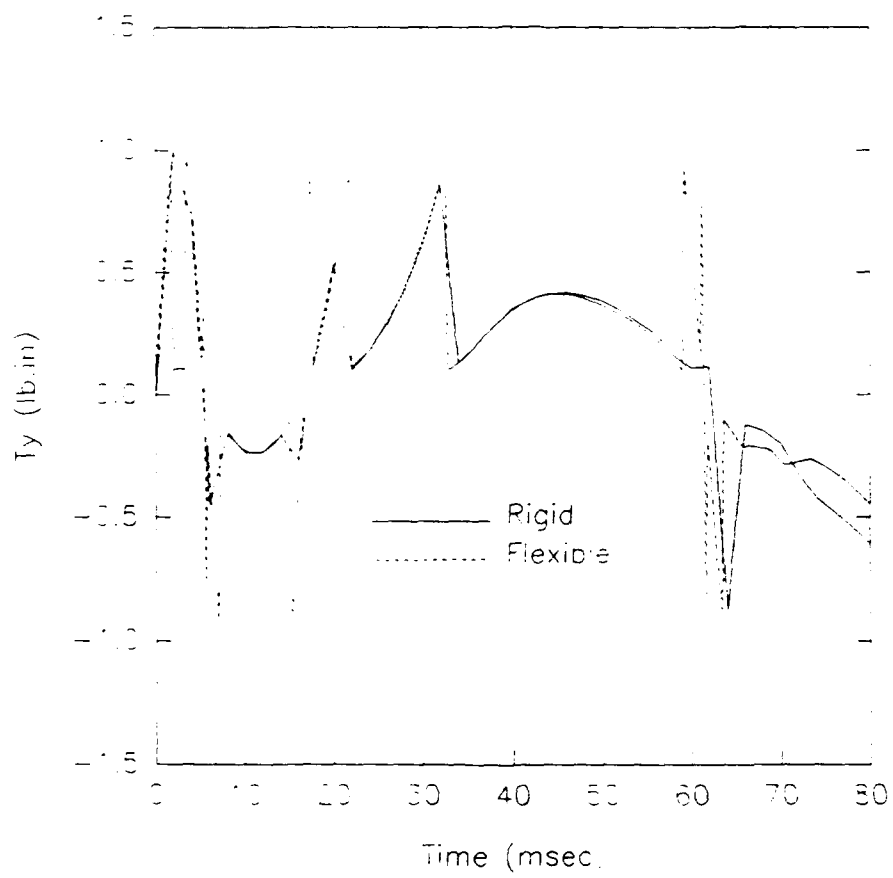
Figure 8. Right Knee Joint Torque about Y-Axis
