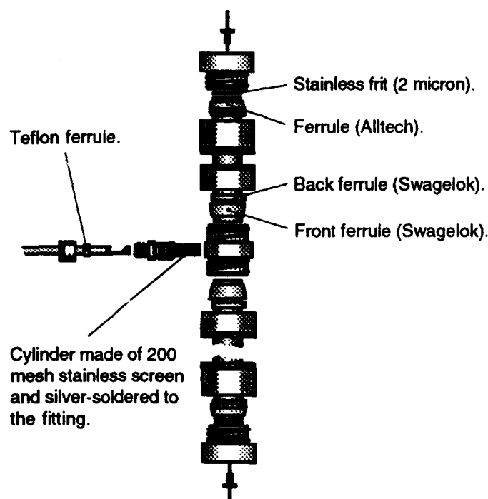
Figure 2. The Soil Column and the Laser Probe Interface.
