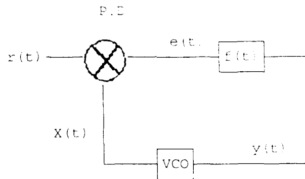
Figure 1 Schematic diagram of phase lock loop
