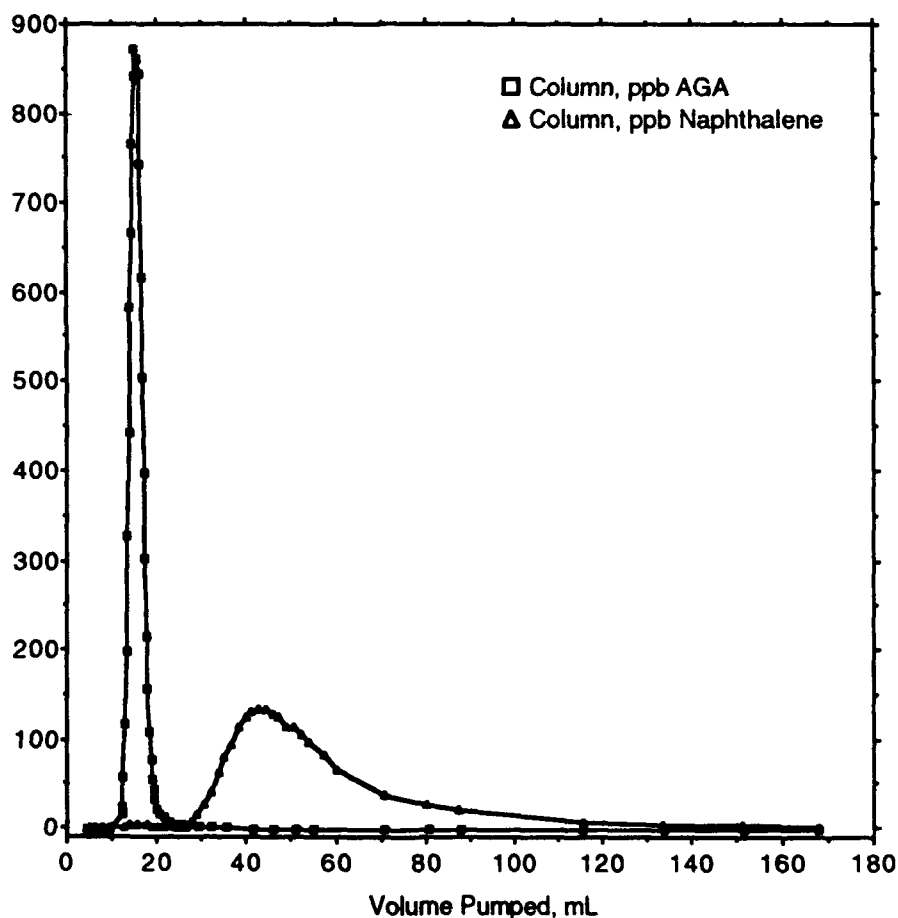
Figure 5. Breakthrough of AGA & Naphthalene on Sand.
