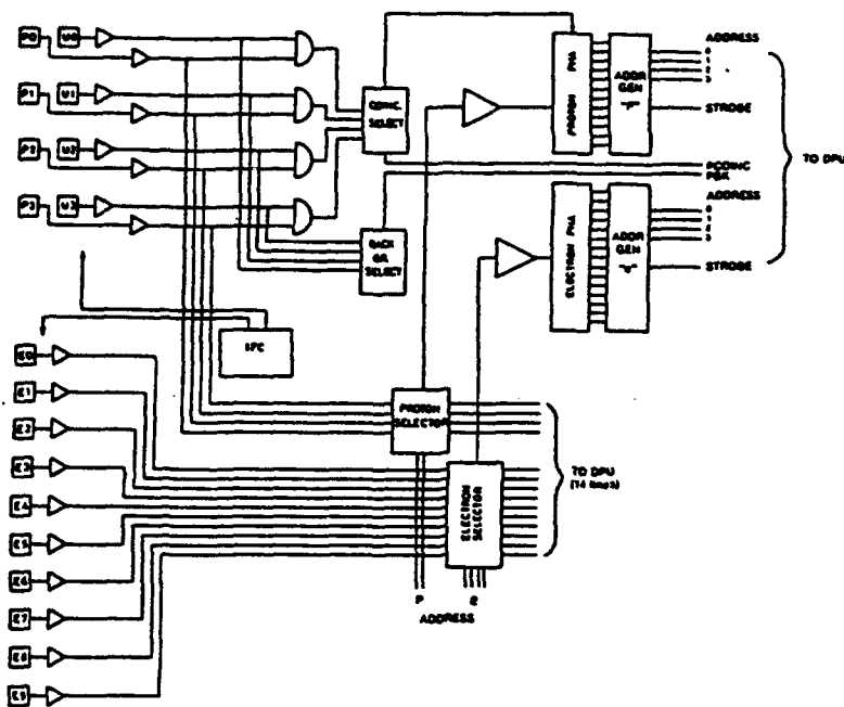
Fig. 3 Block diagram of the analog electronics.
