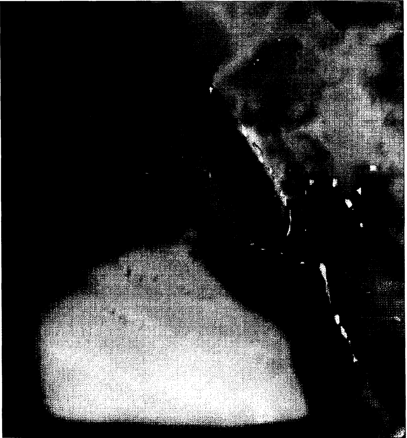
Figure 6. Model Stratus Cloud Fraction, 2030 UTC 02 May 90 (Convective Cloud Fraction Seen Over High Terrain).
