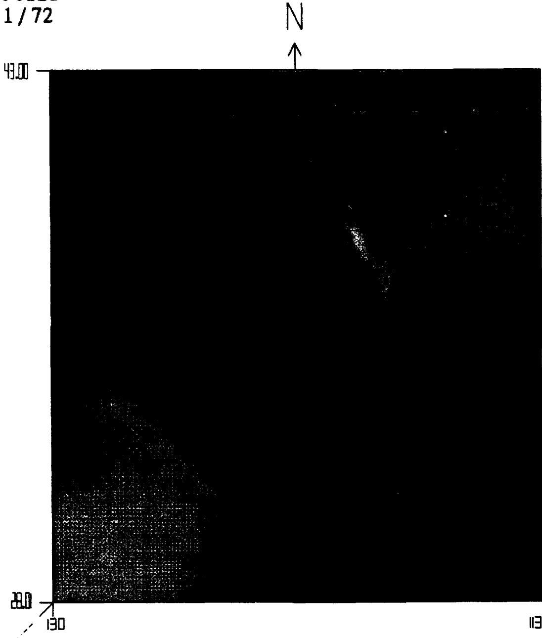
Figure 3. Model Stratus Cloud Fraction, 0030 UTC 02 May 90.
