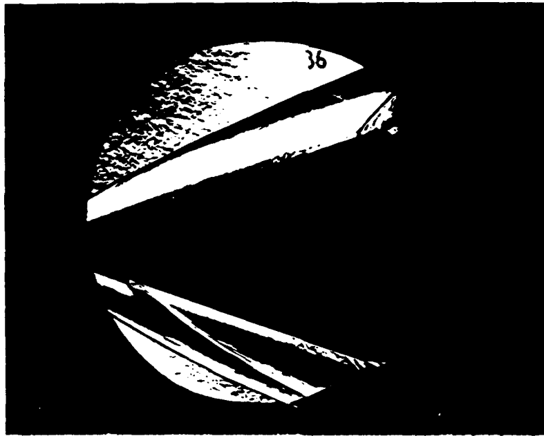
FIGURE 42 SCHLIEREN PHOTOGRAPHY OF FLOW OVER 2D CONFIGURATION WITHOUT COOLING OVER WINDOW ON LOWER SURFACE
