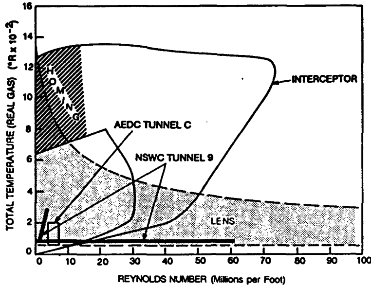
FIGURE 1 TOTAL TEMPERATURE/REYNOLDS NUMBER CAPABILITIES OF THE LENS AND CONTEMPORARY GROUND TEST FACILITIES
