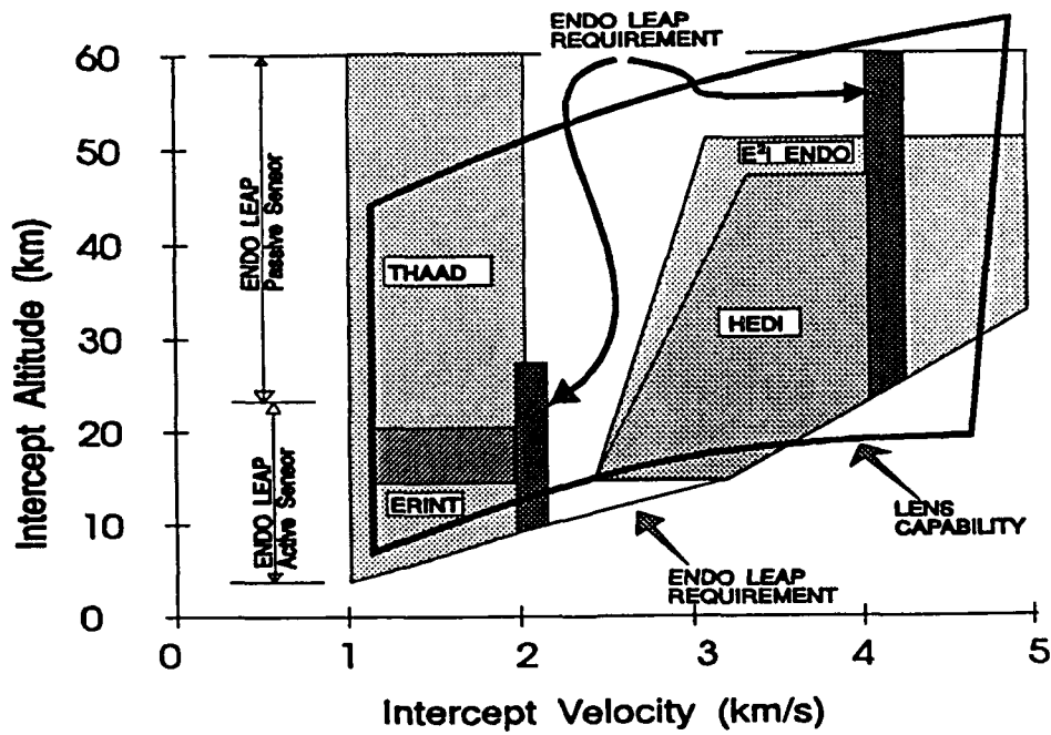
FIGURE 2 INTERCEPTOR PERFORMANCE ENVELOPE AND LENS FACILITY PERFORMANCE
