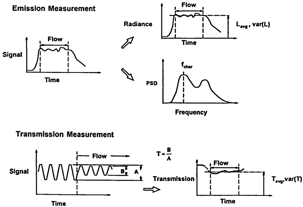
FIGURE 35 IR RADIOMETER DATA PROCESSING PICTORIAL
