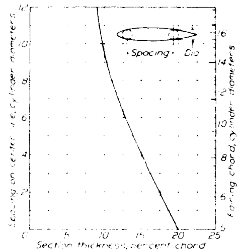
FIGURE 11. Working chart for determining dimensions of tandem strut fairing of minimum drag. Navy no. 1 strut section. NOTE: For tubes of unequal size, use average.
