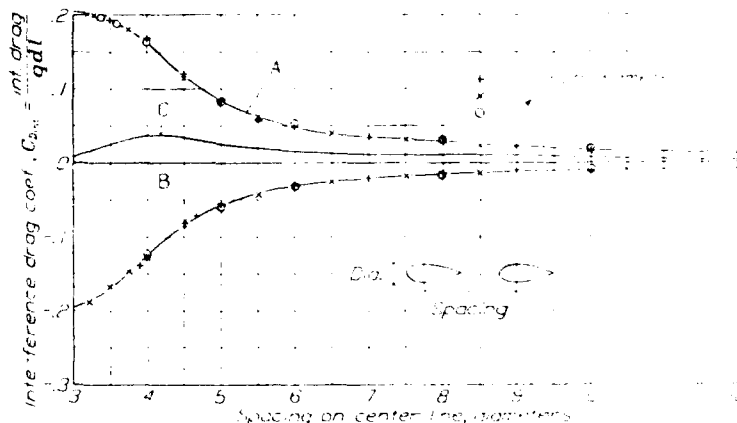
Curve A, rear strut in presence of front strut Curve B, front strut in presence of rear strut Curve C, total interference drag
