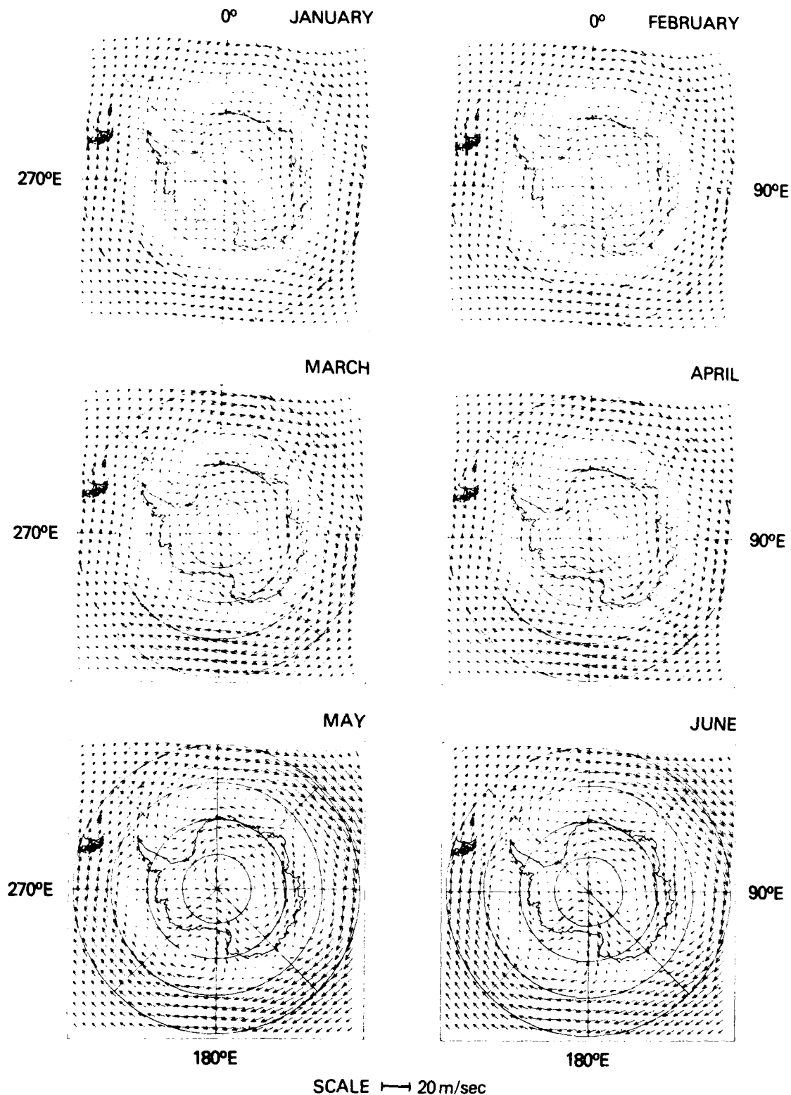
Figure 2-6a. Mean monthly climatological geostrophic winds, January through June. Arrows indicate the direction and relative magnitudes of the wind vectors. The data for these images were obtained in digitized form from Jenne et al. (1974).
