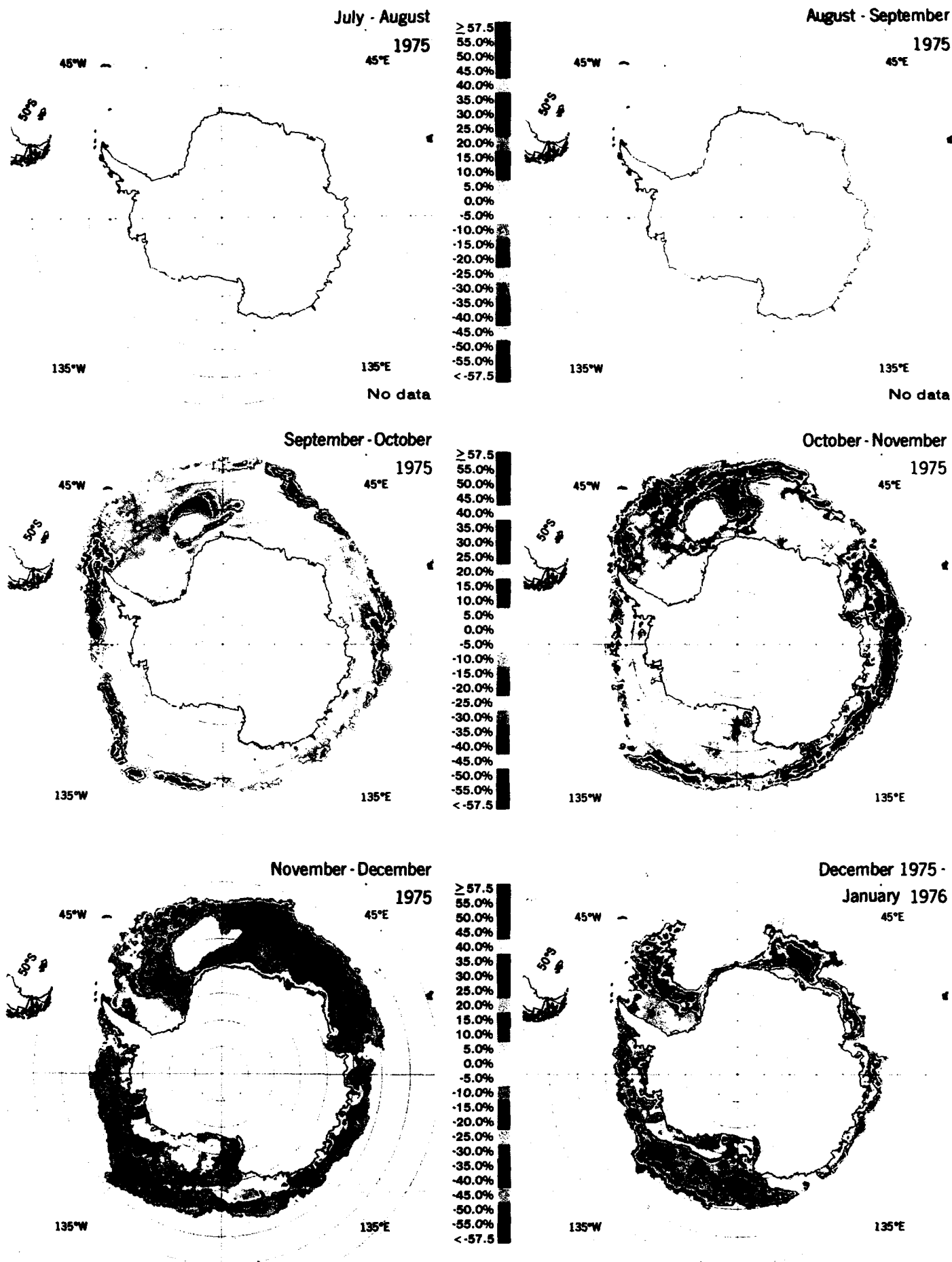
Figure 5-25b. Sea ice concentration monthly change maps for July-August 1975 through December 1975-January 1976.
