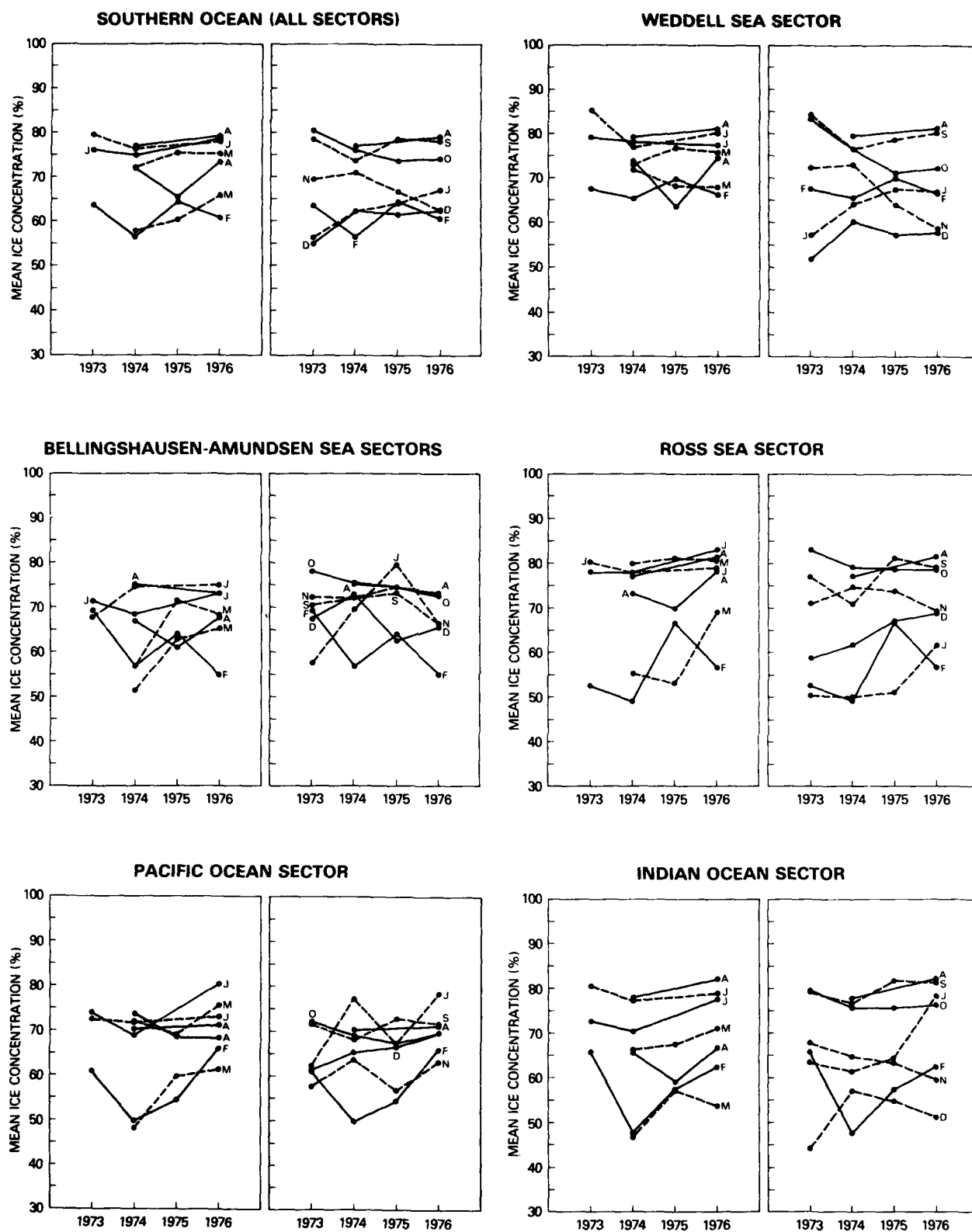
Figure 5-38. Year-to-year changes in mean sea ice concentration, for the total southern ocean and each sector.
