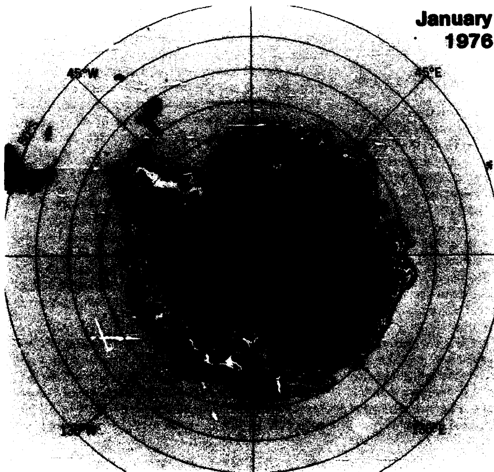
Figure 5-1b. Mean monthly sea ice concentrations for January 1975 and 1976.
