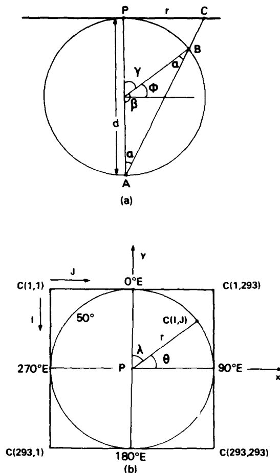
Figure A-4. Schematic diagram for polar stereographic mapping.
