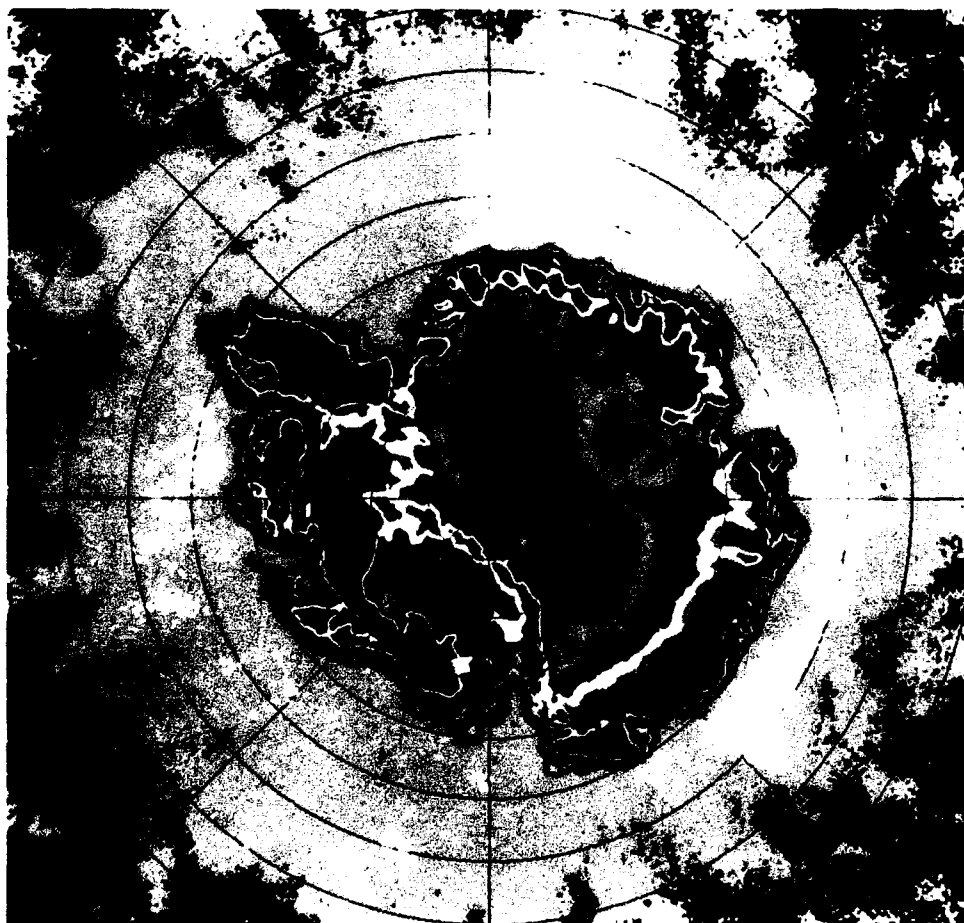
Figure 3-5b. Mean monthly brightness temperatures for February 1975 and 1976.
