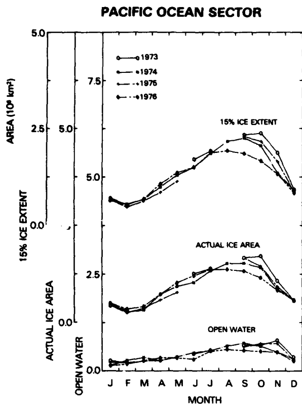
Figure 5-31. Interannual variation of the yearly cycle of the 15-percent extent, the actual ice area, and the open water within the ice pack for the Pacific Ocean sector.
