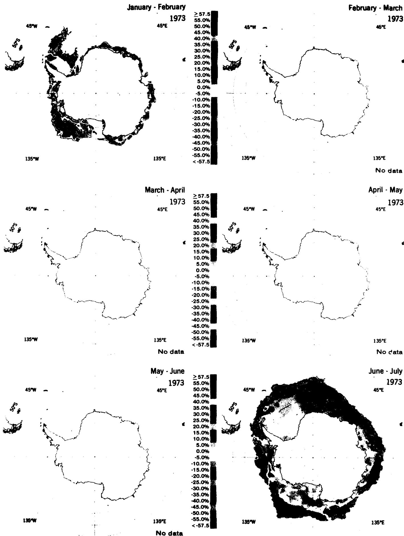
Figure 5-23a. Sea ice concentration monthly change maps for January-February 1973 through June-July 1973.
