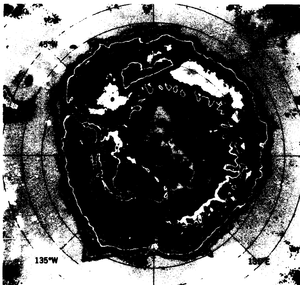
Figure 3-19. Three-year average of mean monthly brightness temperatures for July 1973, 1974, and 1976 and 2-year average for August 1974 and 1976.
