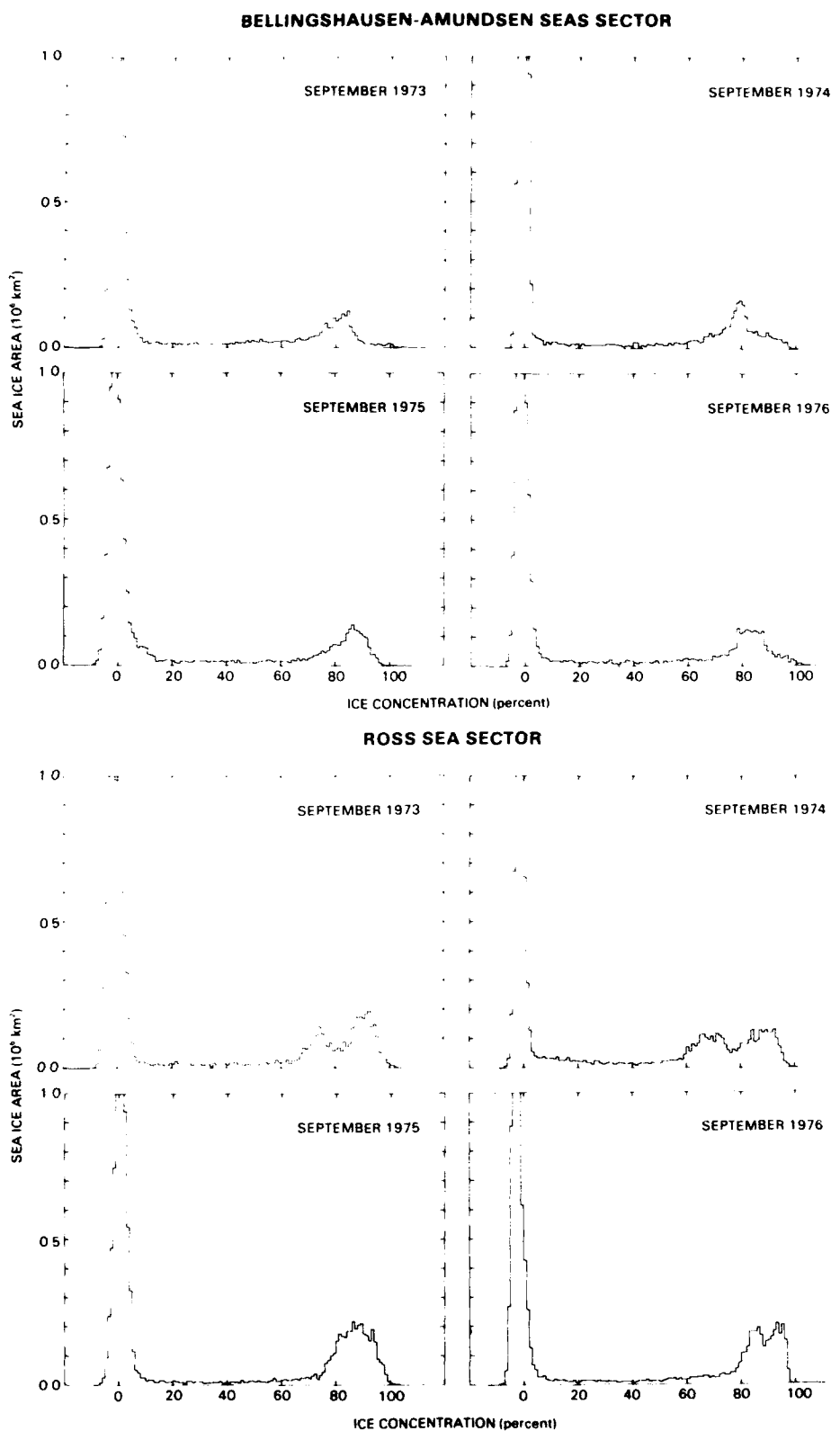
Figure C-5. Year-to-year comparison of areal distribution of percentage ice concentration in the Bellingshausen-Amundsen Seas and the Ross Sea sectors for September.
