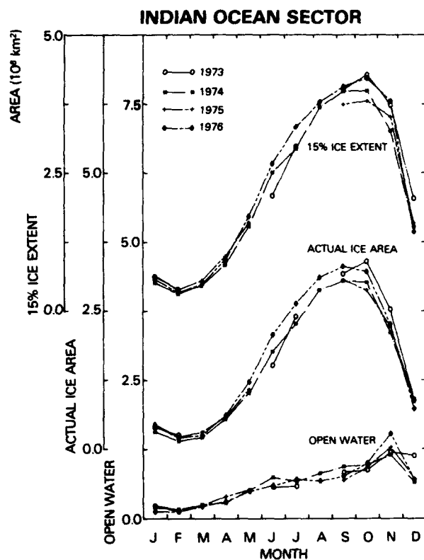
Figure 5-32. Interannual variation of the yearly cycle of the 15-percent extent, the actual ice area, and the open water within the ice pack for the Indian Ocean sector.
