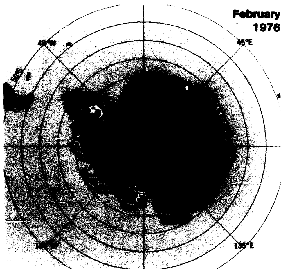
Figure 5-2b. Mean monthly sea ice concentrations for February 1975 and 1976.
