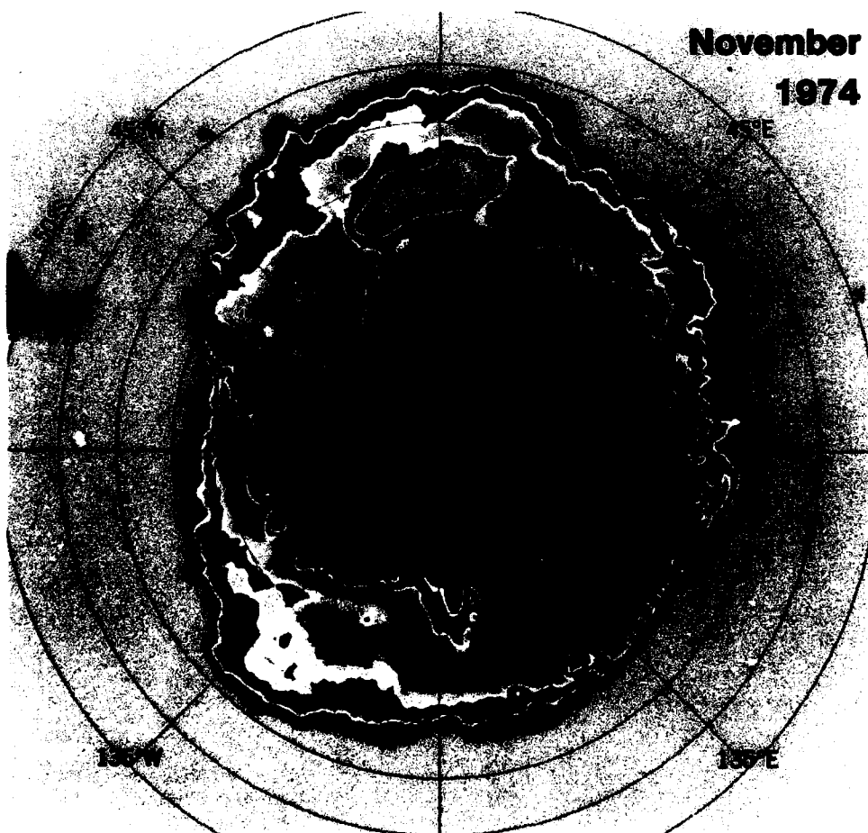
Figure 5-11a. Mean monthly sea ice concentrations for November 1973 and 1974.
