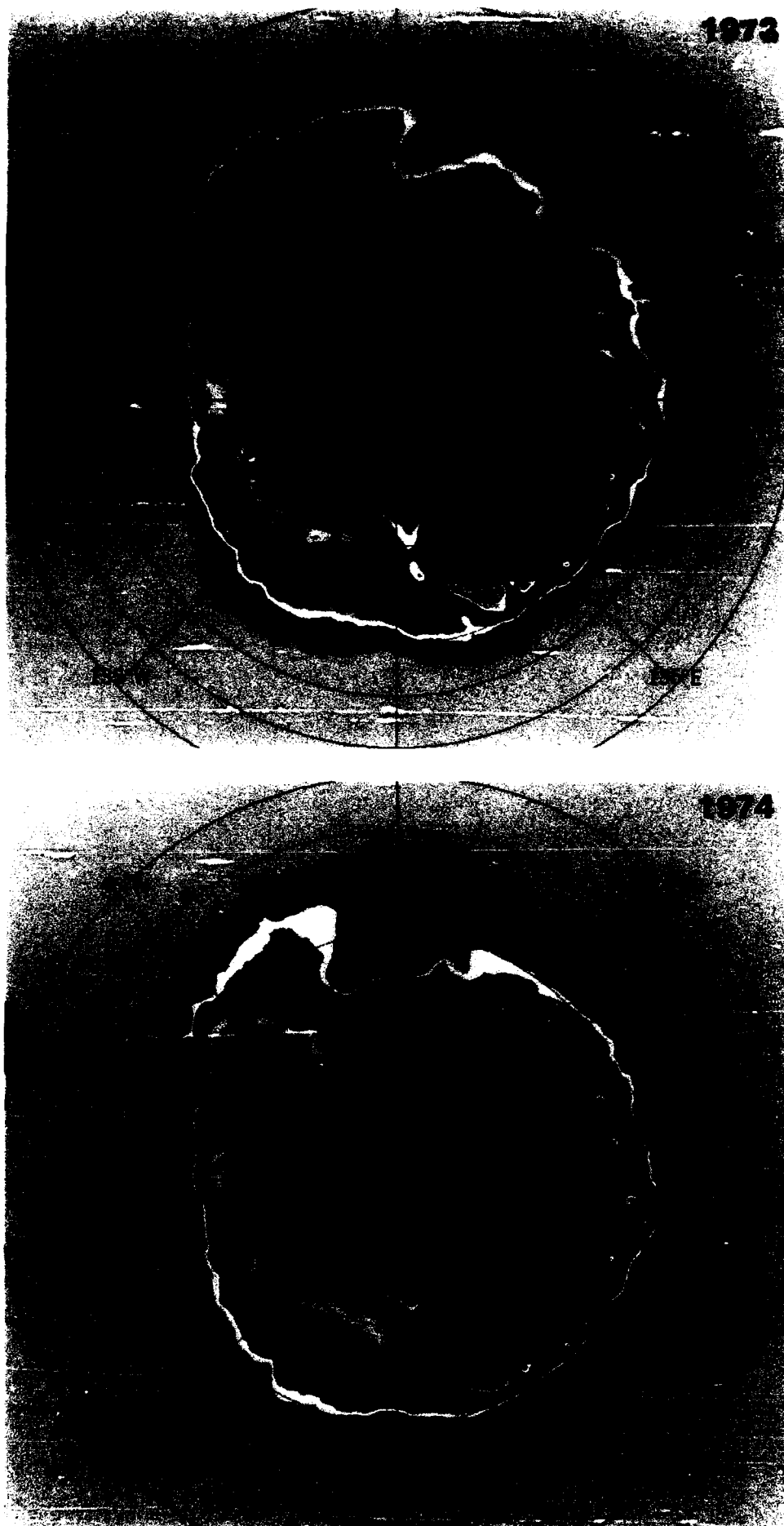
Figure 5-39a. Annual mean sea ice concentrations for 1973 and 1974. Months without data are accounted for by interpolation.
