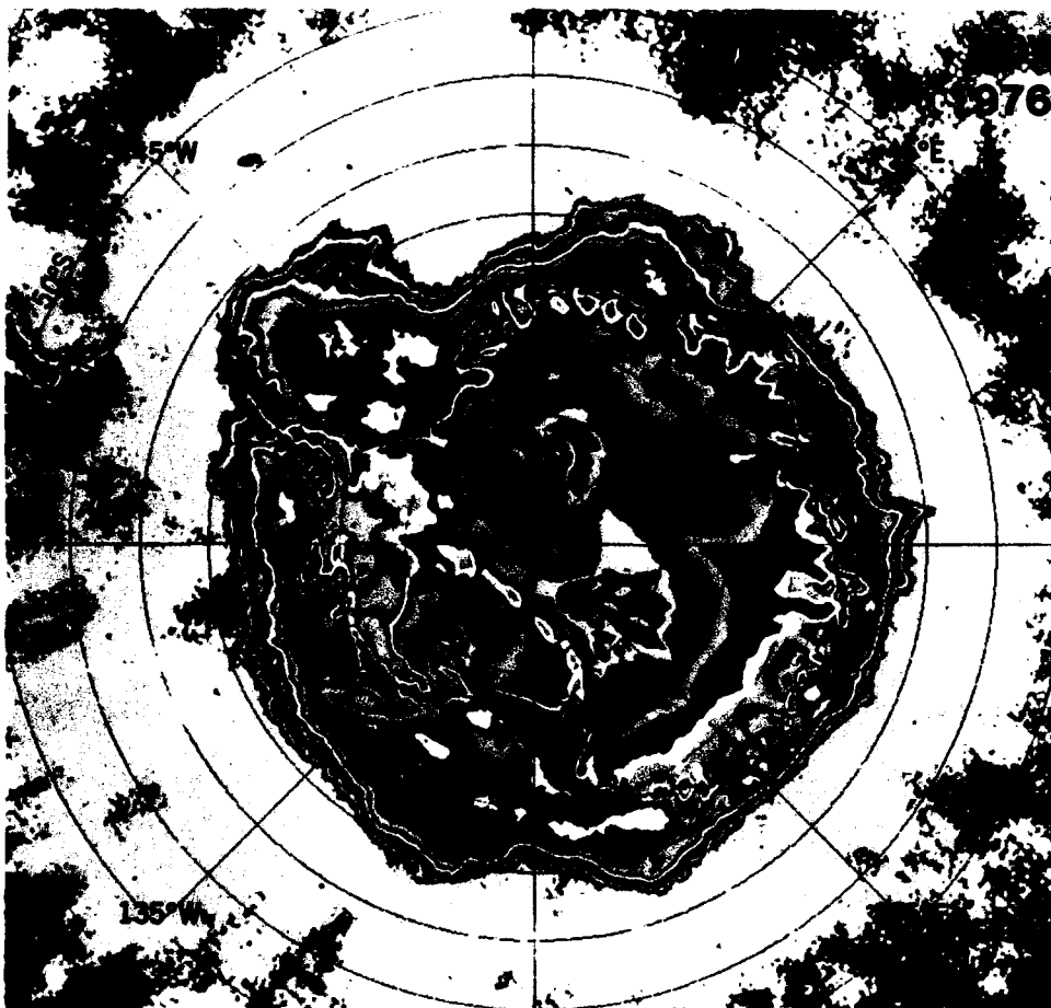
Figure 3-8b. Mean monthly brightness temperatures for May 1975 and 1976.
