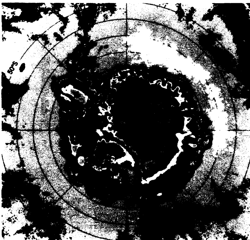
Figure 3-4a. Mean monthly brightness temperatures for January 1973 and 1974.
