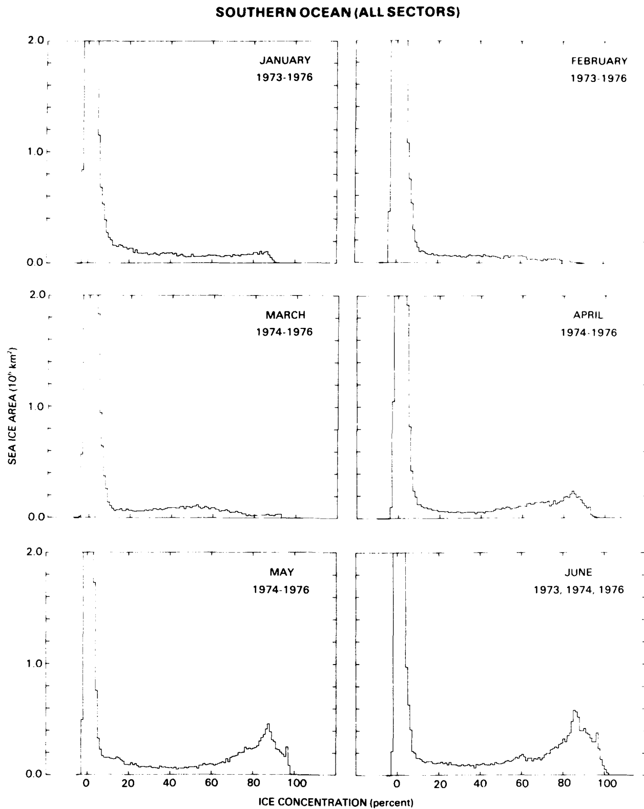
Figure C-1a. Areal distribution of percentage ice concentration in all sectors from January to June (1973-1976).
