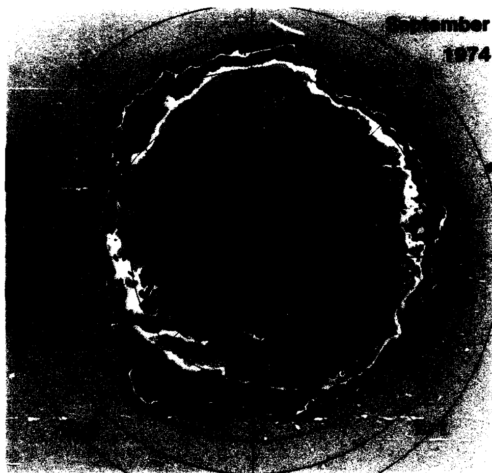
Figure 5-9a. Mean monthly sea ice concentrations for September 1973 and 1974.
