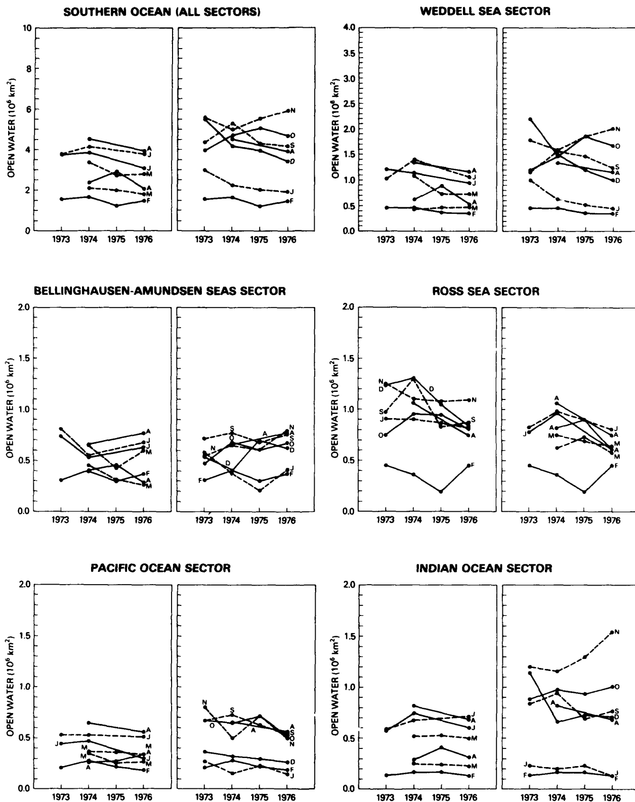
Figure 5-37. Year-to-year changes in open water within the ice pack, for the total southern ocean and each sector.
