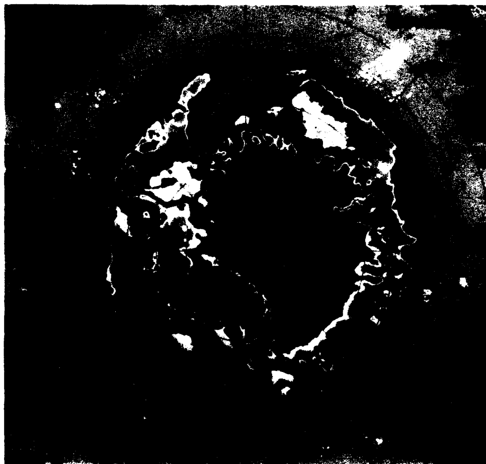
Figure 3-14b. Mean monthly brightness temperatures for November 1975 and 1976.
