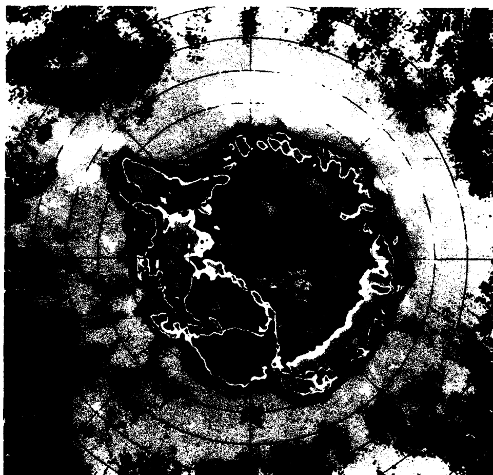
Figure 3-6b. Mean monthly brightness temperatures for March 1975 and 1976.
