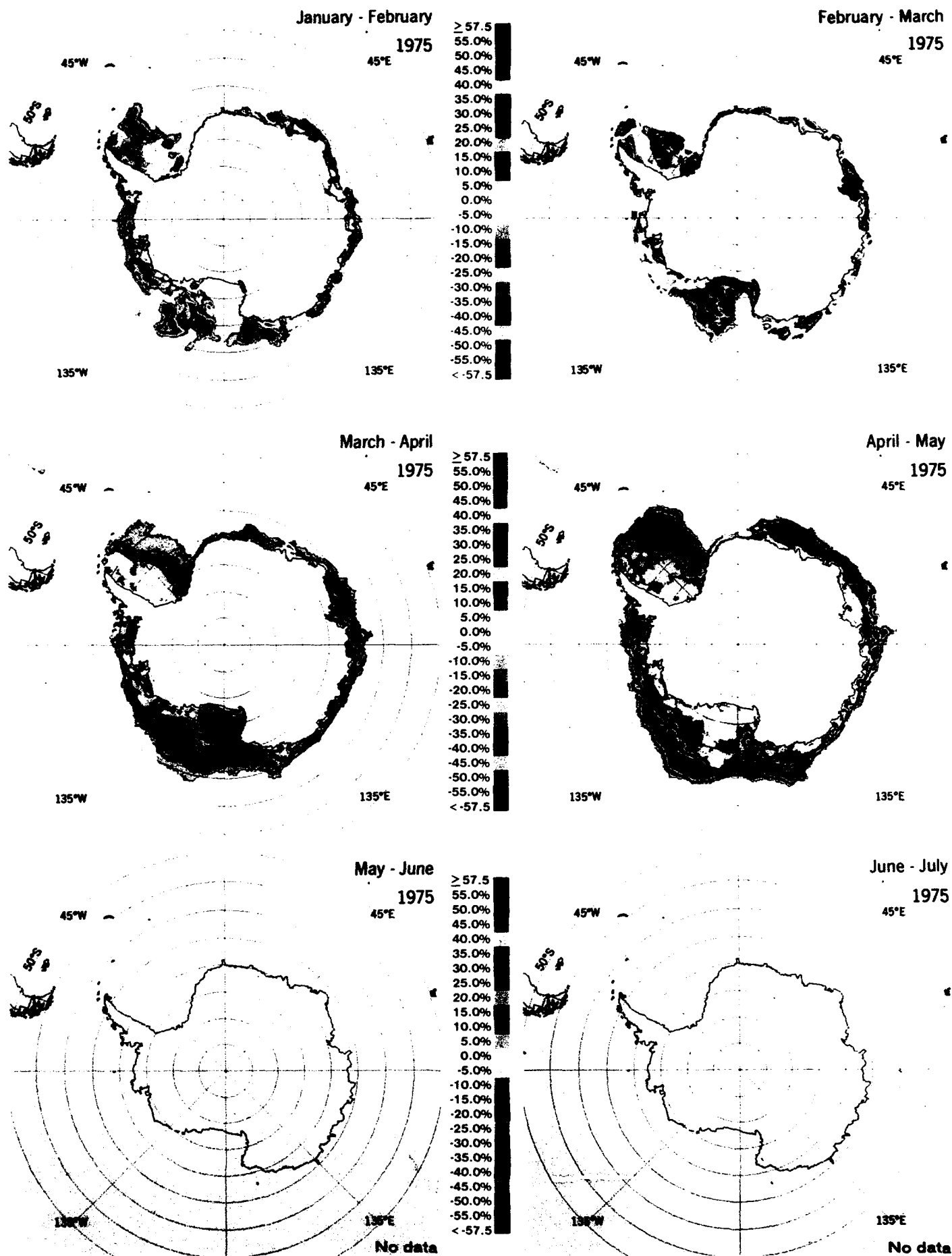
Figure 5-25a. Sea ice concentration monthly change maps for January-February 1975 through June-July 1975.
