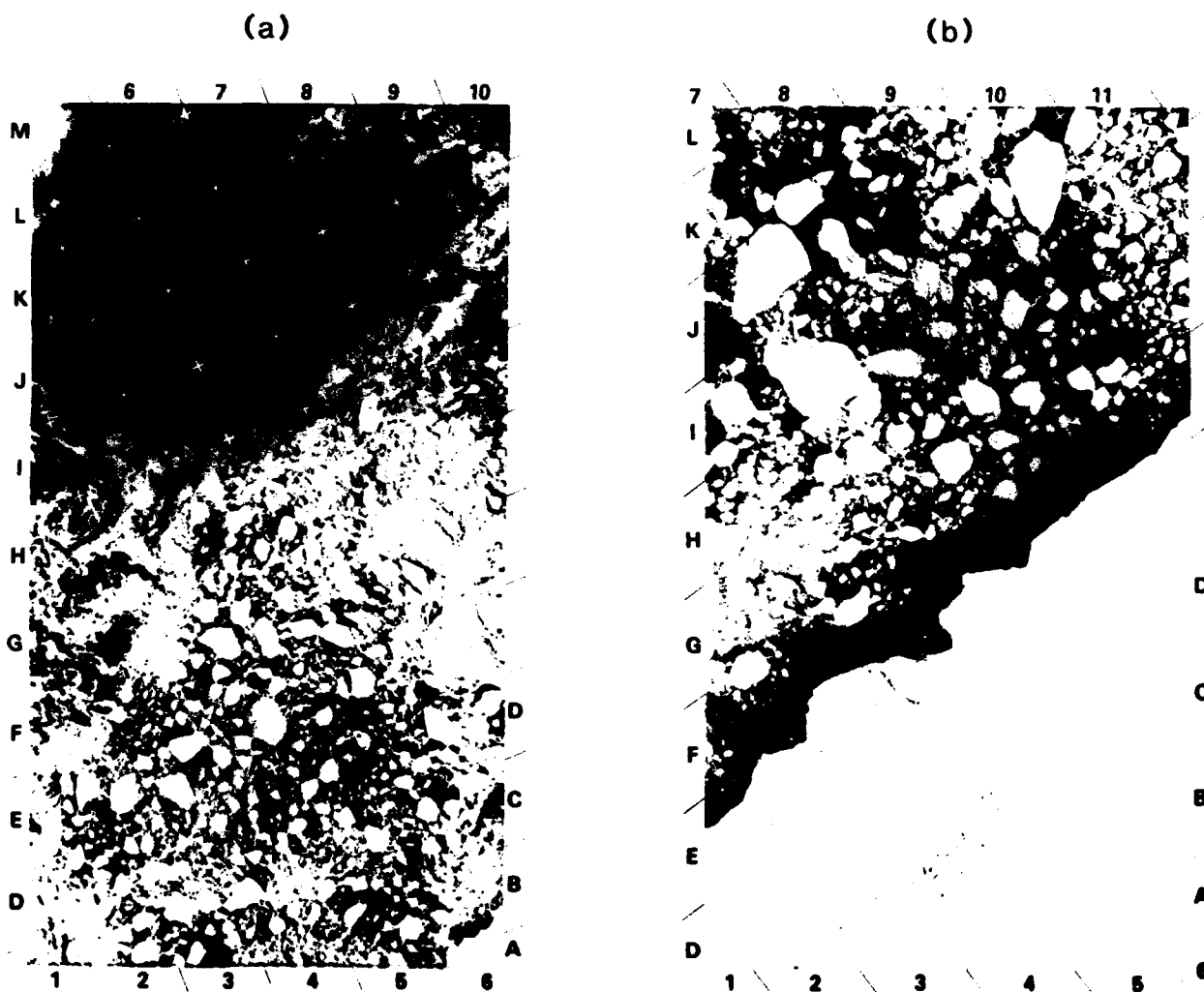
Figure 3-25. Landsat multispectral scanner images at near-infrared (1.1 microns) wavelengths: (a) image for November 23, 1975, centered at 68°1'S, 4°49'W and (b) image for November 13, 1973, centered at 69°2'S, 9°16'E.
