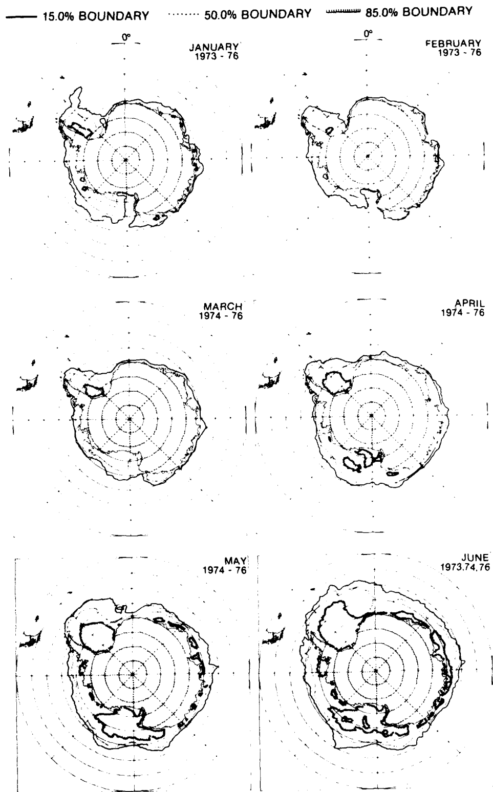
Figure B-11a. Mean monthly ice concentration contours for January through June, averaged for the years indicated.
