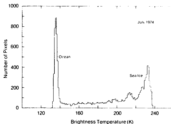
Figure 3-27. Distribution of brightness temperature derived from ESMR data in the Weddell Sea sector (60°W to 20°E) during July 1974.
