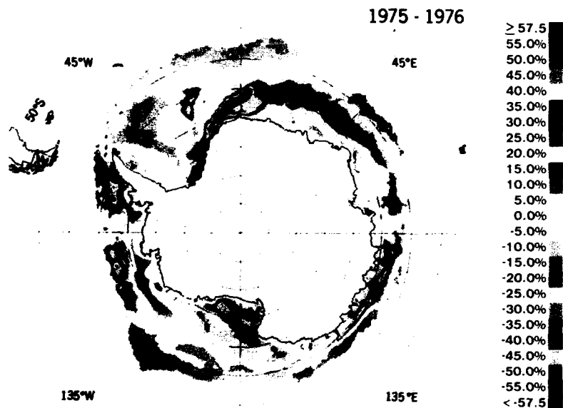
Figure 5-40. Change in annual mean sea ice concentrations from 1973 to 1974, from 1974 to 1975, and from 1975 to 1976.
