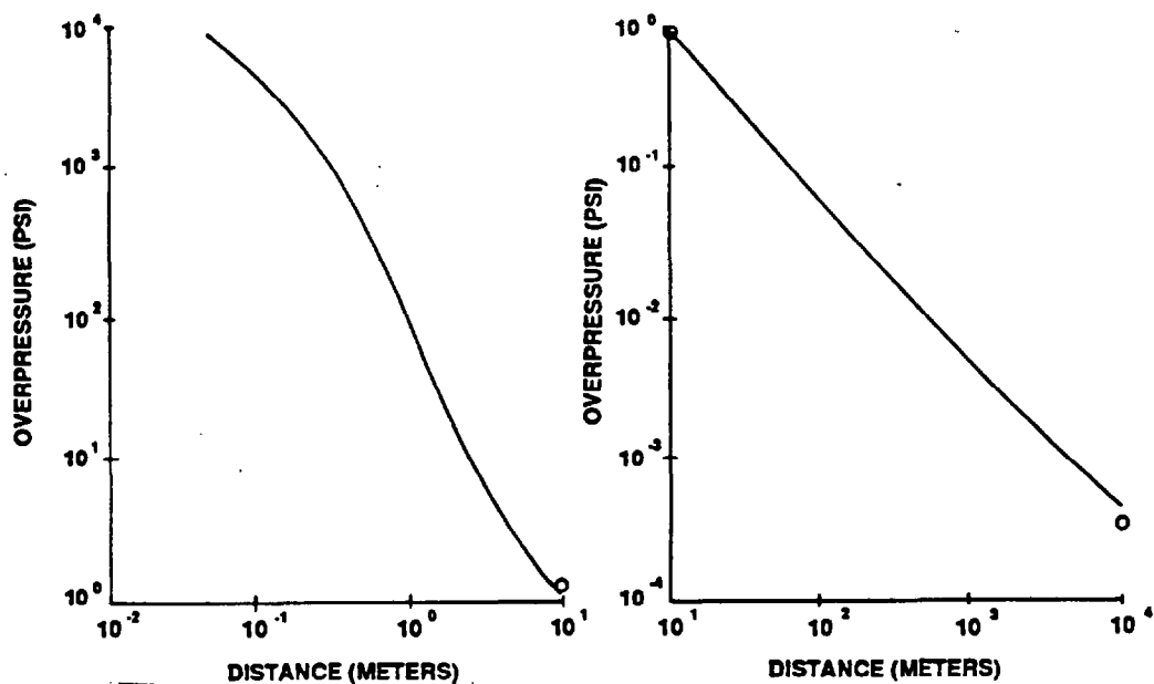
Figure 8. Peak free field overpressure vs. distance due to the detonation of a 0.454-kg (1-lb) charge of TNT at sea level: a) near field and b) far field.
