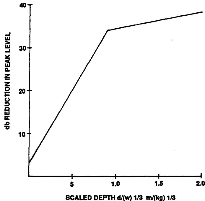
Figure 11. Buried correction - peak overpressure level vs. scaled depth.
