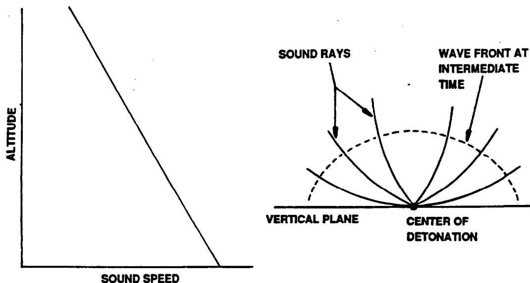
Figure 4. Sound wave propagation from a detonation on the earth surface with a negative sound velocity gradient.
