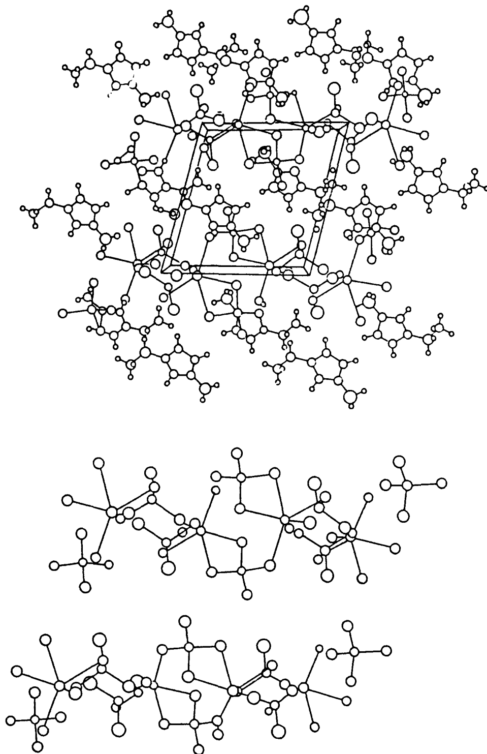
Crystal structure of the MEIC-NaCl-AlCl 3 salt. The composition is a congruently melting material with the ions in ratios of MEI + :Na + :AlCl 4 - = 1:1:2. The top figure shows the packing of layers of MEI + ions interspersed with NaAlCl 4 layers. The structures of the MEI + have been deleted in the bottom figure to emphasize the Na + ...AlCl 4 - network.
