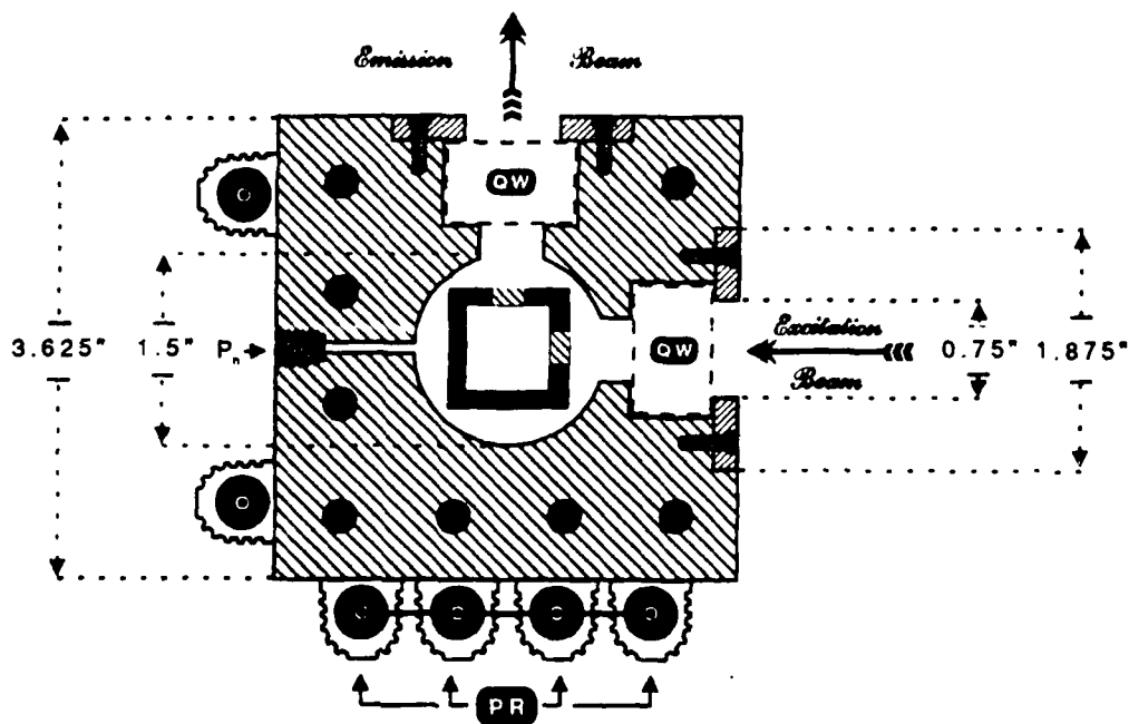
FIG. 2—Cross-sectional view through the center of the steel chamber body. Center , central bore containing the fixed cuvette holder; fused silica windows ( QW ); flange securing window to body; penetration port ( Pn ) for RTD or pressurization line; and metal jacketed power resistors ( PR ) for heat exchange.
