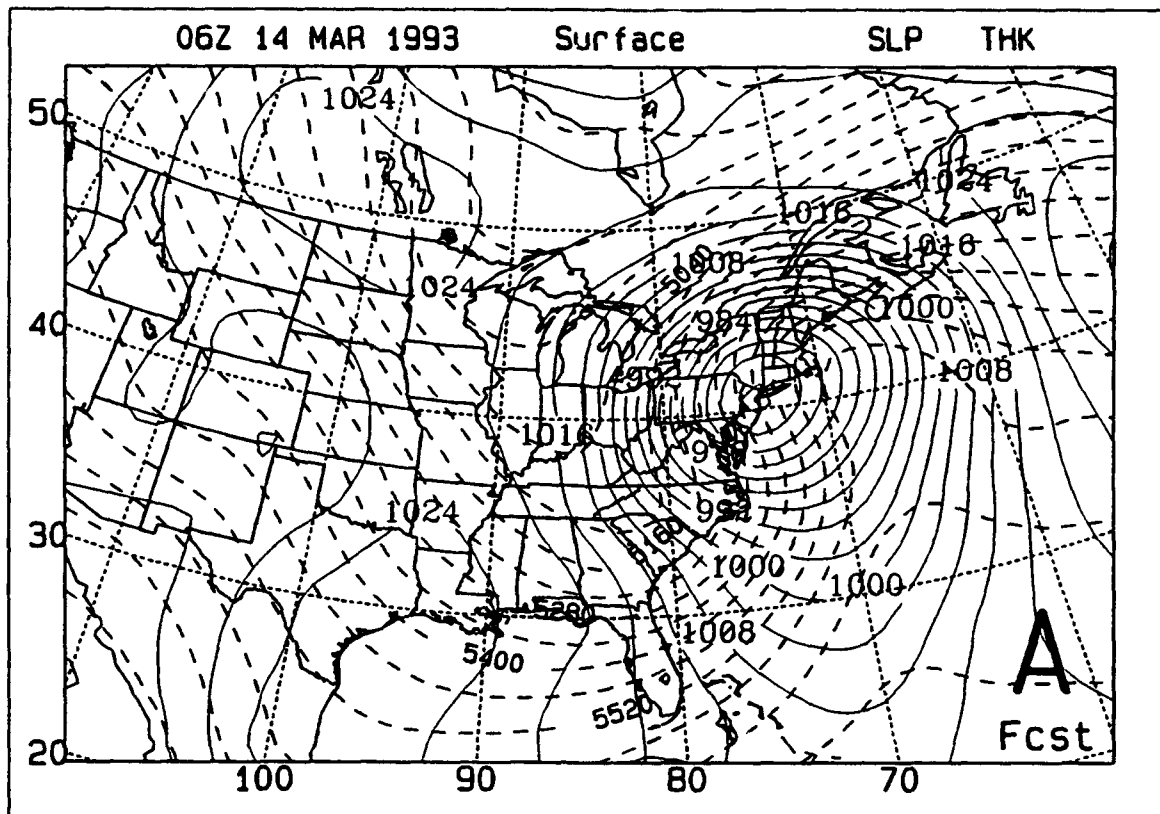
Figure 23. As in Figure 8, except for 42 h forecast verifying at 0600 UTC 14 March 1993.
