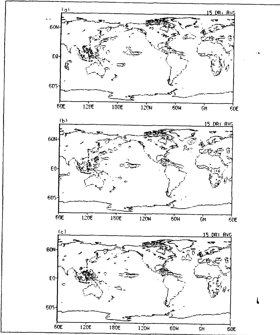
Figure 11. 15 day average atmospheric heating for Forecast 2: (a) POSITIVE, (b) NO, (c) NEGATIVE runs. Minimum contour is 2°C/day. Contour interval is 1°C/day.
