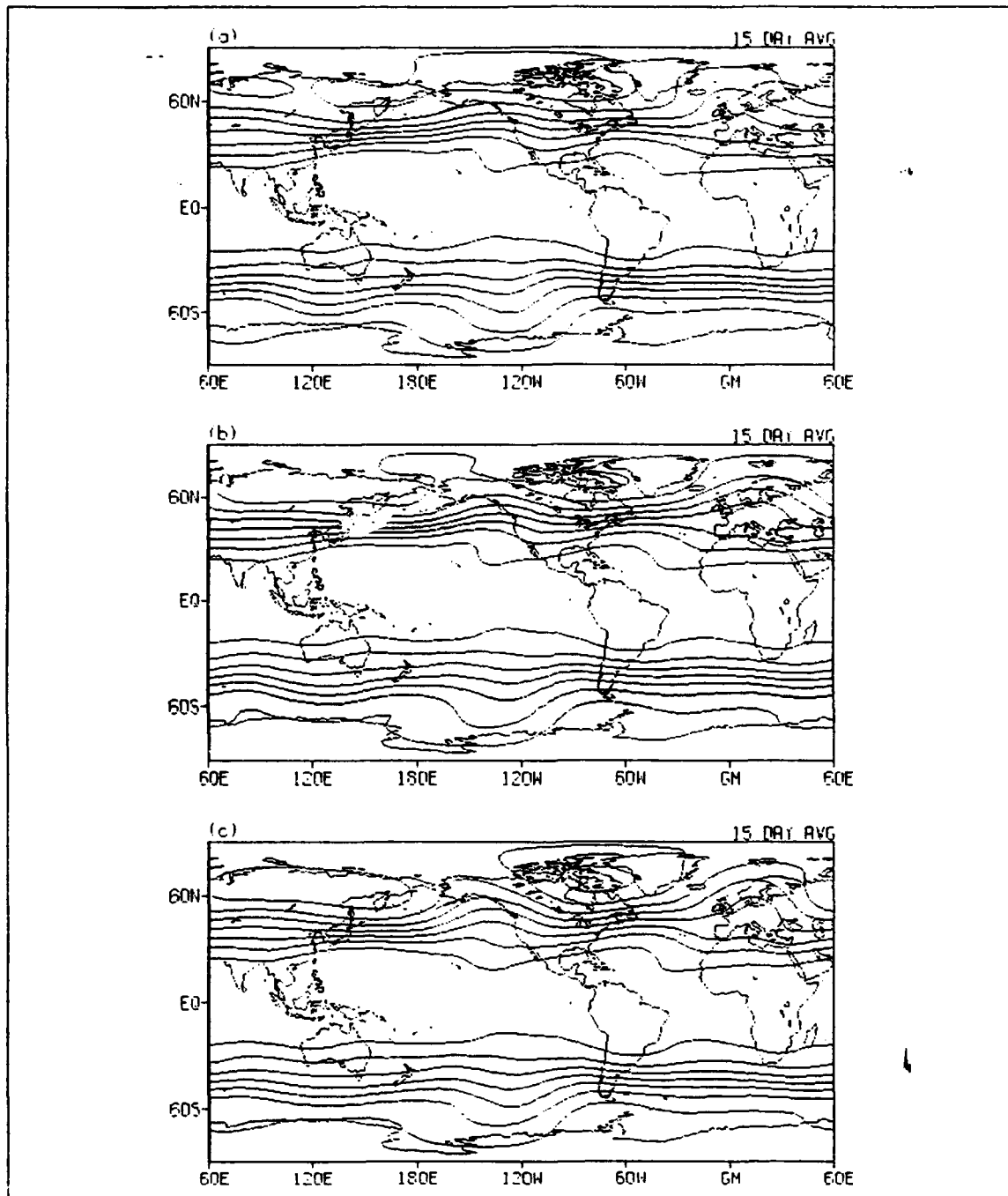
Figure 12. 15 day average 200 mb geopotential height for Forecast 2: (a) POSITIVE, (b) NO, (c) NEGATIVE runs. Minimum contour is 10500 gpm. Contour interval is 200 gpm.
