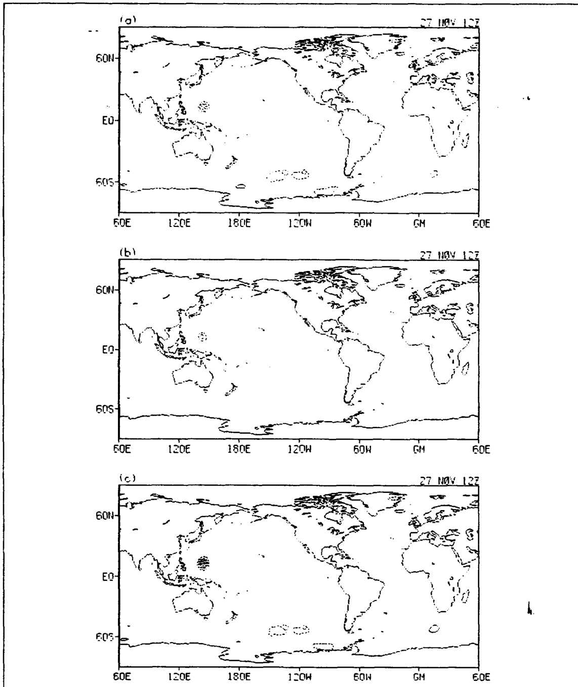
Figure 6. Differences in sea level pressure initial conditions for Forecast 2: (a) POSITIVE - NO, (b) NO - NEGATIVE, (c) POSITIVE - NEGATIVE differences. Contour interval is 4 mb.
