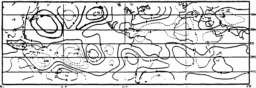
(b) Outgoing Longwave Radiation
