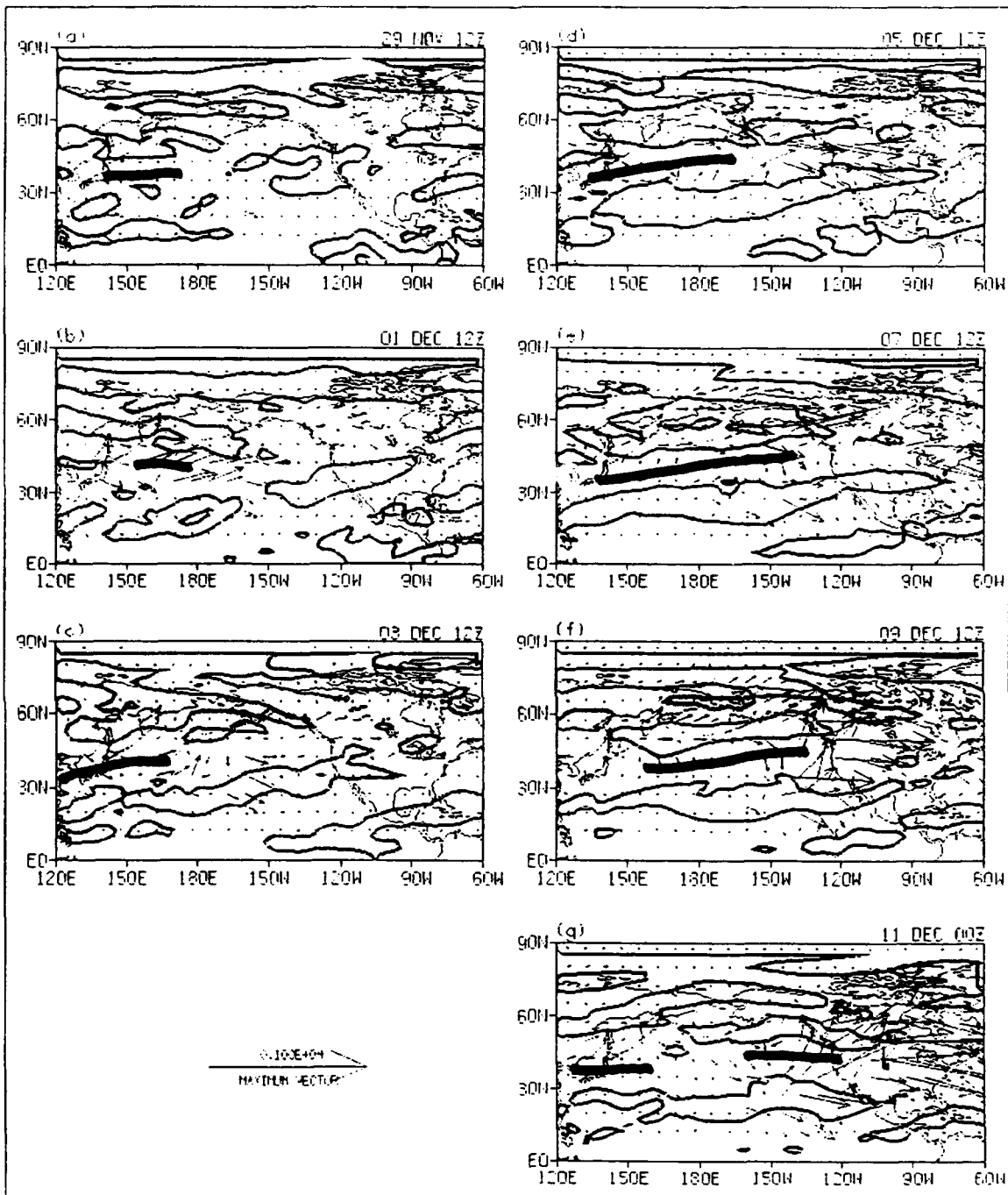
Figure 35. EA QG wave activity flux vectors ( m^2/s^2 ) overlaid with POSITIVE 200 mb jet axis and POSITIVE 200 mb potential BTI. Jet ( u > 60 m/s) is thick black line. BTI contour is 0 m^{-1}s^{-1} .
