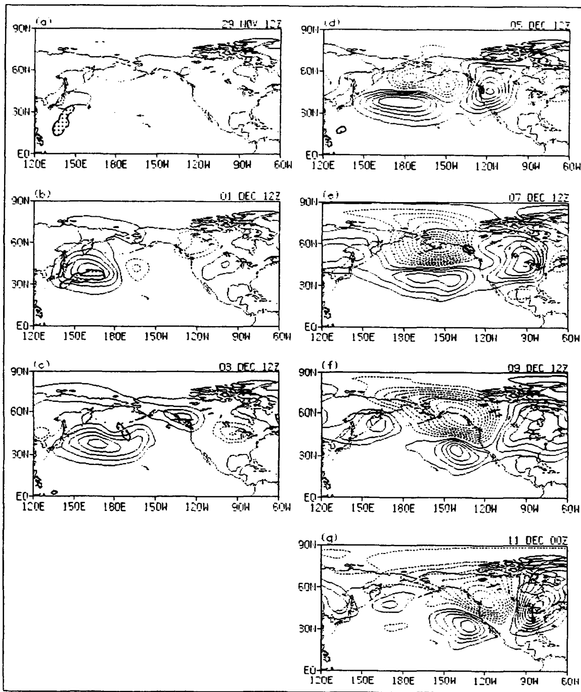
Figure 30. EA differences (POSITIVE-NEGATIVE) heating and 200 mb heights. Solid (dashed) contours represent positive (negative) height differences; contour interval is 50 gpm. Dotted areas shows heating difference > 5°C/day.
