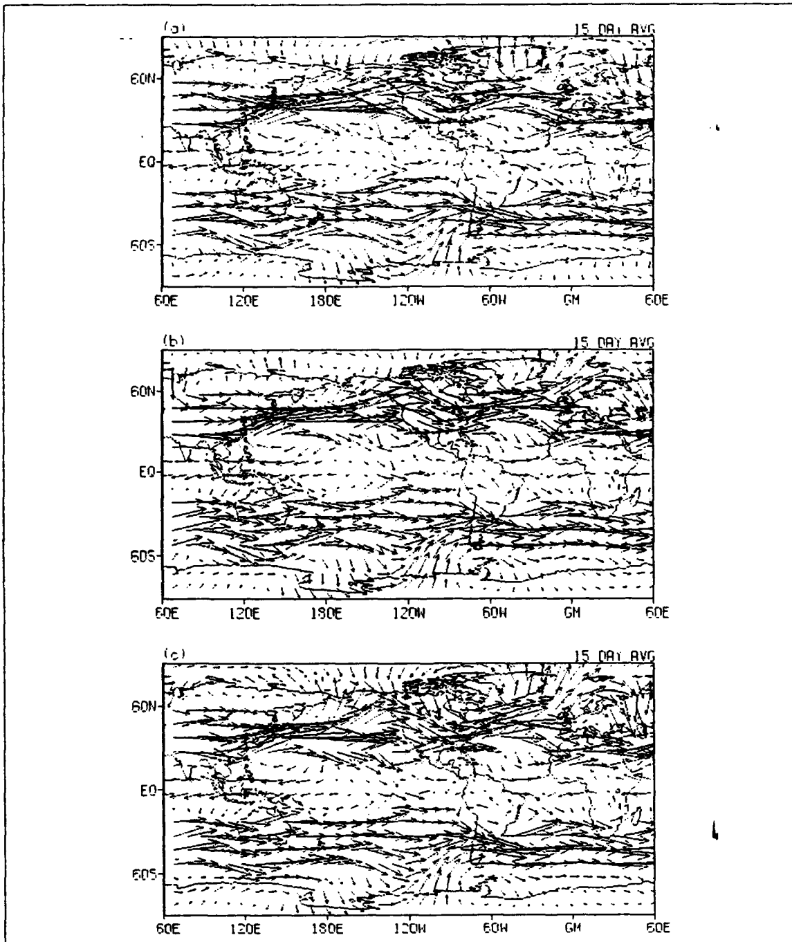
Figure 13. 15 day average 200 mb winds for Forecast 2: (a) POSITIVE, (B) NO, (C) NEGATIVE runs. Vector scale (m/s) as indicated.
