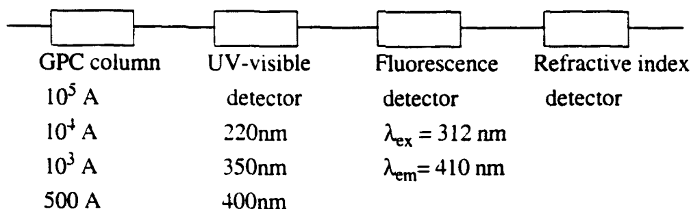
Scheme 2 Scheme of instrumentation for end group analysis
