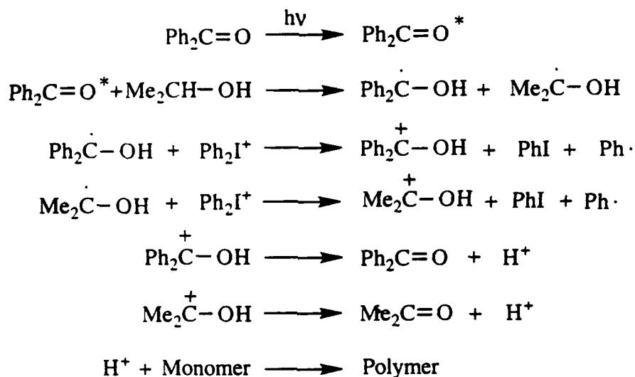
Scheme 1 Radical promoted cationic polymerization
