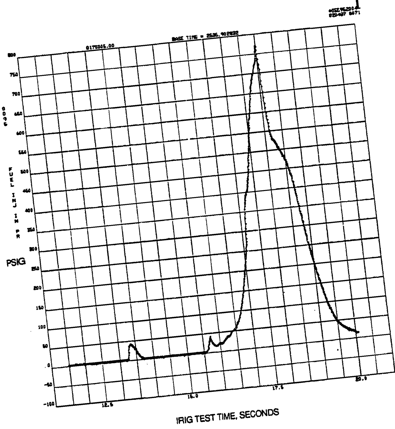
Figure 7-67 FUEL INJECTOR PRESSURE VERSUS TEST TIME - 87-017-005
