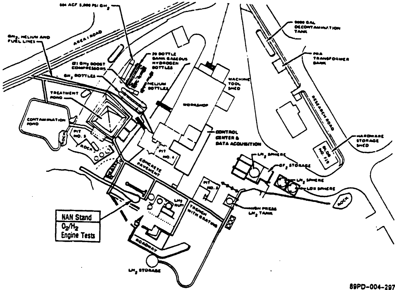
Figure 7-14 APTF OVERVIEW
