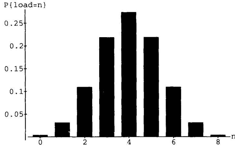
Figure 3.2: Loading probability mass function for an eight-channel bundle, where each channel carries a message with probability 1/2 .
