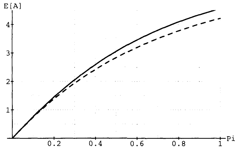
Figure 3.13: The bandwidth of the 16 \times 16 indirect cube made from 4 \times 4 crossbars, as depicted in Figure 3.9, is shown dashed. The bandwidth of the variant with a first stage made from 8 \times 4 , dilation 2 switches, as depicted in Figure 3.10, is shown in solid black. Both are plotted against the source transmission probability, for a uniform destination address distribution.
