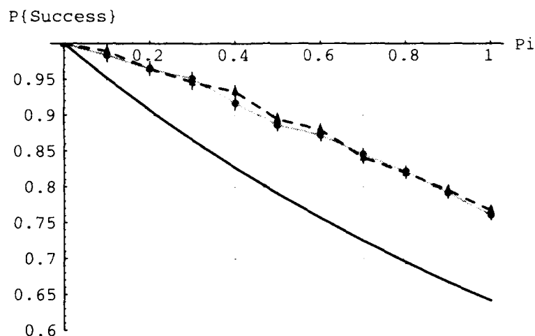
Figure 5.13: The probability of successful message transmission is shown for each of the three networks in Figures 5.11, 5.12, and 5.7. The results for the replicated network are shown in black, and are exact; the results for the deterministically-interwired network are shown in grey, and those for the randomly-interwired network are shown dashed. See the text for a discussion of the results.
