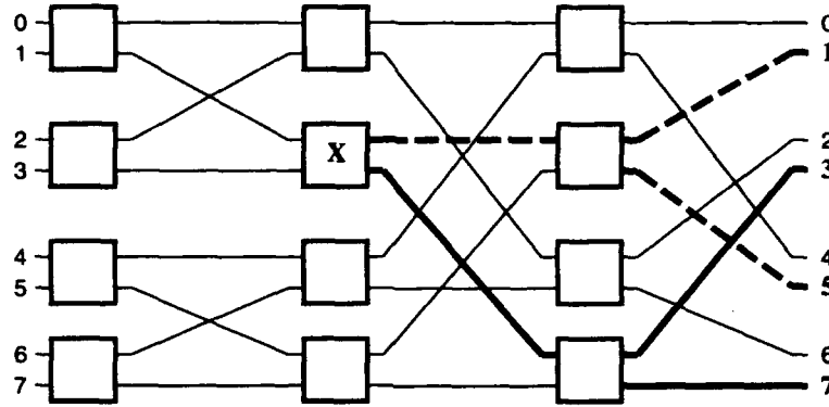
Figure 3.5: The destination set of the switch X is \{1, 3, 5, 7\} . The destination set of the upper channel is \{1, 5\} ; that of the lower channel is \{3, 7\} .
