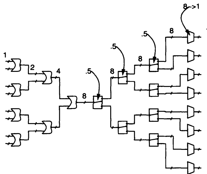
Figure 3.6: Schematic representation of an 8 \times 8 crossbar network. Here we show the switching probabilities set for a uniform destination address distribution.
