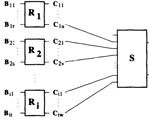
Figure 4.3: Channels referred to in Equation (4.2). Although the probabilities of the message loads on the channels C_{11}, \dots, C_{iw} are not in general independent, the loads on the subset of channels from each switching element are independent given the message loads on the input channels B_{11}, \dots, B_{it} .
