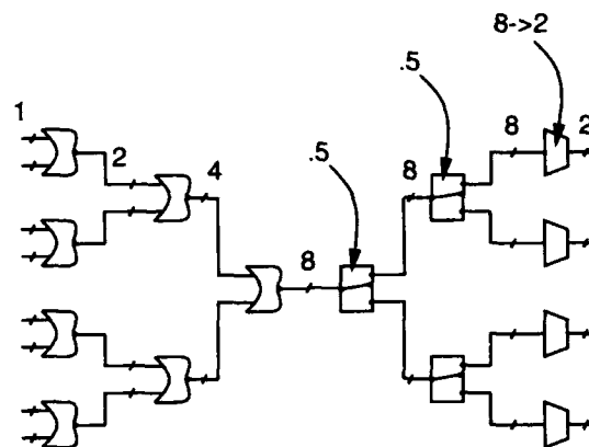
Figure 3.11: Schematic representation of an eight-by-four, dilation two switching component. The switching probabilities are for a uniform destination address distribution.
