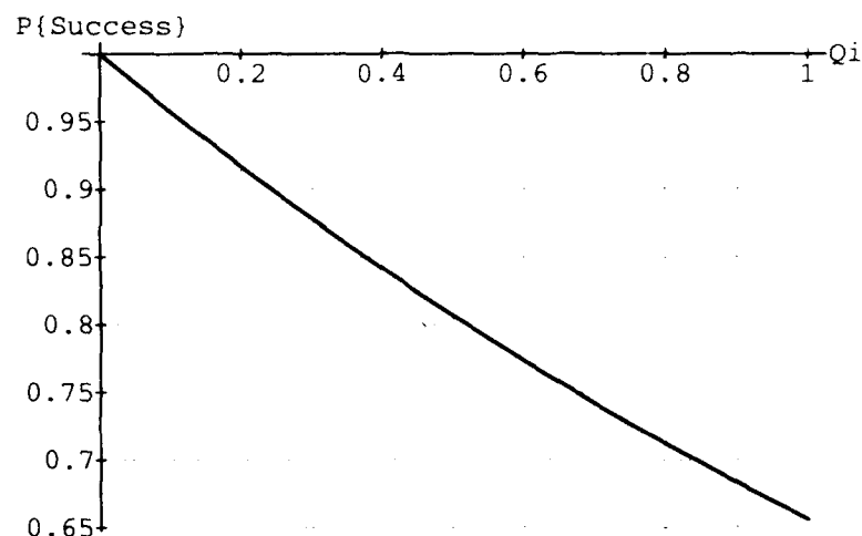
Figure 3.7: The probability of successful message transmission (labeled P\{\text{Success}\} ) as a function of the probability that a source is transmitting (labeled Q_i ), in an eight-by-eight crossbar network with a uniform destination distribution.
