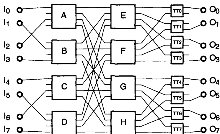
Figure 4.5: The network of Figure 4.1, with switches labeled.
