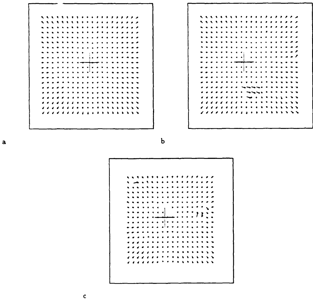
Figure 10: An example of optical flows computed by using (a) 2D-2D , (b) 1D-2D and (c) 1D-1D . In most frame pairs in a sequence the three flows are much more similar to each other.
