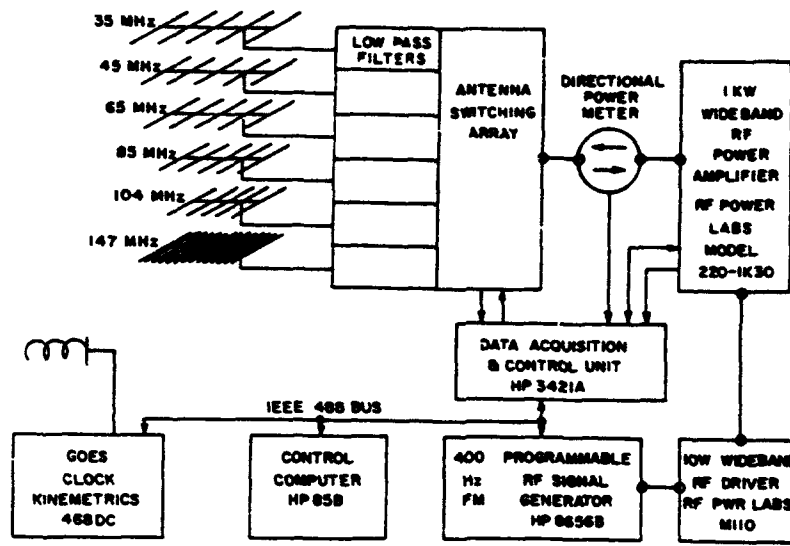
TRANSMITTER
