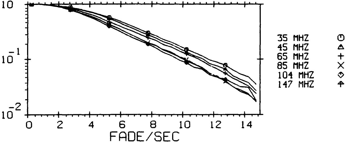
NORMALIZED DISTRIBUTION OF FADES/SECOND FOR JUNE 1991
