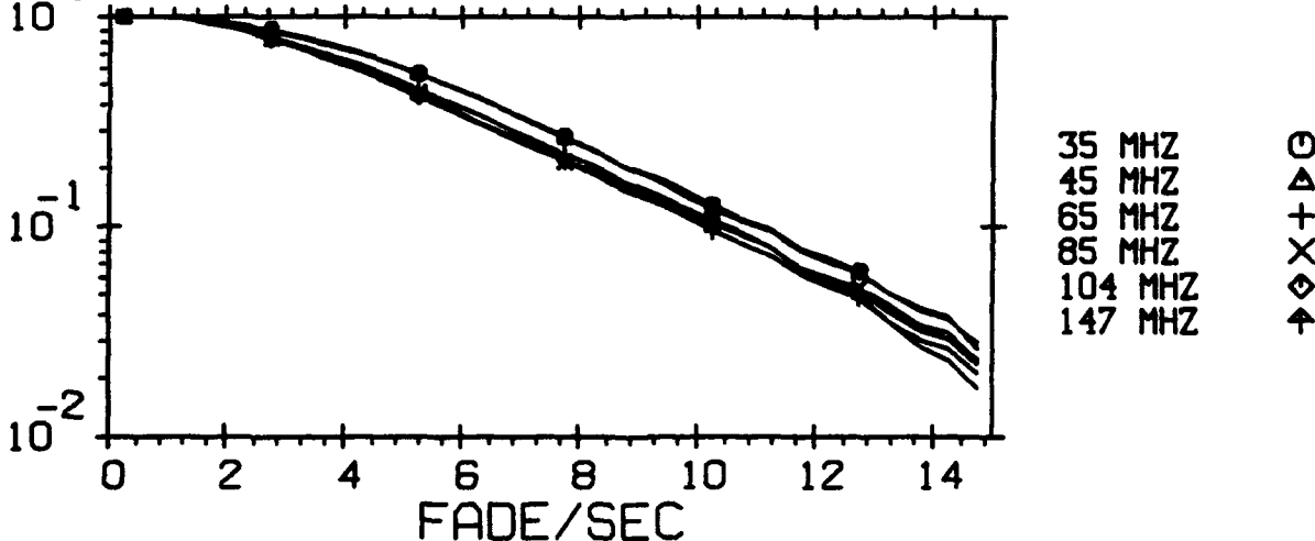
NORMALIZED DISTRIBUTION OF FADES/SECOND FOR AUGUST 1991
