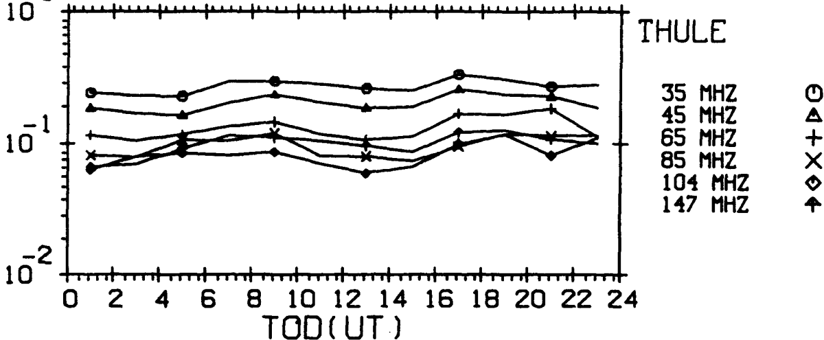
AVERAGE UNDERDENSE TIME CONSTANT VS TIME FOR AUGUST 1991
