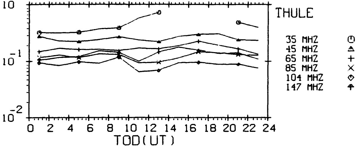
AVERAGE UNDERDENSE TIME CONSTANT VS TIME FOR JUNE 1991
