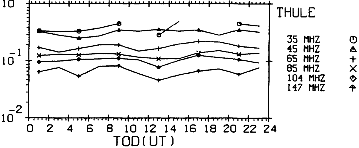
AVERAGE UNDERDENSE TIME CONSTANT VS TIME FOR JUNE 1990
