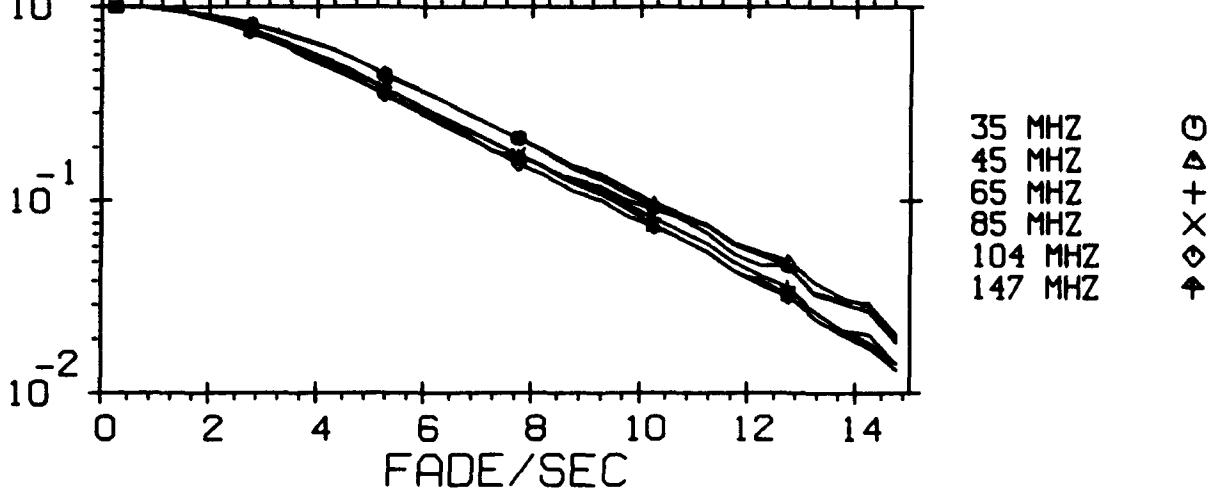
NORMALIZED DISTRIBUTION OF FADES/SECOND FOR JUNE 1990
