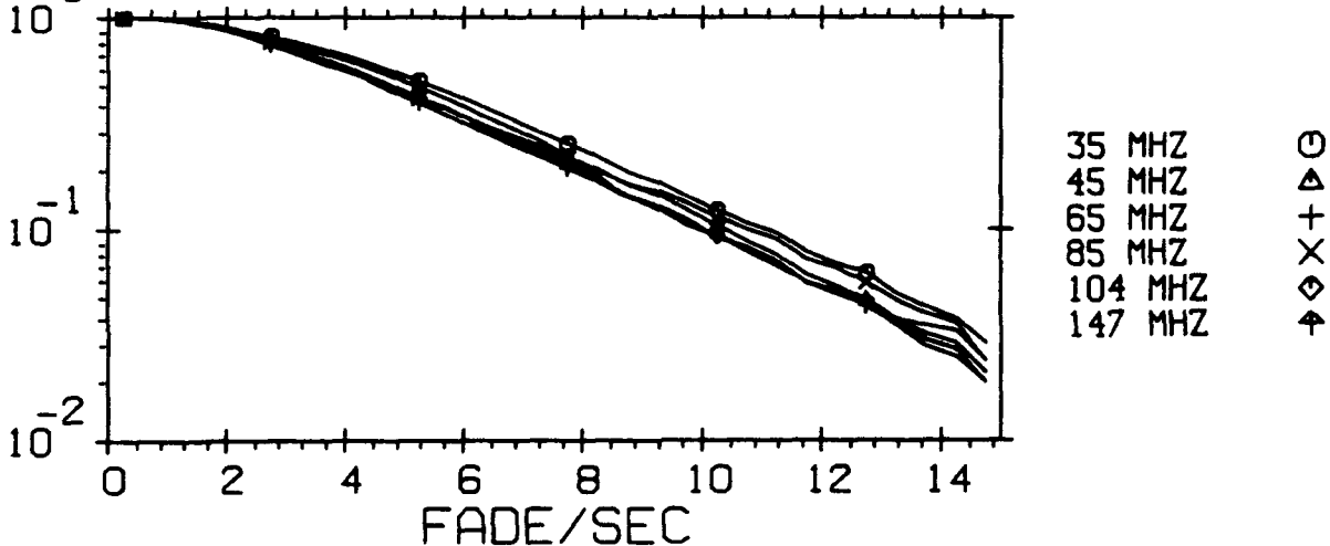
NORMALIZED DISTRIBUTION OF FADES/SECOND FOR APRIL 1992
