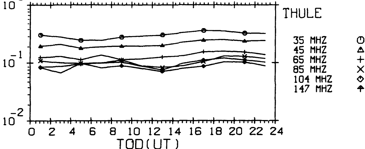
AVERAGE UNDERDENSE TIME CONSTANT VS TIME FOR APRIL 1992
