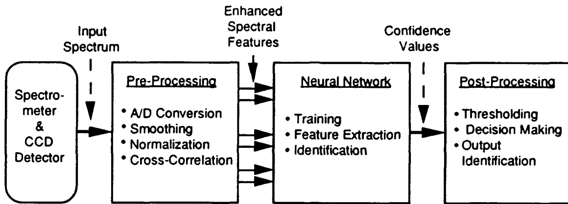
Figure 2 Schematic diagram of POC's neural-network-based spectral signal processing.
