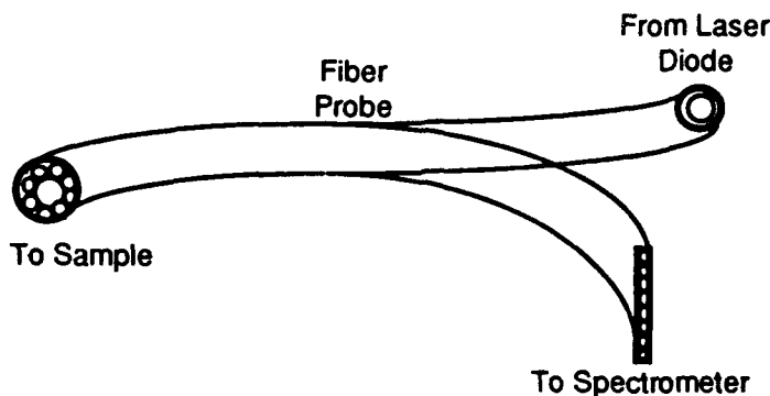
Figure 6 Structure of the fiber probe.
