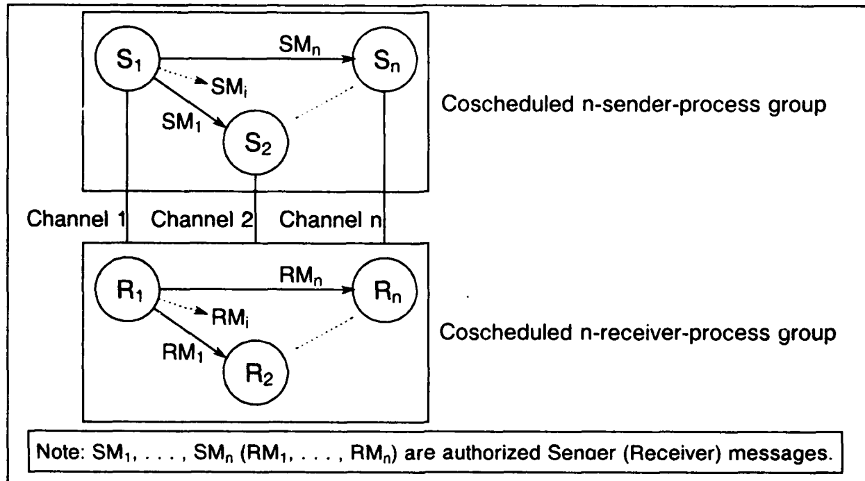
Figure 2-8. Example of n Channels Aggregated in Parallel
