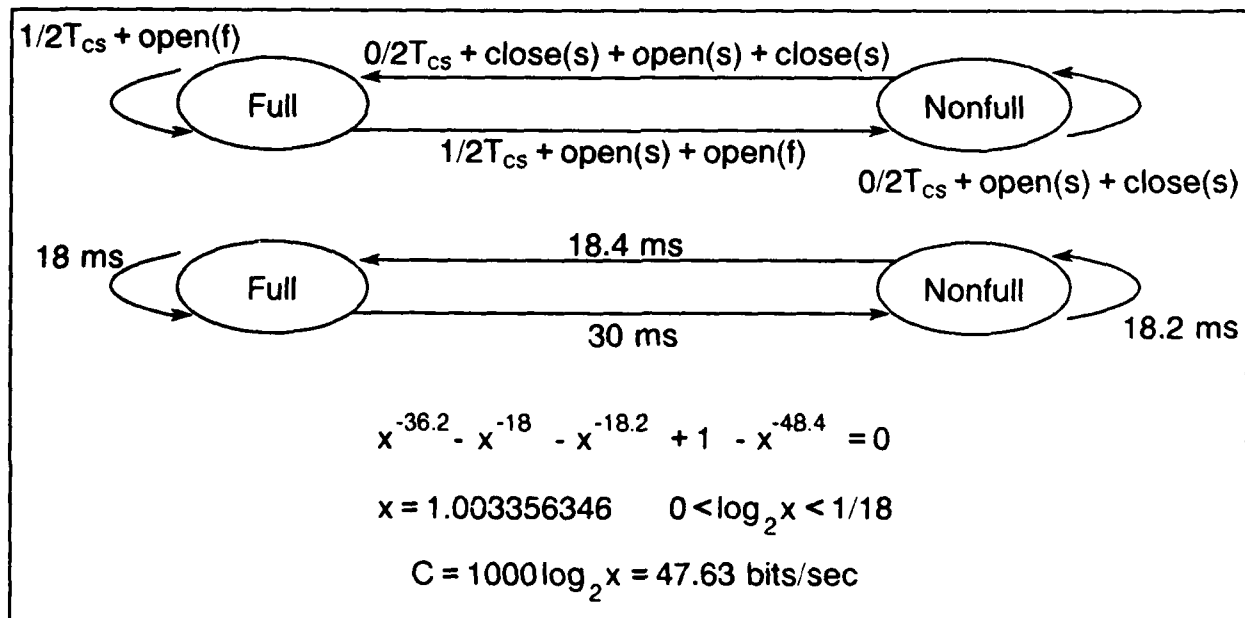
Figure 4-3. State Graphs for the Inode Table Channel
