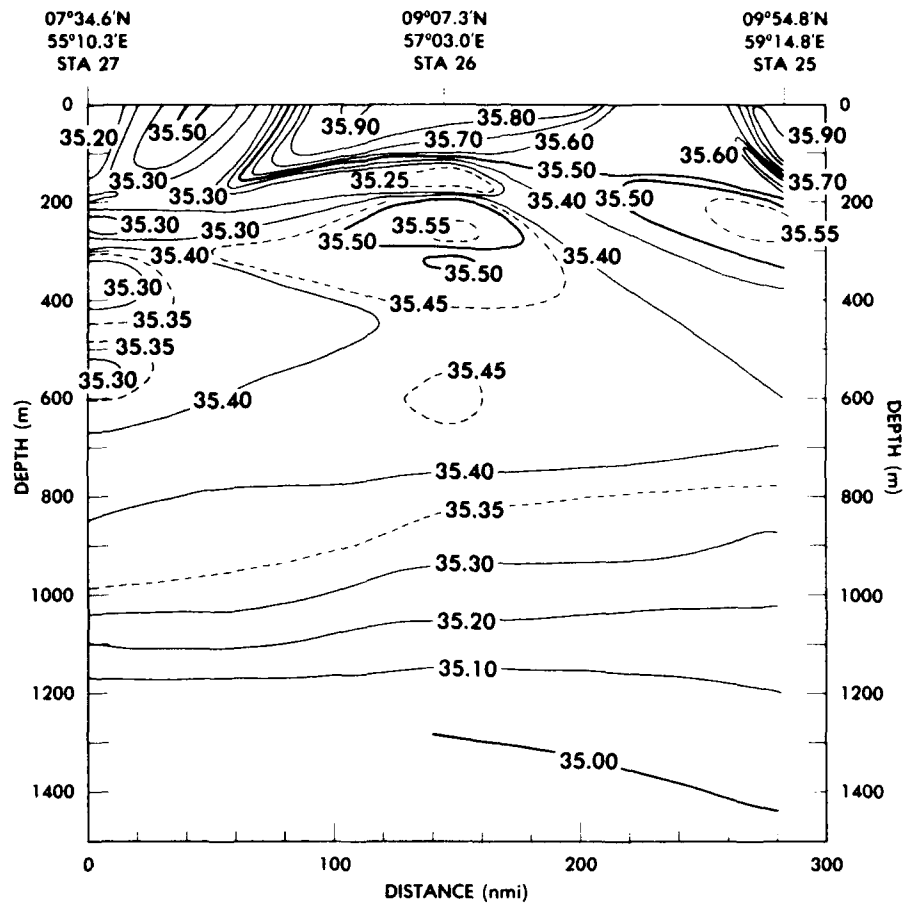
Figure 47. Salinities (‰) along Section 9, USNS WILKES, 31 August - 2 September 1979
