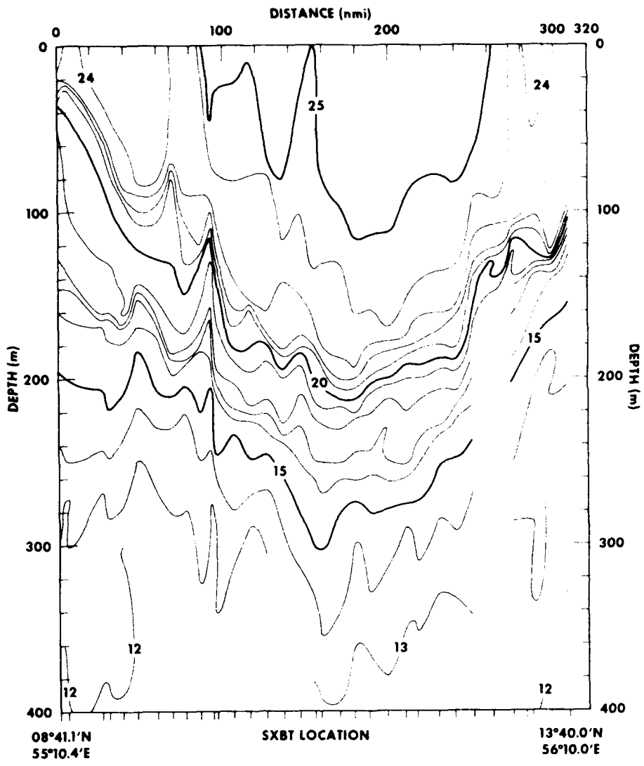
Figure 12. XBT Temperature ( ^{\circ}\text{C} ) Section 7, 28 - 30 August 1979 (see figure 5)
