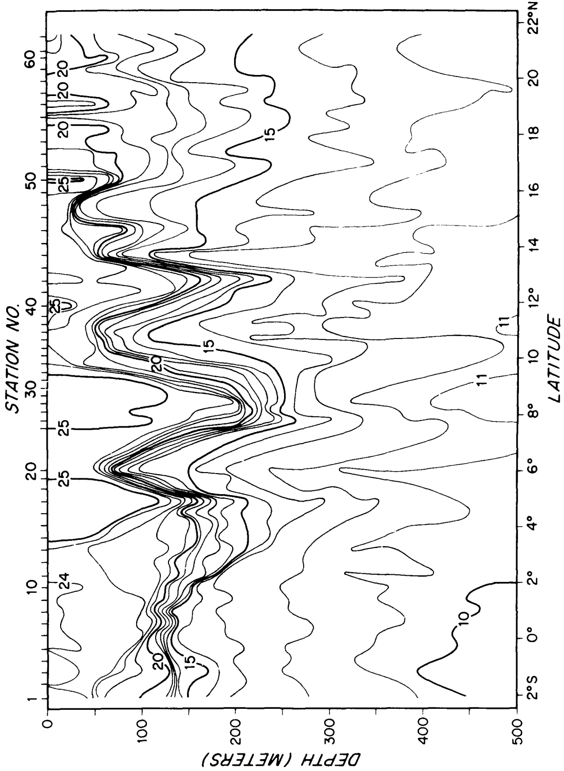
Figure 23. Temperature ( ^{\circ}\text{C} ) from XBT stations along tanker sea lane (see figure 1)
