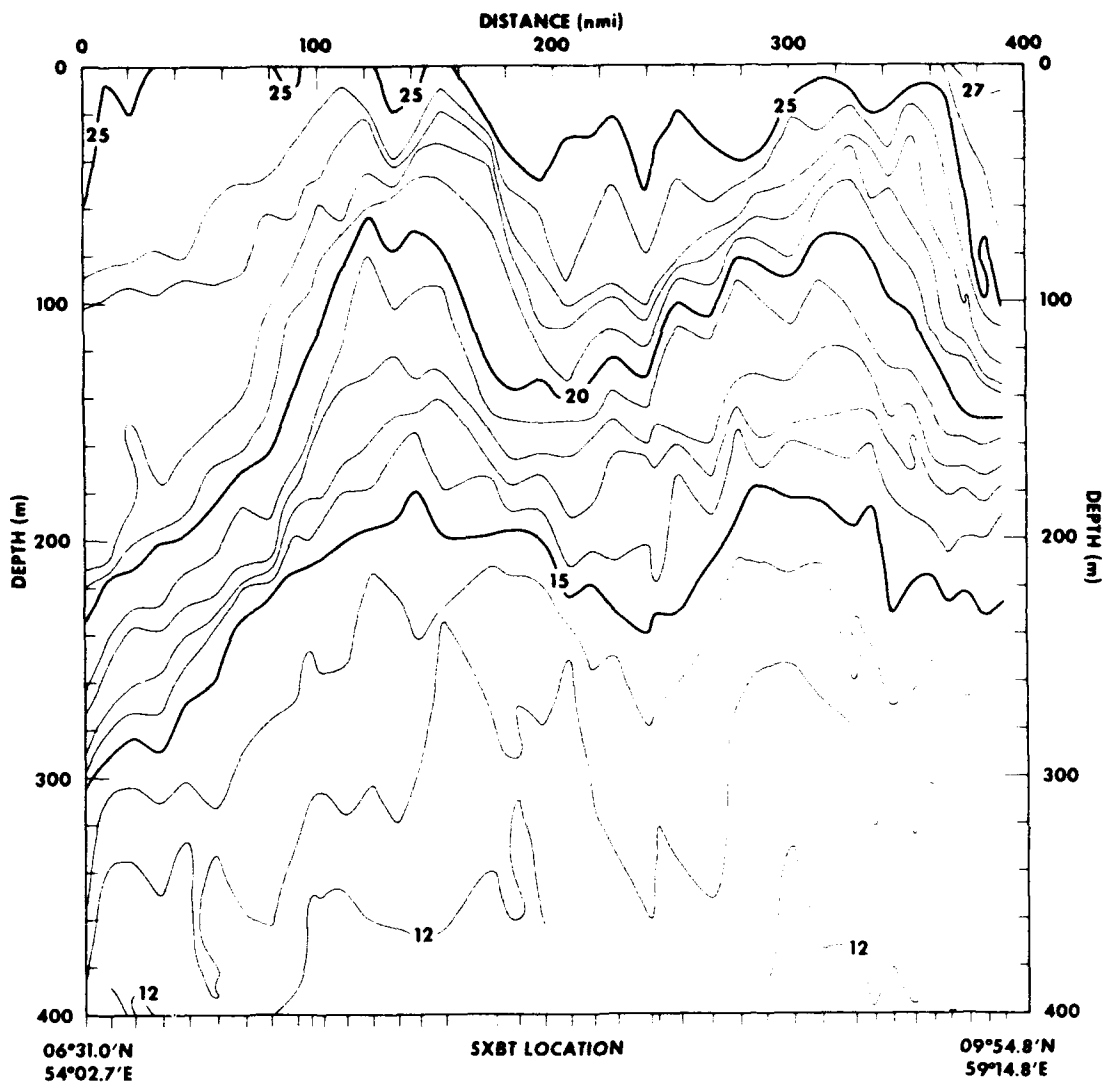
Figure 14. XBT Temperature (°C) Section 9, 31 August - 2 September 1979 (see figure 5)
