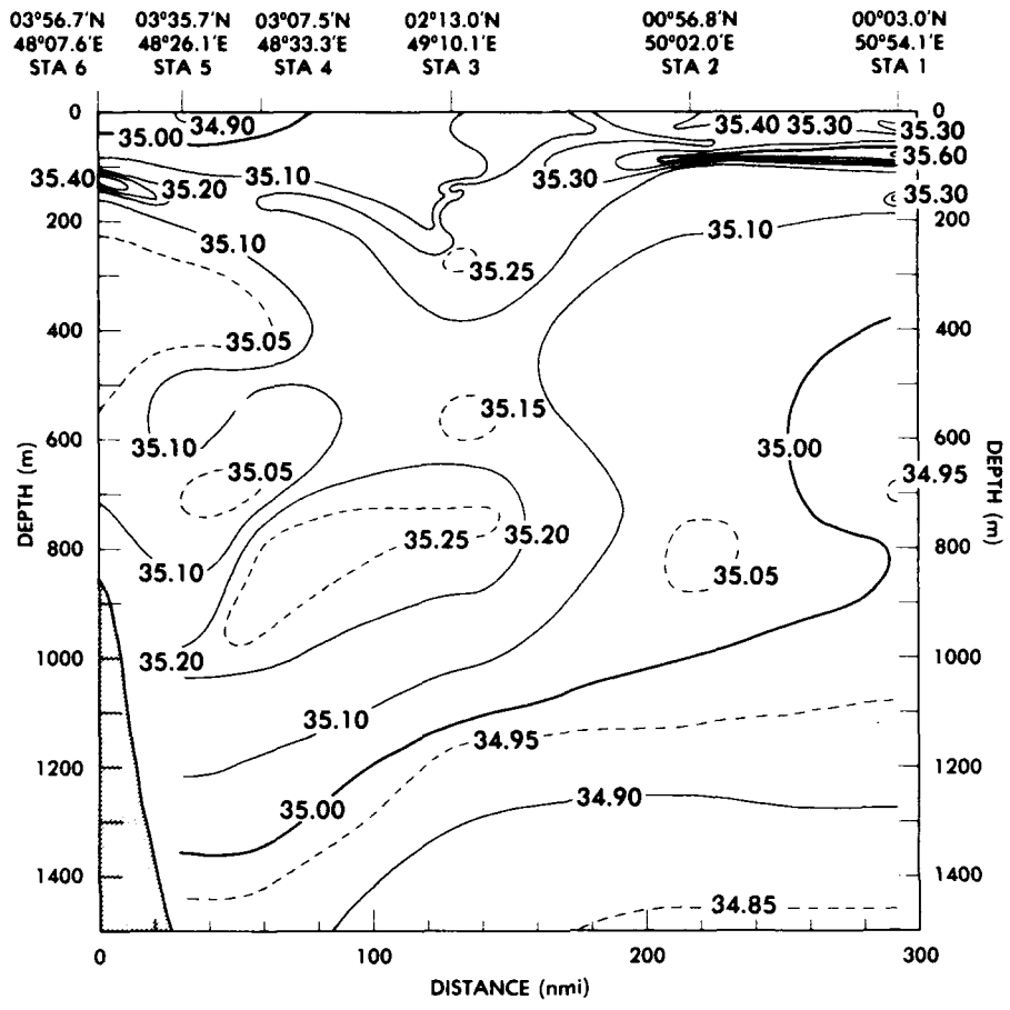
Figure 37. Salinities (‰) along Section 1, USNS WILKES, 16 - 19 August 1979
