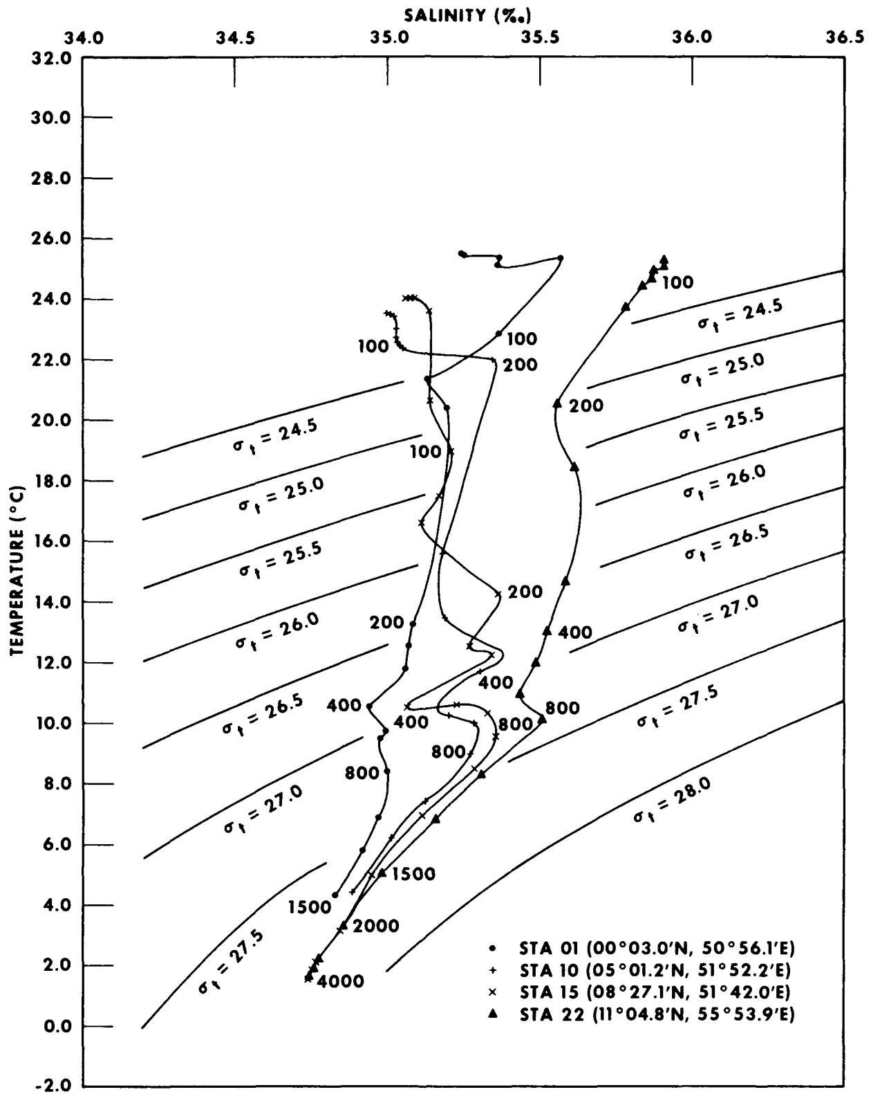
Figure 25. Temperature-Salinity (TS) Curves, Stations 1, 10, 15, 22
