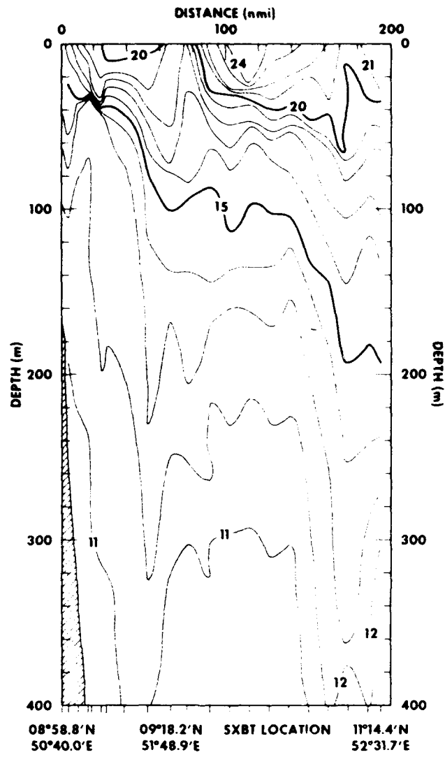
Figure 10. XBT Temperature ( ^{\circ} C) Section 5, 26 - 27 August 1979 (see figure 5)
