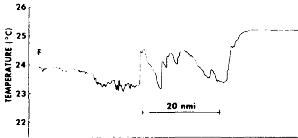
Figure 48a. Continuous sea surface analog temperature ( ^{\circ}\text{C} ) traces made across thermal discontinuities between 18 and 31 August 1979 (see figure 48). Values to the left of thermal discontinuities give temperatures within regions of cool, upwelled water
