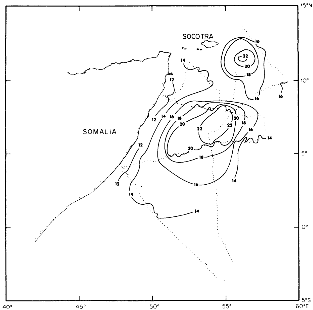
Figure 28. Temperature (°C) at 200m depth, USNS WILKES, 18 August - 3 September 1979
