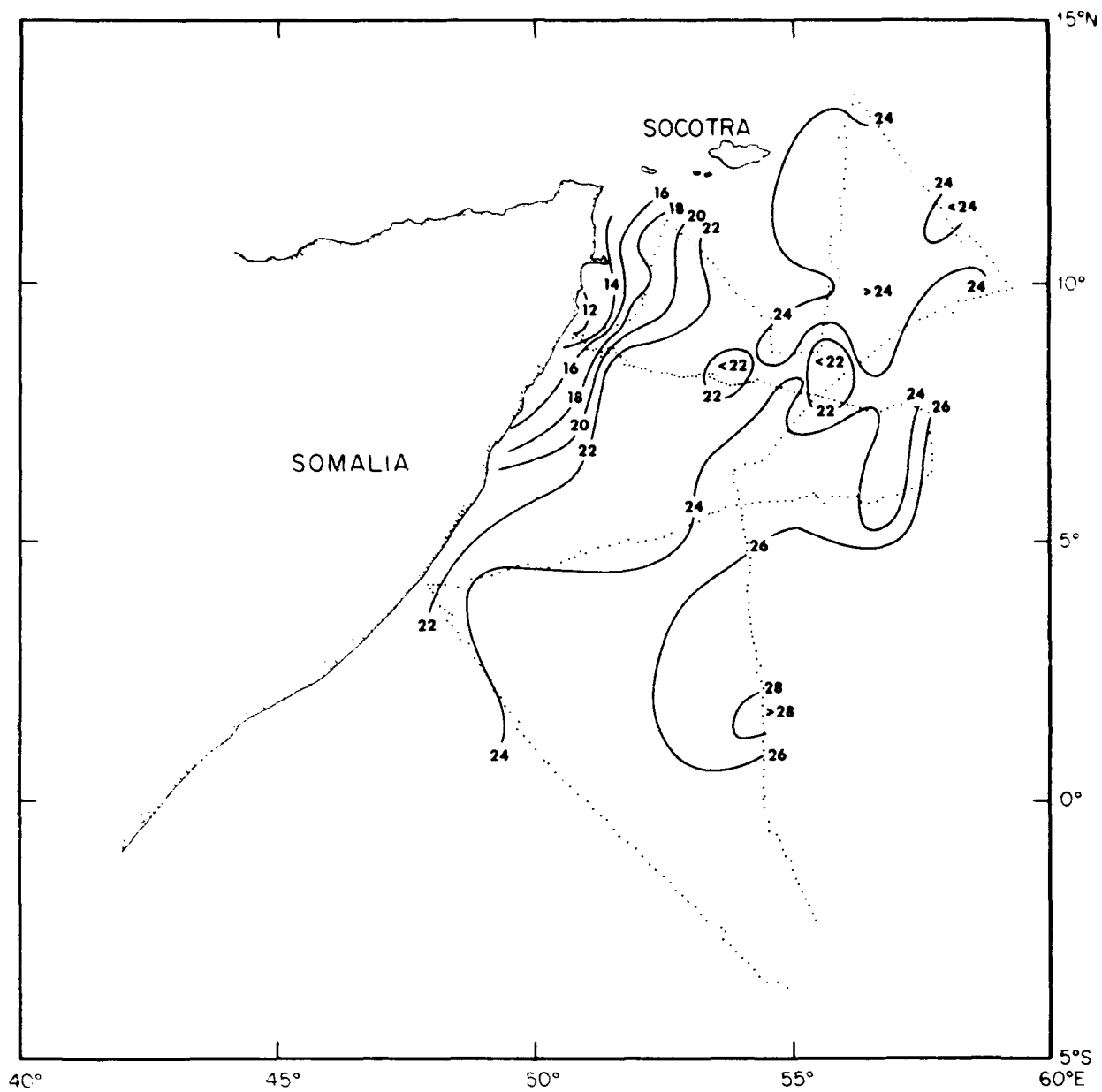
Figure 26. Temperature (°C) at 50m depth, USNS WILKES, 18 August - 3 September 1979
