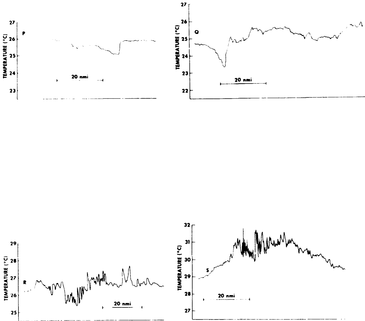
Figure 48c. Continuous sea surface analog temperature (°C) traces made across thermal discontinuities between 31 August and 3 September 1979 (see figure 48). Values to the right in trace P give temperatures in southeastern corner of Socotra Eddy. Values to the right in trace Q give temperatures in northern edge of great whirl. Traces R and S are oriented north-south with values to the left giving temperatures at northern ends of traces
