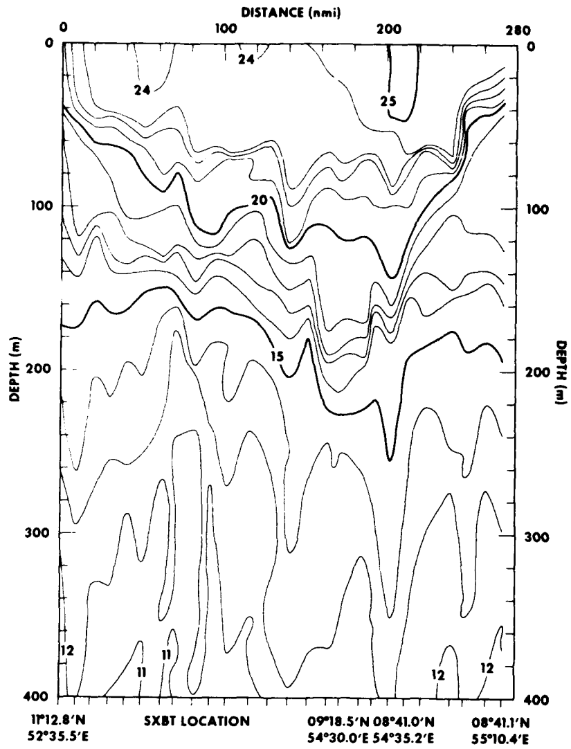
Figure 11. XBT Temperature (°C) Section 6, 27 - 28 August 1979 (see figure 5)
