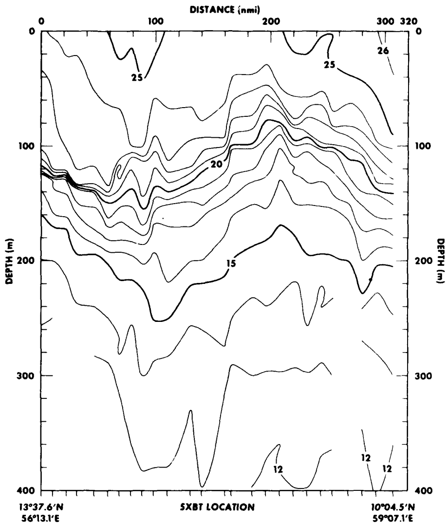
Figure 13. XBT Temperature ( ^{\circ} C) Section 8, 30 - 31 August 1979 (see figure 5)
