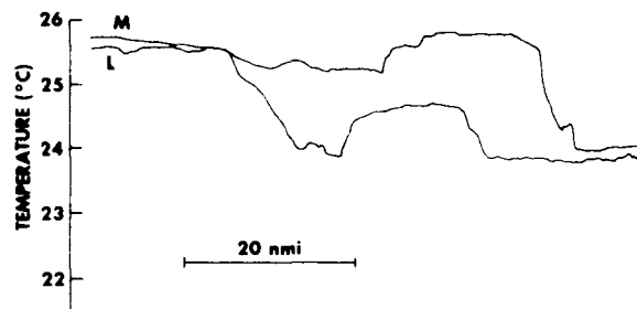
Figure 48b. Continuous sea surface analog temperature ( ^{\circ}\text{C} ) traces made across thermal discontinuities between 26 and 30 August 1979 (see figure 48). Values to the left in traces I, J, and K give temperatures in cool, upwelled water of coastal origin. Values to the left in traces L and M give temperatures in the interior of the Socotra Eddy
