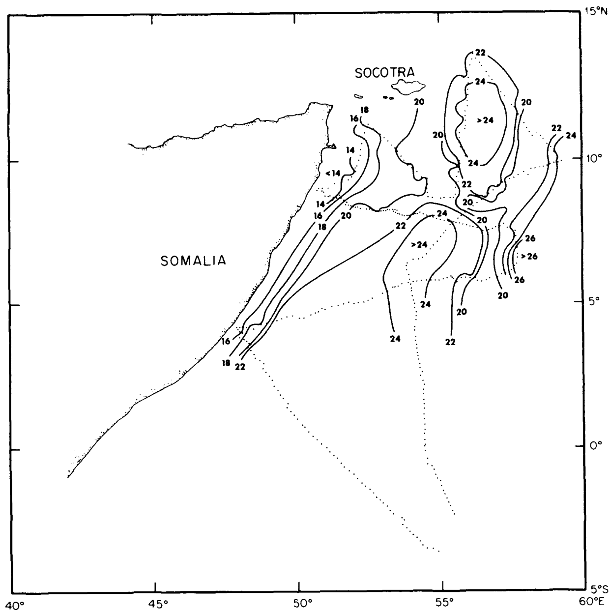
Figure 27. Temperature (°C) at 100m depth, USNS WILKES, 18 August - 3 September 1979
