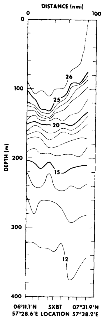
Figure 8. XBT Temperature ( ^{\circ}\text{C} ) Section 3, 22 - 23 August 1979 (see figure 5)
