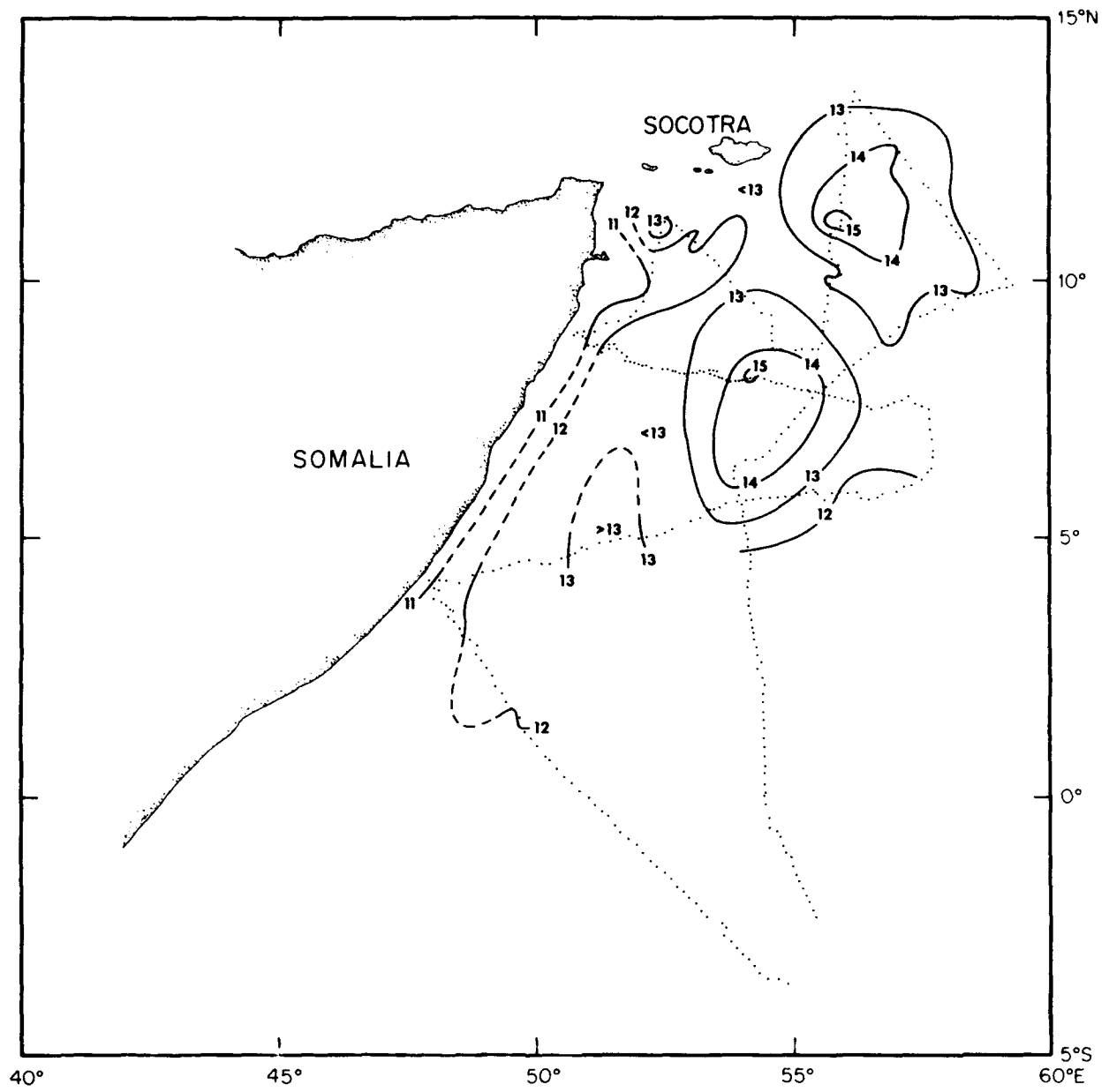
Figure 29. Temperature (°C) at 300m depth, USNS WILKES, 18 August - 3 September 1979
