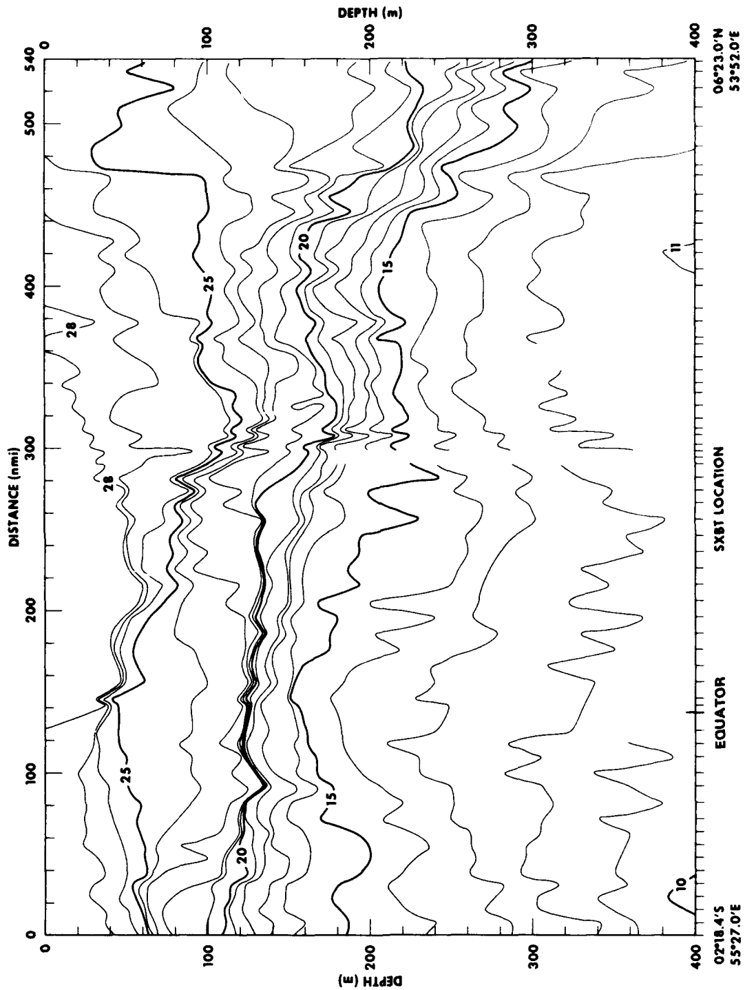
Figure 15. XBT Temperature (°C) Section 10, 2 - 4 September 1979 (see figure 5)
