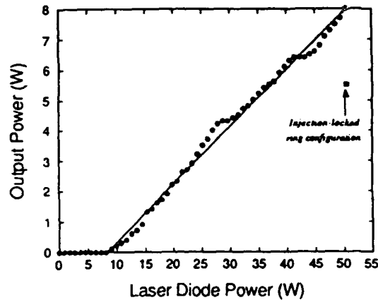
Figure 5. Input-output power curve for the standing wave laser vs input diode laser power. Each dot represents the addition of a single diode laser. The threshold pump power is 8.3W. The maximum output power is 8.0W in a TEM 00 mode. The slope efficiency is 19%. The single point is the 5.5W output power for a ring cavity oscillator that is injection locked.
