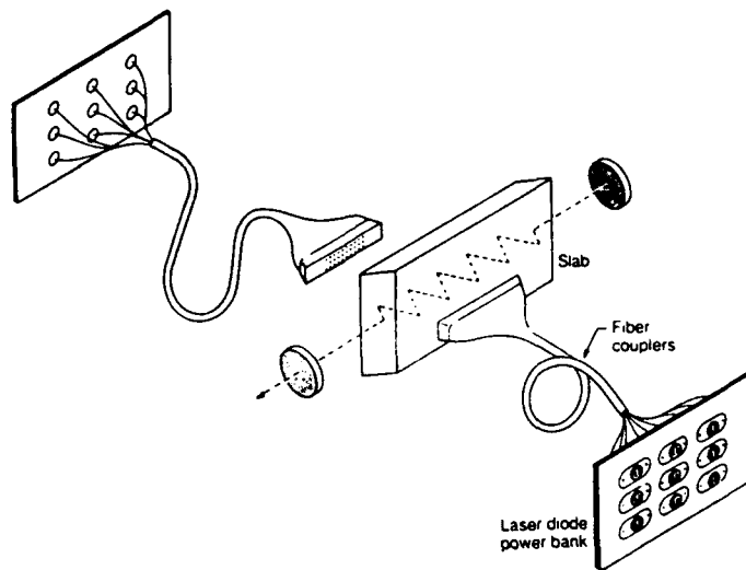
Figure 1. Schematic of the proposed high average power solid state laser pumped by diode lasers coupled via optical fibers. This design offers that advantages of power scaling, separation of the thermal problems of the diode cooling and the slab cooling, possibility of repair during operation, and the opportunity to upgrade diode lasers without forcing a redesign of the slab laser head.
