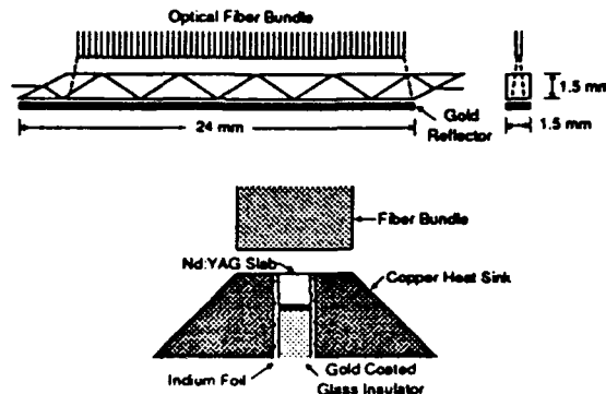
Figure 3. Schematic of the conduction-cooled, fiber-coupled, laser-diode-pumped, cw Nd:YAG minislab laser head. Pumping is orthogonal to the conduction cooled faces. The laser is pumped by 56, 1Watt laser diodes coupled to 300 \mu m core diameter fibers. A gold coated mirror reflects the pump radiation back through the 1.5mm thick Nd:YAG slab for efficient pumping.
