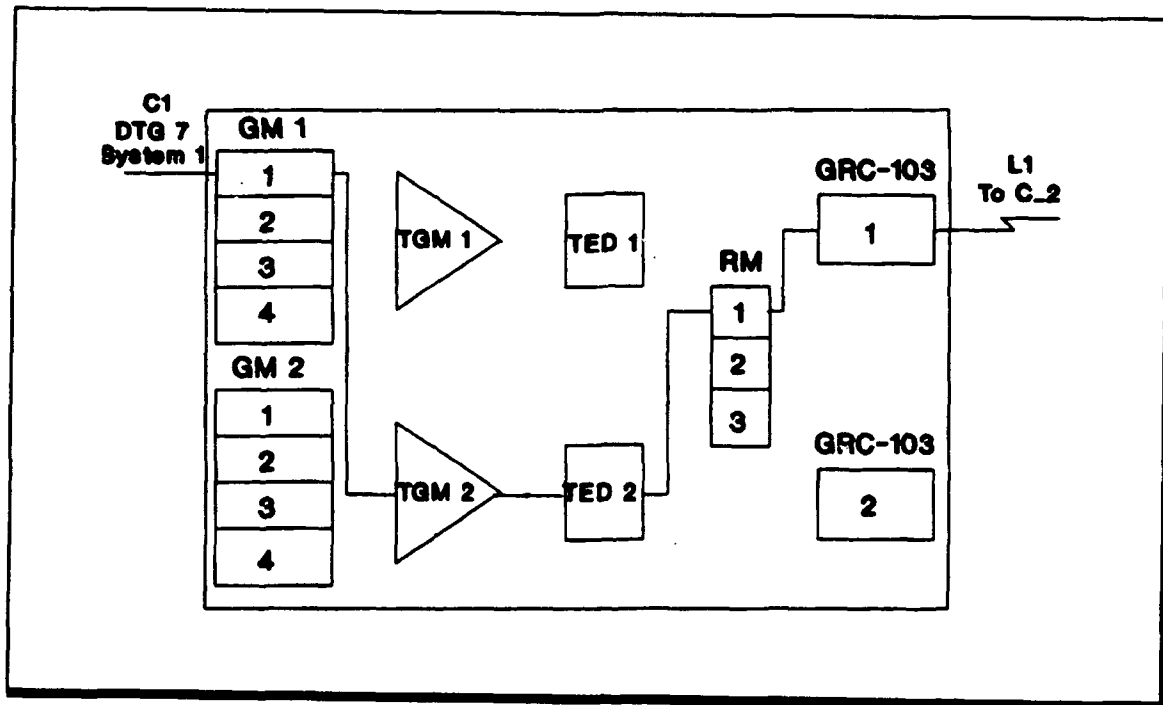
Figure 28: Node 2 C_1 Internal Connectivity
