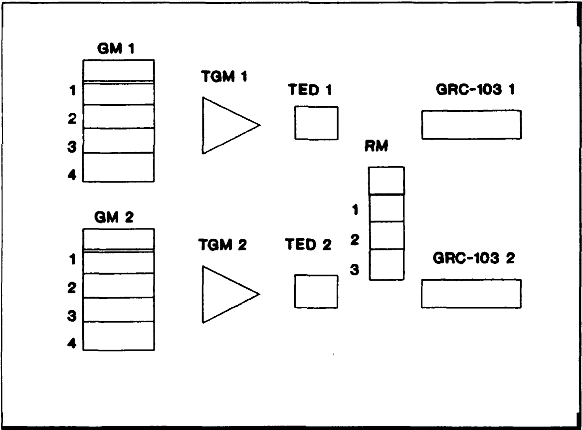
Figure 11: TRC-173 Component Level
