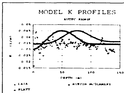
Figure 4. AUTEK range field results. Note scatter in k data.
