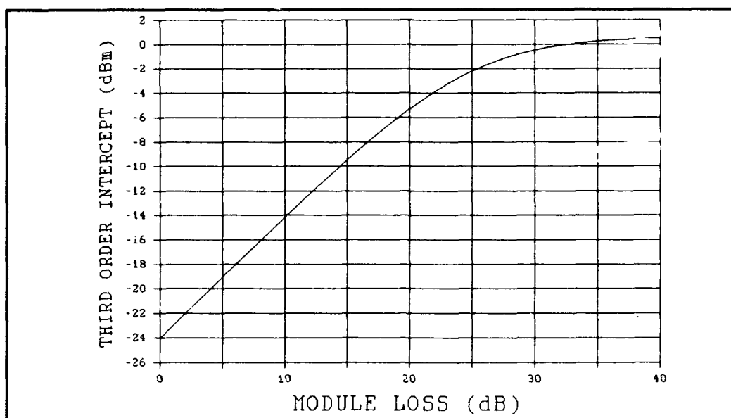
Figure C-5B. Case 5, MESFET 3-Stage Third-Order Intercept, Reference Page 31.
