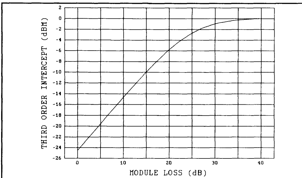
Figure C-4E. Hoffman's C-1 Results, Case 4, MESFET 3-Stage Third Order Intercept, Reference Page 30, Shown For Comparison.
