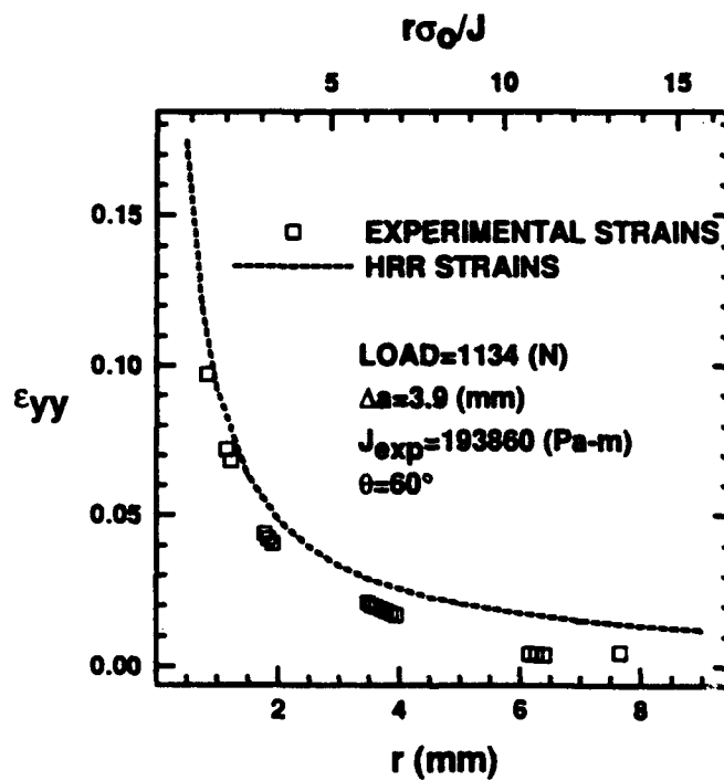
Figure 15b. Crack tip \epsilon_{yy} of 2024-T3 SEN specimen with moderate stable crack growth. Coarse grating analysis
