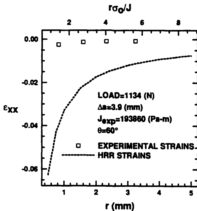
Figure 15a. Crack tip \epsilon_{xx} of 2024-T3 SEN specimen with moderate stable crack growth. Coarse grating analysis
