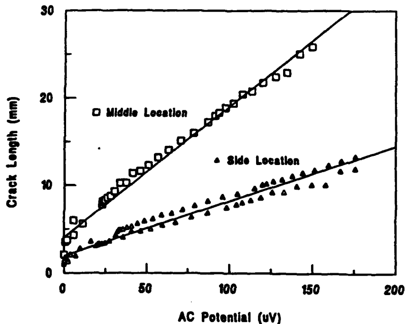
FIGURE 7. EFFECT OF POTENTIAL LEAD PLACEMENT ON CRACK LENGTH SENSITIVITY
