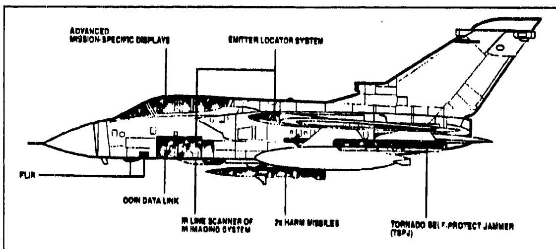
Figure 6-1. Tornado Aircraft Equipped for SEAD
