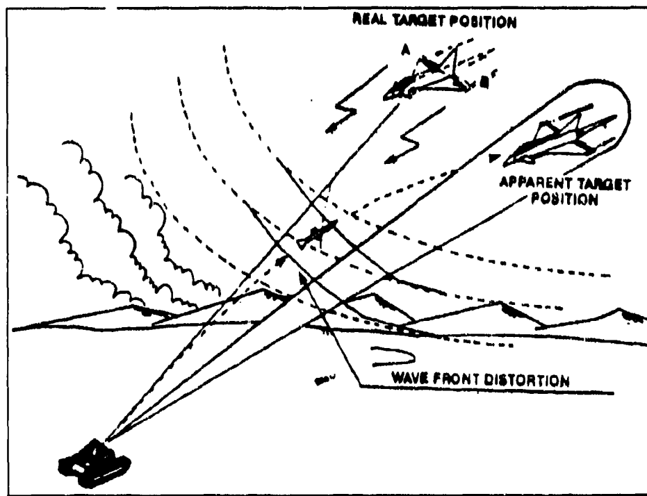
Figure 4-1. Cross-Eye Deception
