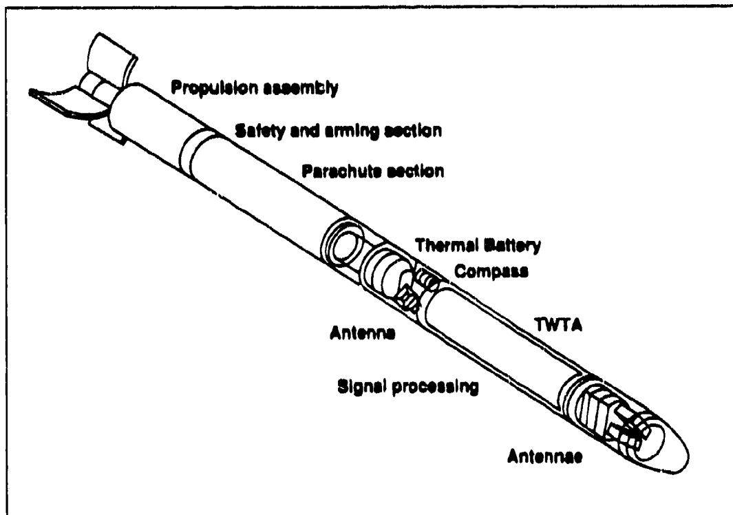
Figure 4-15. Carmen Decoy
