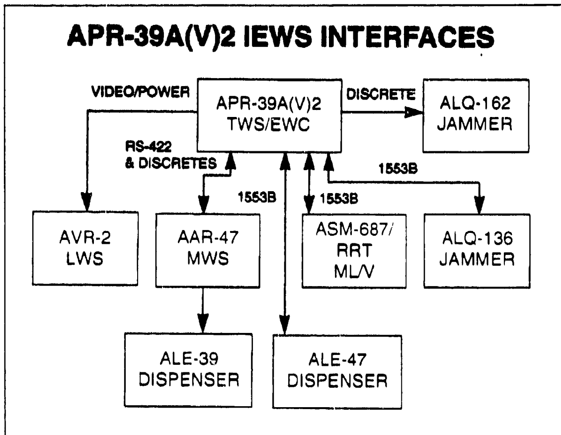
Figure 5-4. Blockdiagram over APR-39A(V)2 as Integrated EW system
