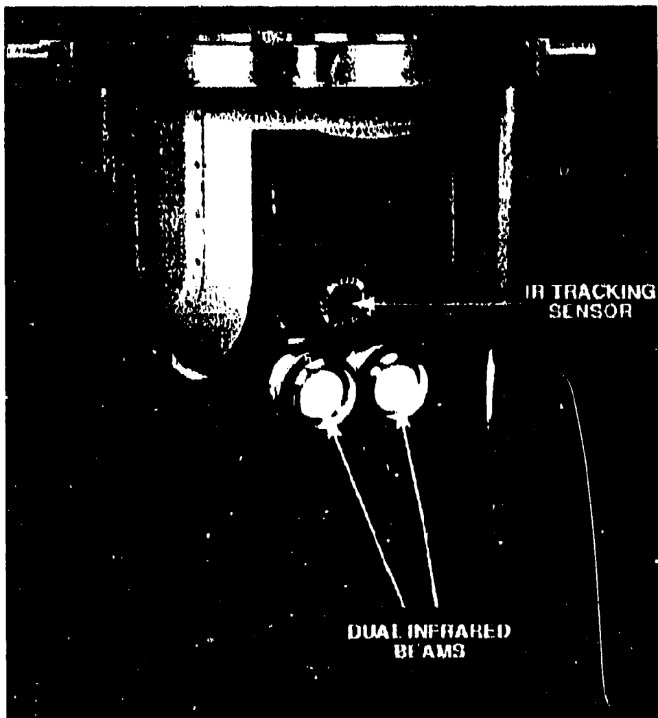
Figure 4-8. DIRCM
