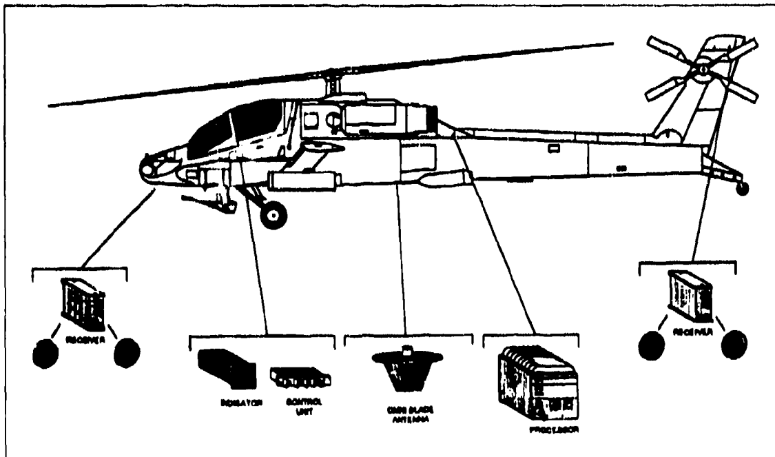
Figure 3-10. AN/APR-39A(V)3
