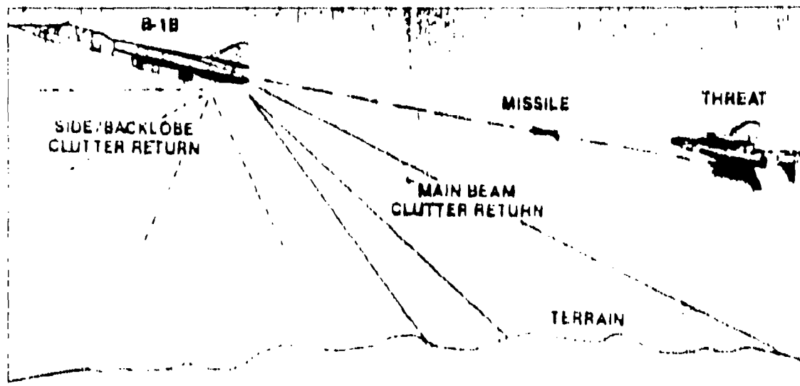
Figure 3-15 Clutter Return for Active MWS
