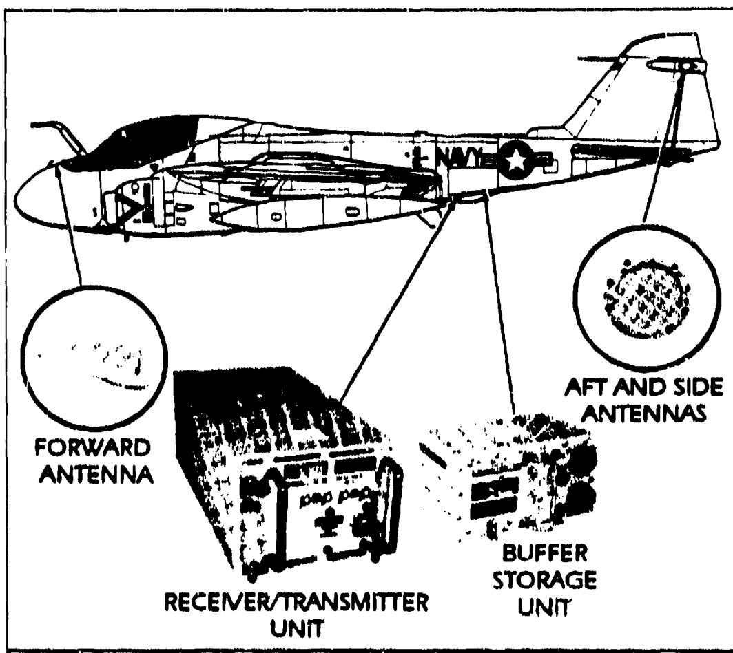
Figure 3-17. AN/ALQ-156(A) Missile Warning System
