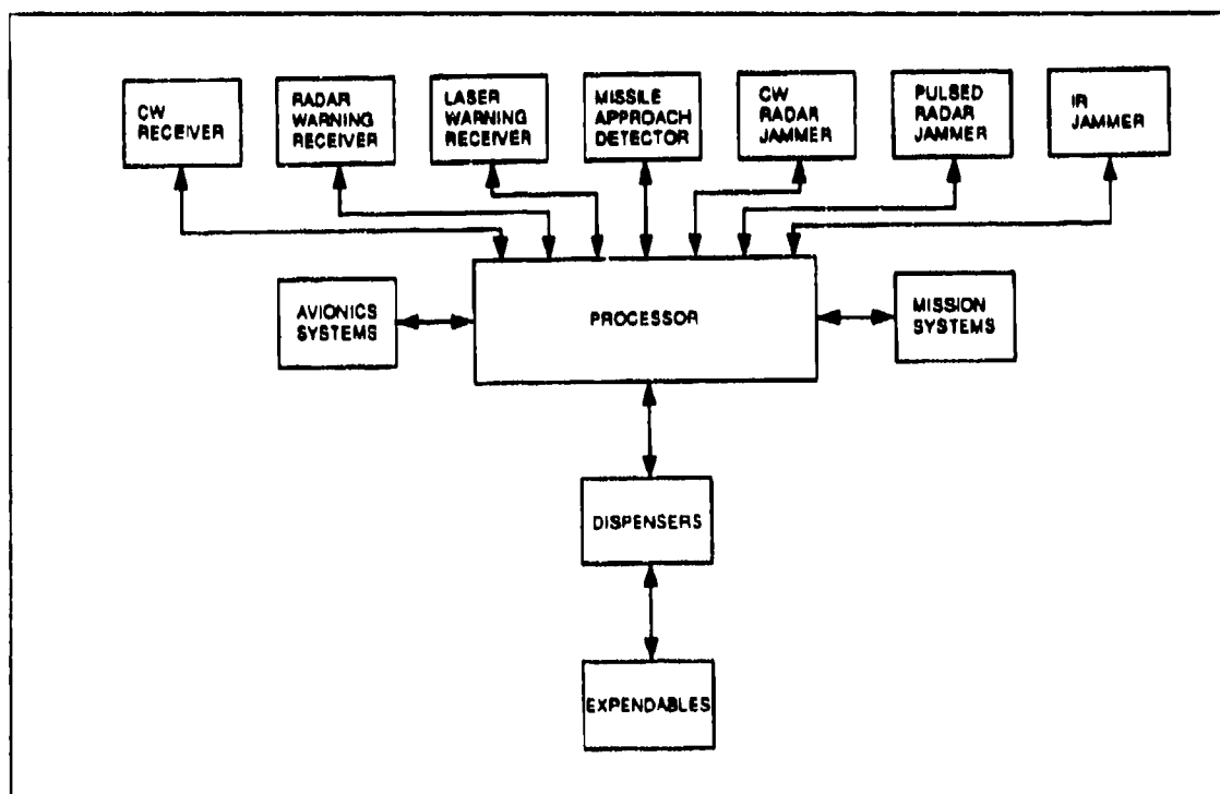
Figure 5-3. Prinicpal Diagram over INEWS
