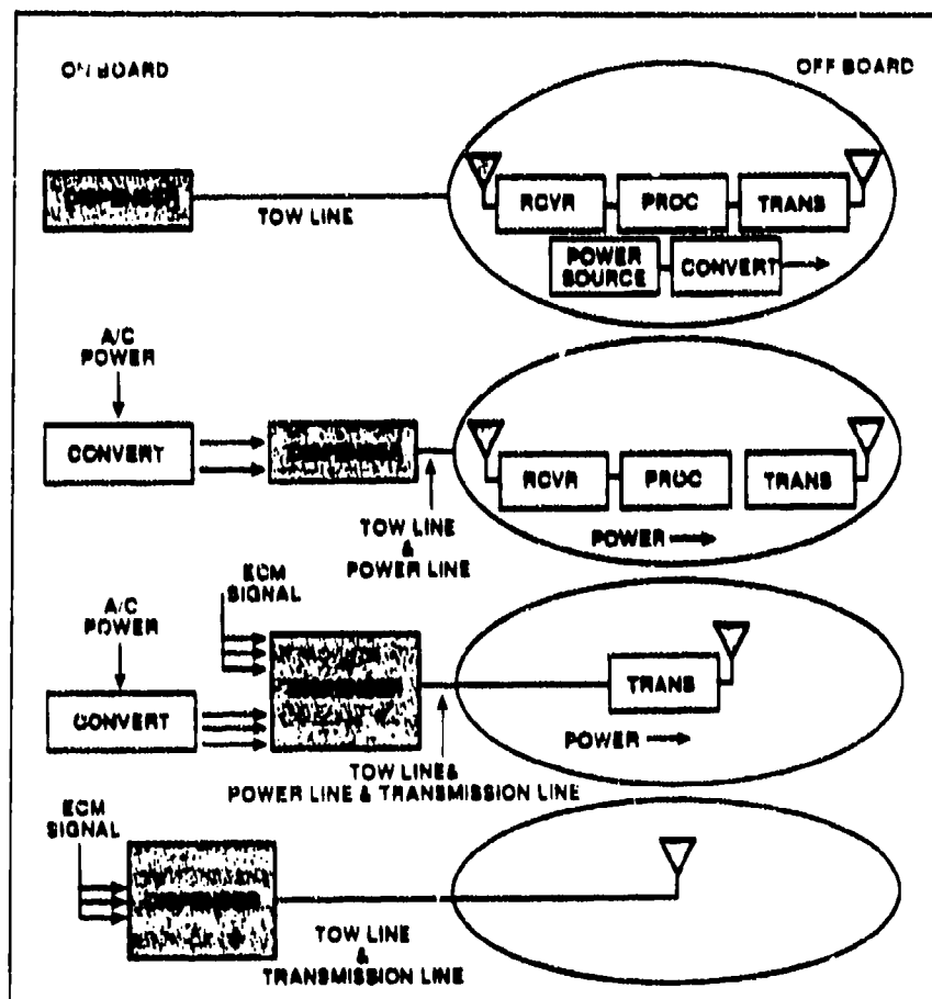
Figure 4-18 Different Possible Configurations for Airborne Decoys
