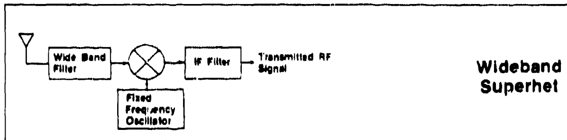
Figure 3-2. Superhetrodyne Receiver
