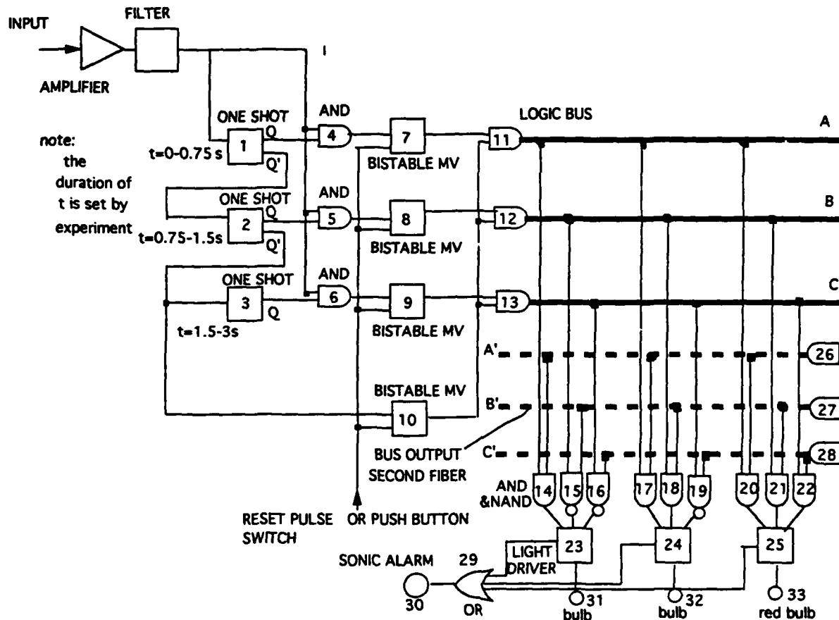
Figure 3-1. Logic diagram.
