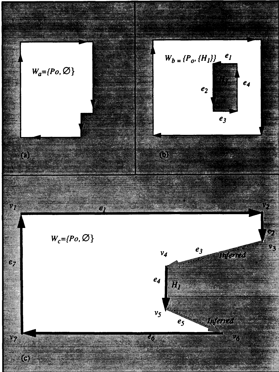
Figure 6.5 - Example Worlds
