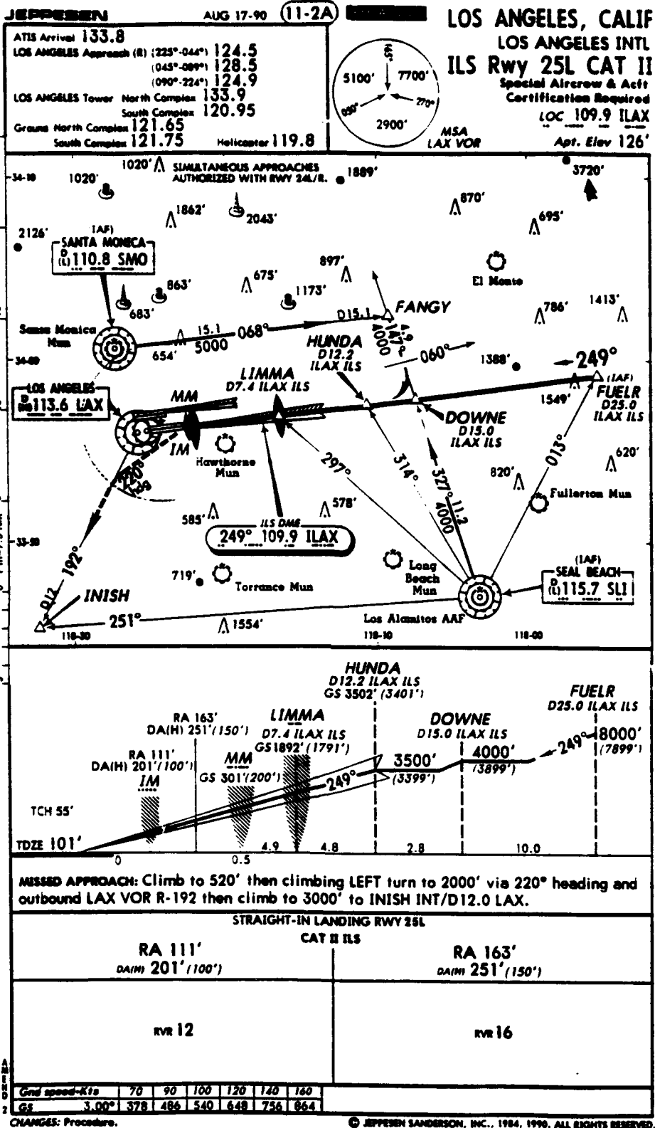
FIGURE 6. ILS APPROACH RUNWAY 25L, CAT II
