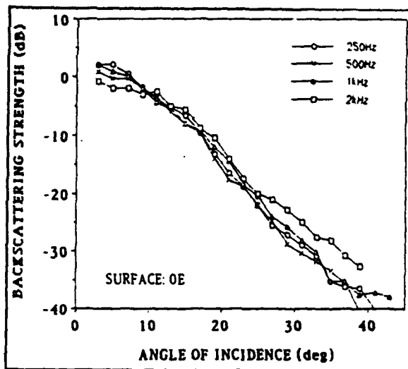
Figure 4: Frequency dependence of scattering from surface 0E.
