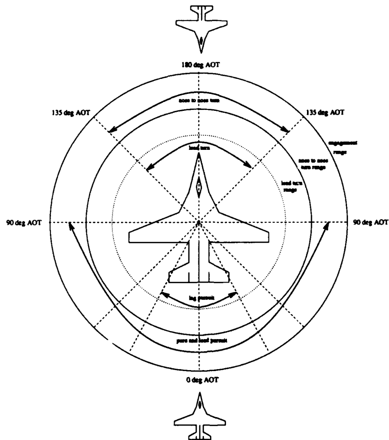
Figure 4.4 Simple maneuvers.
