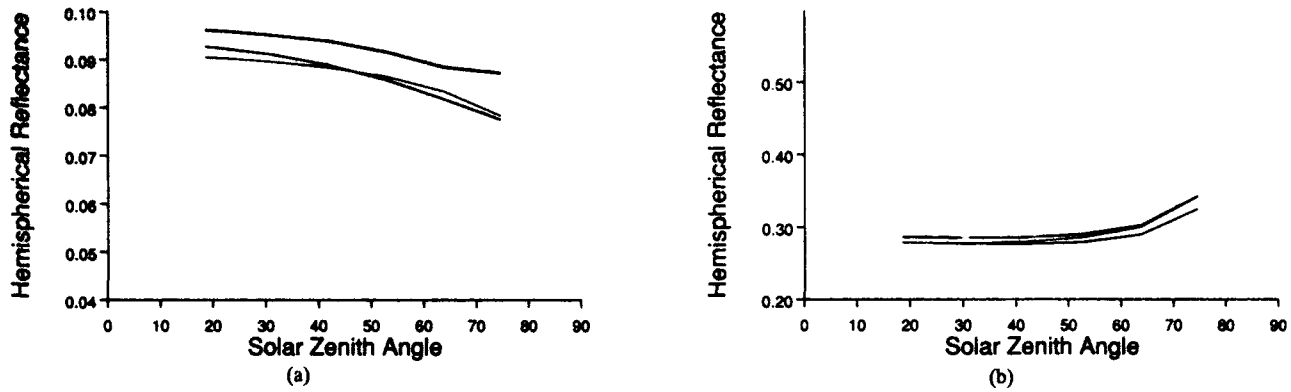
Fig. 5. Spectral hemispherical reflectances from the Liang-Strahler coupled radiative transfer model using a planophile canopy (LAI = .5) with a Rayleigh atmosphere (—), an optical depth of .1 for (a) \lambda = .65 \mu\text{m} and .07 for (b) \lambda = .8 \mu\text{m} (---), and the inclusion of a 1.2 specular index (—○—).
