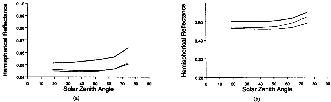
Fig. 6. Spectral hemispherical reflectances from the Liang-Strahler coupled radiative transfer model using a planophile canopy (LAI = 3) with a Rayleigh atmosphere (—), an optical depth of .1 for (a) \lambda = .65 \mu\text{m} and .07 for (b) \lambda = .8 \mu\text{m} (---), and the inclusion of a 1.2 specular index (—○—).
