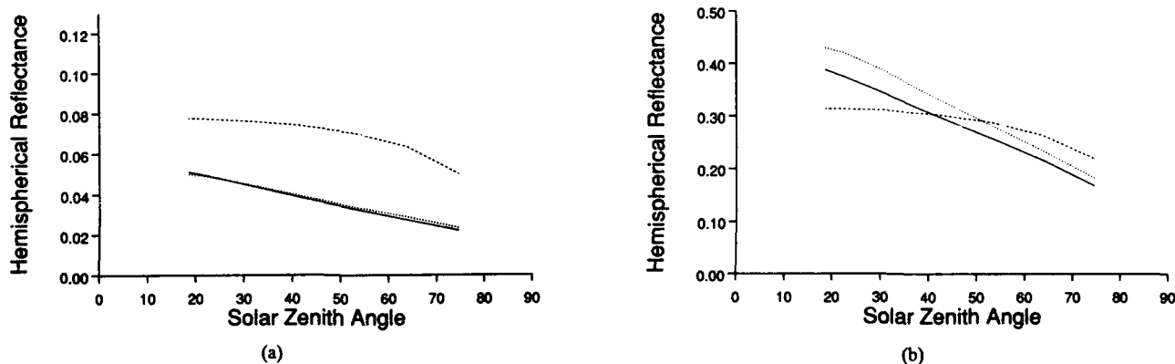
Fig. 3. The instantaneous hemispherical reflectance from the geometric-optical model for a 60% conifer (—) covered scene, a 40% savanna (---) covered scene, and a 80% shrub (· · ·) covered scene in the red (a) and near-infrared (b) wavelengths.
