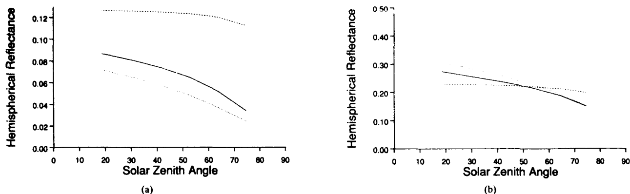
Fig. 4. The instantaneous hemispherical reflectance from the geometric-optical model for a 20% conifer (—) covered scene, a 10% savanna (- - -) covered scene, and a 30% shrub (· · ·) covered scene in the red (a) and near-infrared (b) wavelengths.
