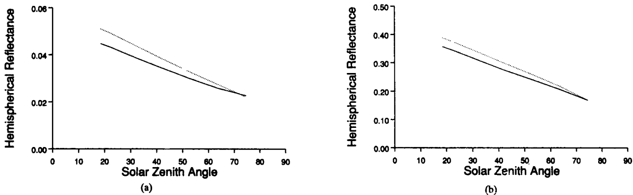
Fig. 7. Instantaneous 60% conifer covered canopy hemispherical reflectances (—) from the geometric-optical model calculated by using the dense homogeneous hemispherical reflectances from the Liang-Strahler coupled radiative transfer model as sunlit canopy component signatures (a) \lambda = .65 \mu\text{m} , (b) \lambda = .8 \mu\text{m} . The geometric-optical model hemispherical reflectances calculated with a constant sunlit canopy component signatures are provided again for comparison (···).
