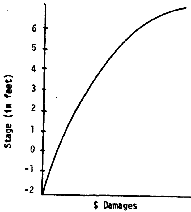
(a) Land Use Composite Stage-Damage Function
