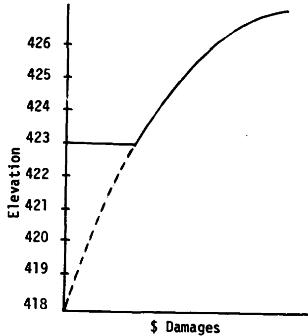
(d) Truncated Elevation-Damage Function for Grid Cell
