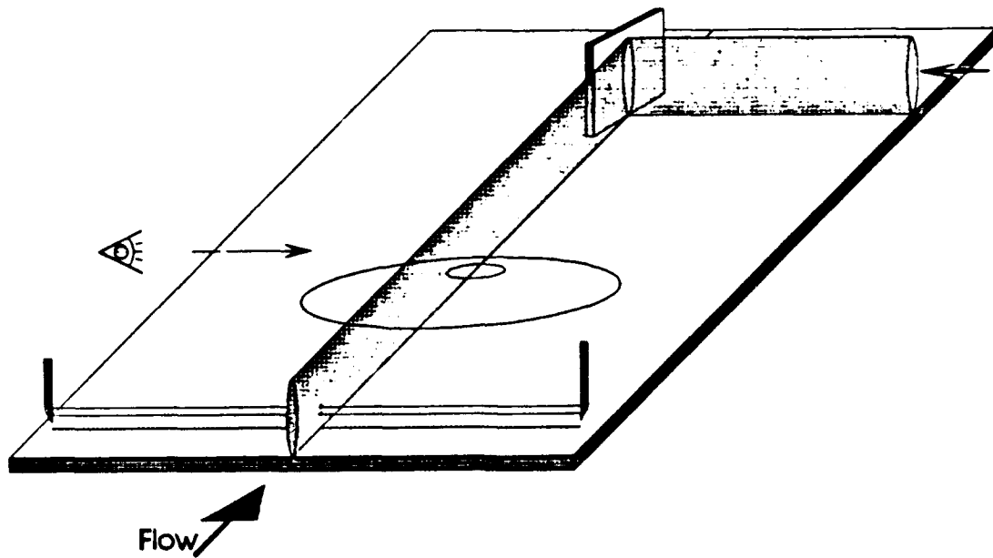
Figure 8a. Schematic of Laser-Light Sheets Arrangement for X-Type Visualization Set Up.
