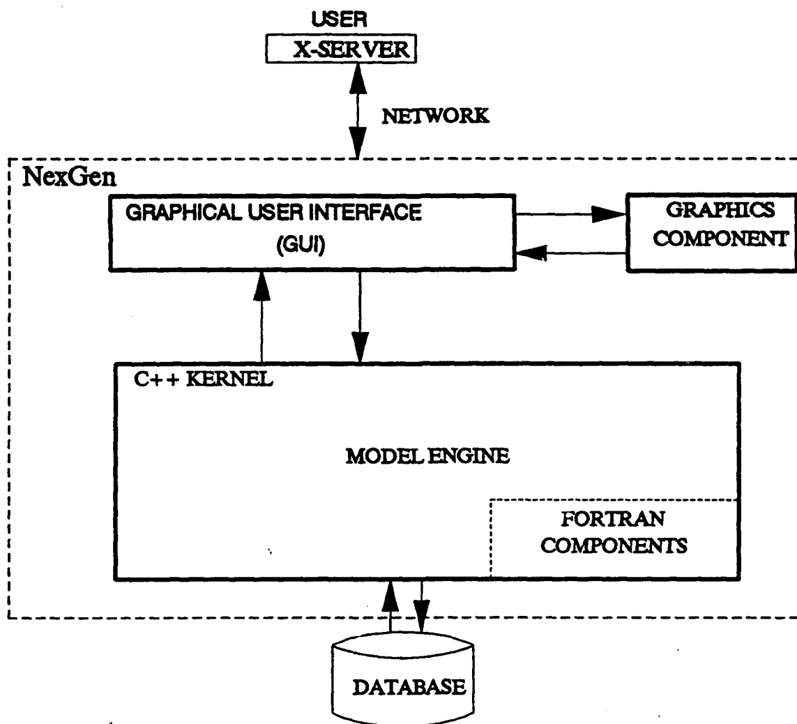
Figure 1. Recommended NexGen Software Architecture
