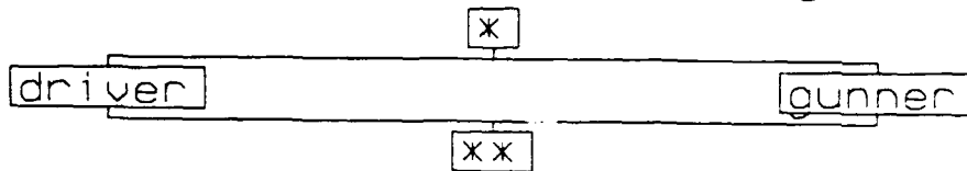
Figure A-15. Fault tree for loss of driver and gunner.
