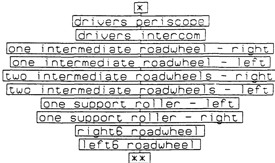
Figure A-1. Fault tree for reduced speed, slight.
