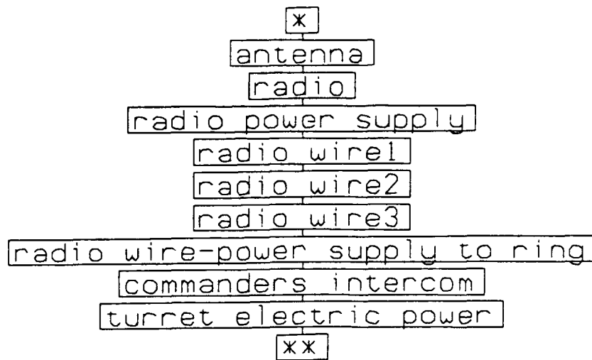
Figure A-19. Fault tree for no external comms beyond 300 ft.
