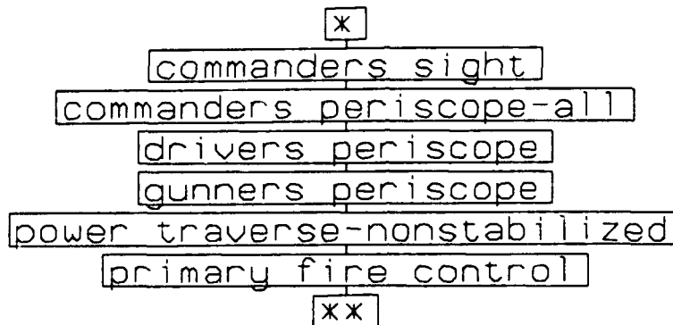
Figure A-9. Fault tree for reduced acquisition capability.
