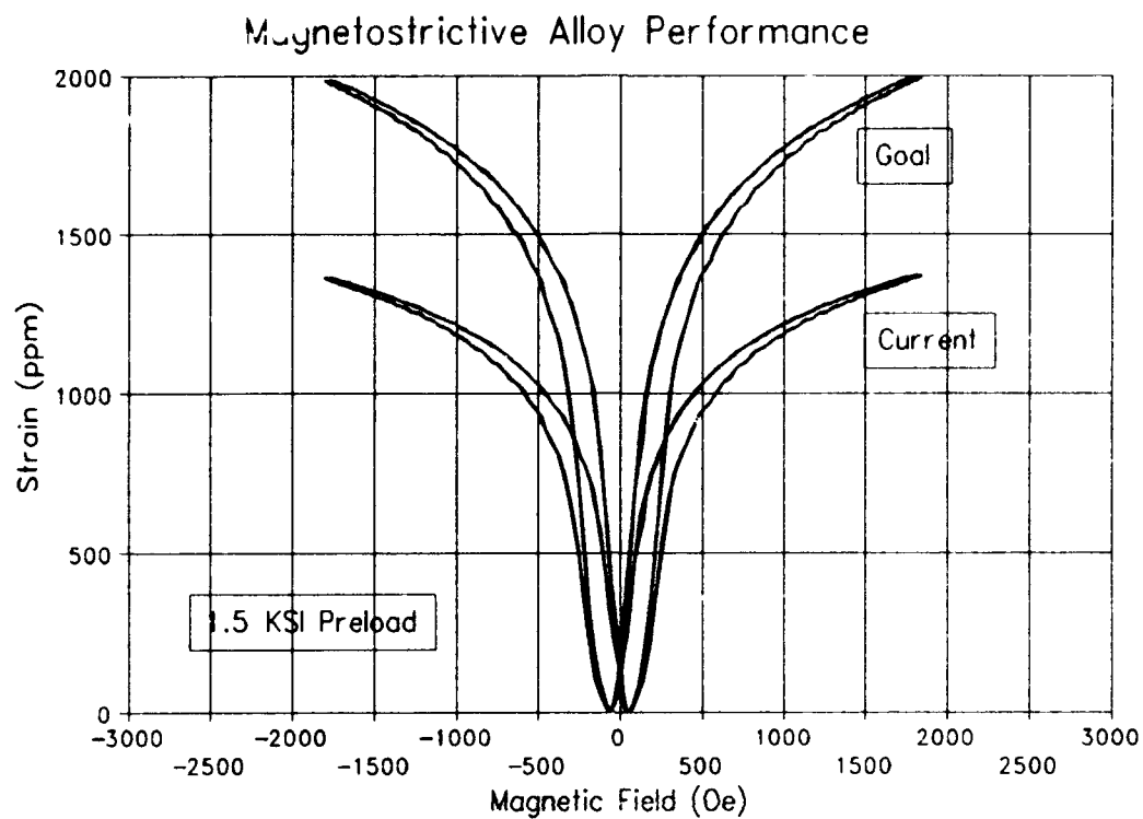
Figure 3. Performance of magnetostrictive TERFENOL-D transducer elements (current twinned \langle 112 \rangle oriented crystals compared to research goals of defect-free \langle 111 \rangle crystallographic oriented drive elements).
