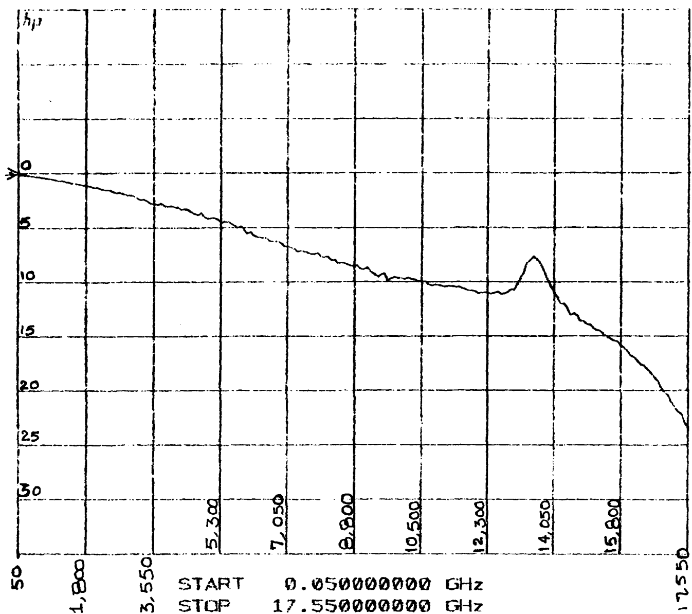
Figure 7. Attenuation measurement of a paint. 10 gms of 10% Hypalon, 3 gms of iron powder, 3 gms of nickel powder and 3 gms of nickel zinc ferrite.
