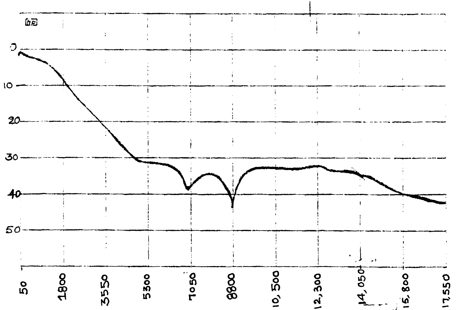
Figure 3. Attenuation measurements of Eccosorb 269 E manufactured by Emerson & Cuming.
