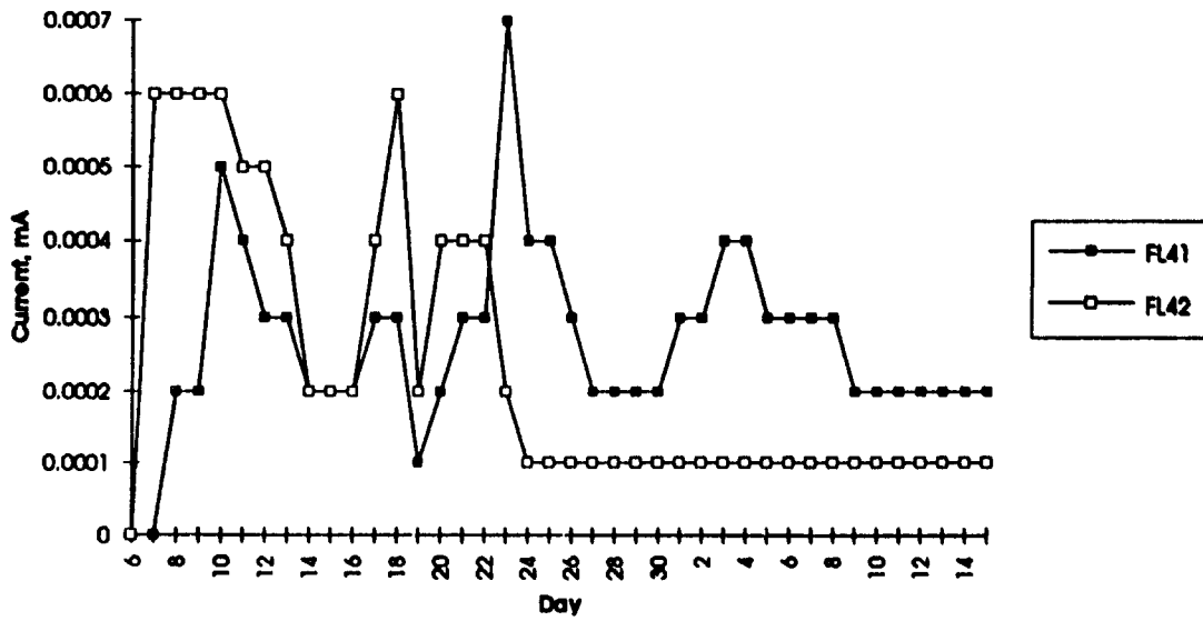
Figure 10. Time-to-Corrosion (Florida Class 4)
