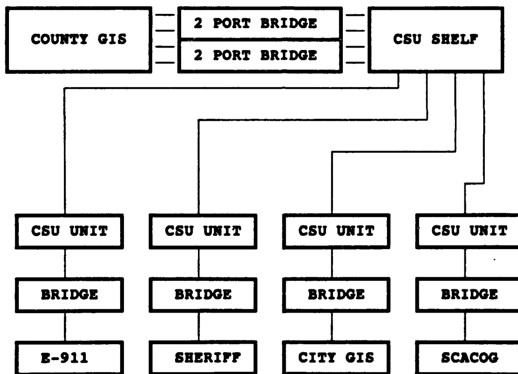
Figure 2: T-1 Schematic
