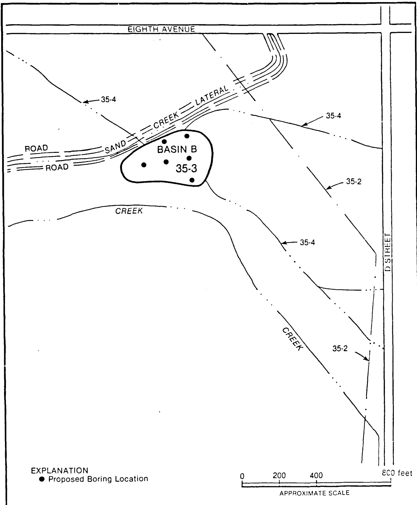
Figure 3.3-11 BORING LOCATION MAP SITE 35-3 RMA, SECTION 35 SOURCE: HARDING LAWSON ASSOCIATES
