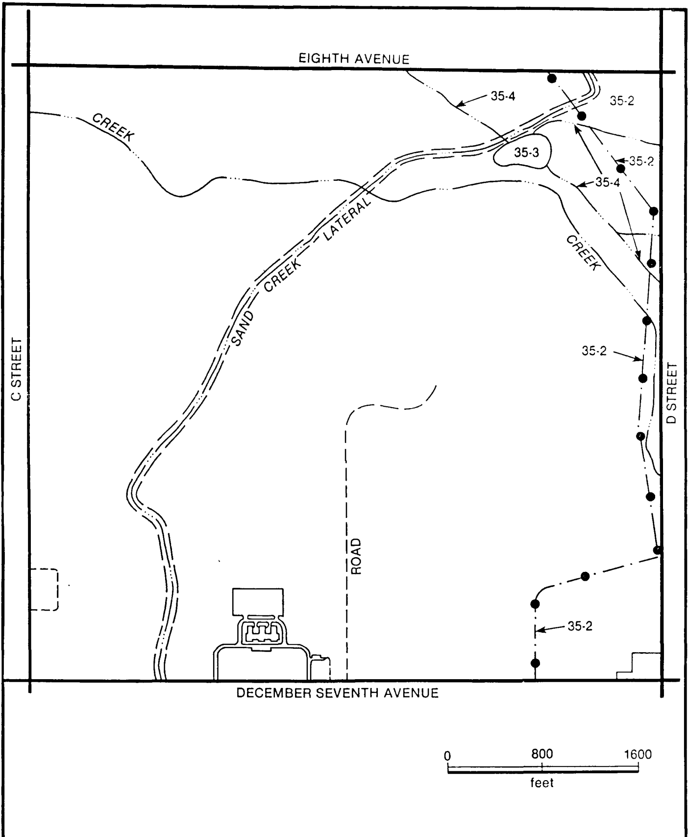
Figure 3.3-10 BORING LOCATION MAP SITE 35-2 RMA, SECTION 35 SOURCE: HARDING LAWSON ASSOCIATES
