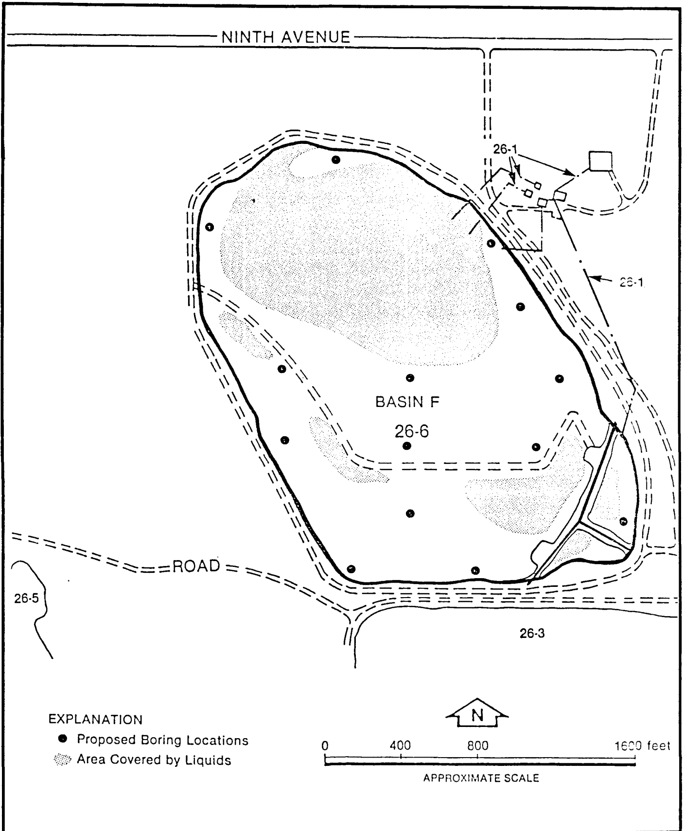
Figure 3.3-6 BORING LOCATION MAP SITE 26-6 RMA, SECTION 26
