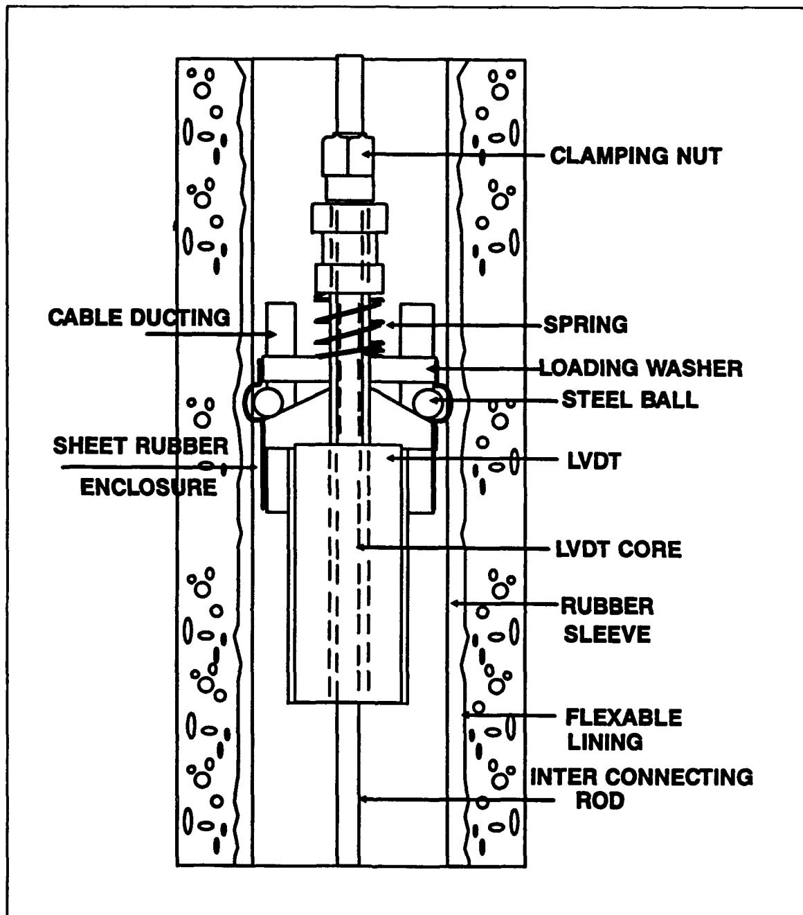
Figure 8. Components of an MDD module
