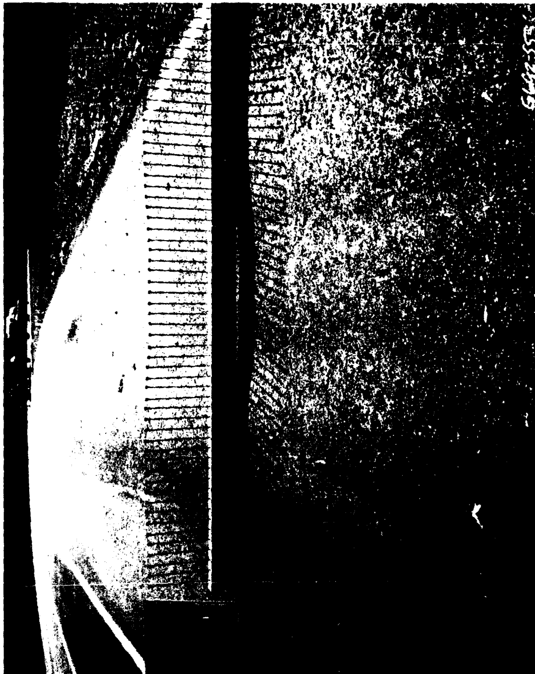
Photo 16. Item 5, high-tire pressure lane, maximum 1-in. rutting after 323 passes
