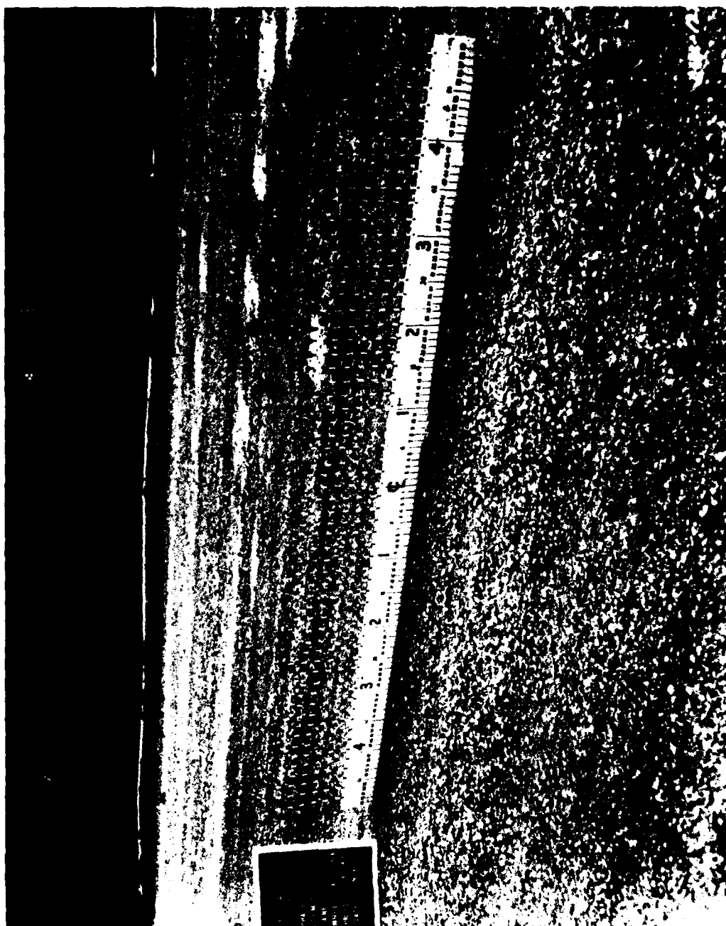
Photo 66. Item 14, low-pressure tire lane, typical low-severity washboarding after 491 passes during the induced failure plan
